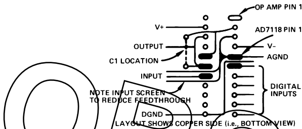
Figure 4. Suggested Layout for AD7118 and Op Amp
