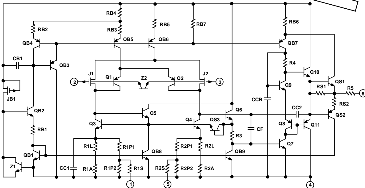
Simplified Schematic
