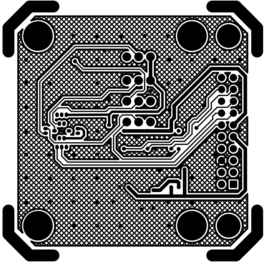
XL346 SENSOR BOARD LAYER 5 (BOTTOM)
