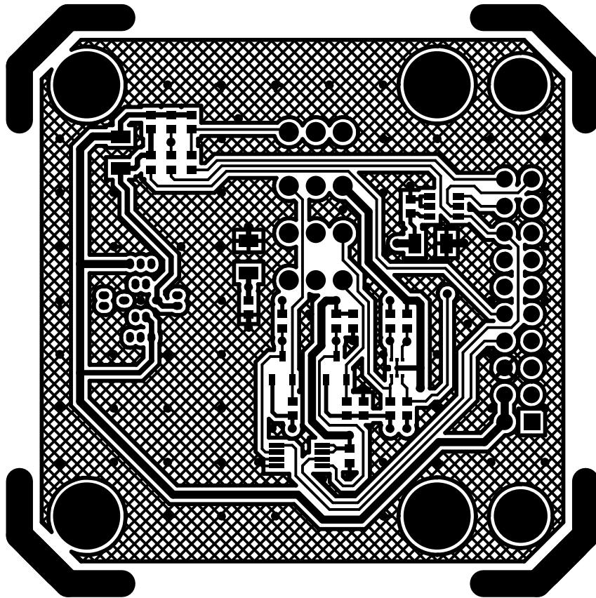
XL346 SENSOR BOARD LAYER 1 (TOP)
