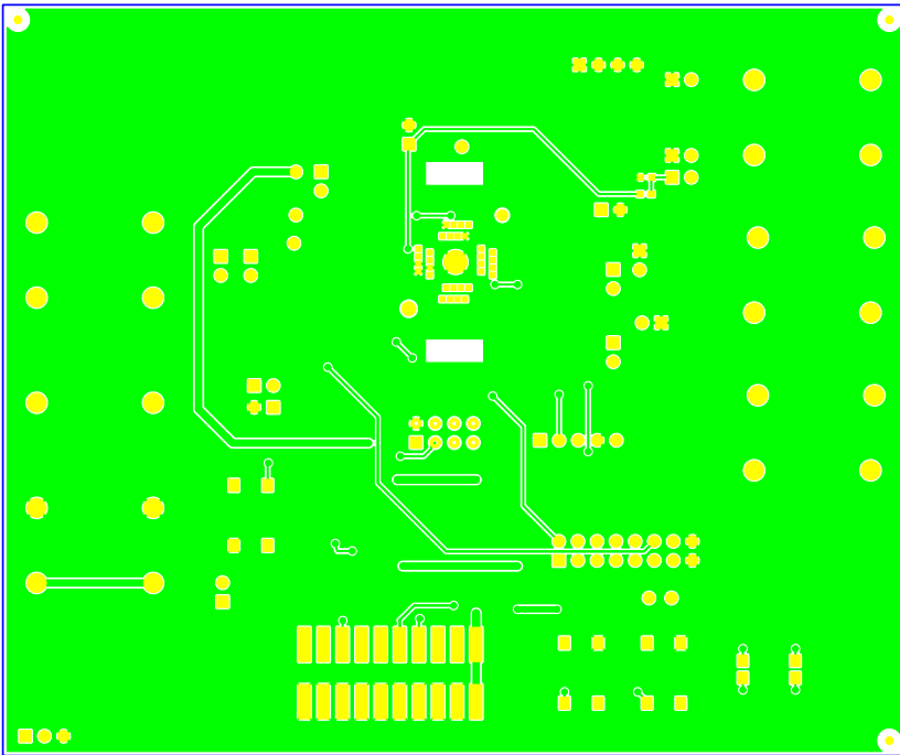
Gen 3 IBS ADuCM330 (Rev. B) - Top Side View. Top Side - Layer 1
