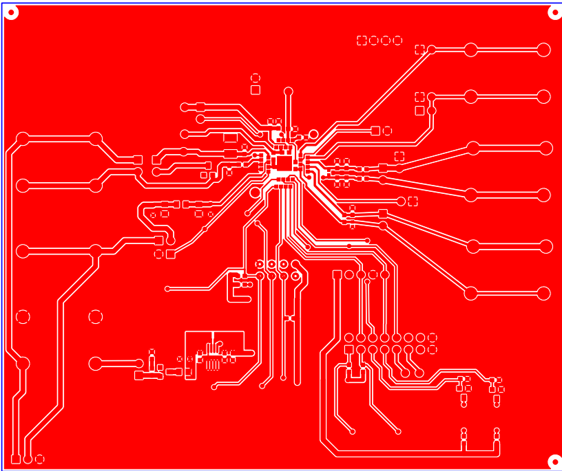
Gen 3 IBS ADuCM330 (Rev. B) - Top Side View. Bottom Side - Layer 2
