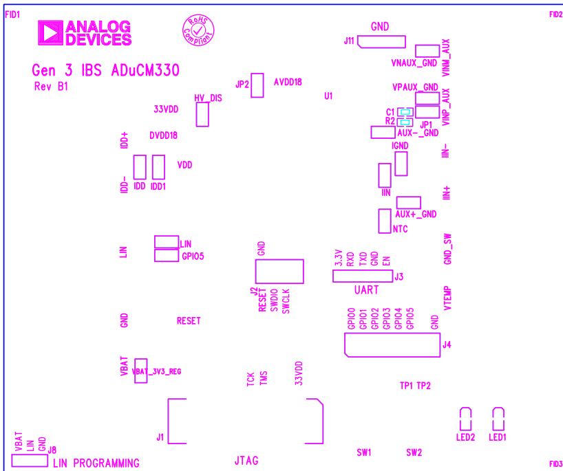
Gen 3 IBS ADuCM330 (Rev. B) – Top Side View.
