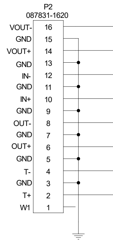
LTpowerAnalyzer 16-pin Molex Socket
