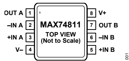
Figure 1. 8-Lead MSOP (RM-8)
