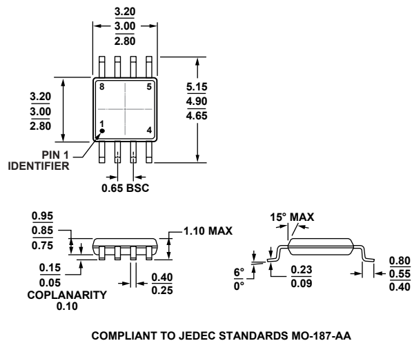
Figure 28. 8-Lead Mini Small Outline Package [MSOP] (RM-8) Dimensions shown in millimeters
