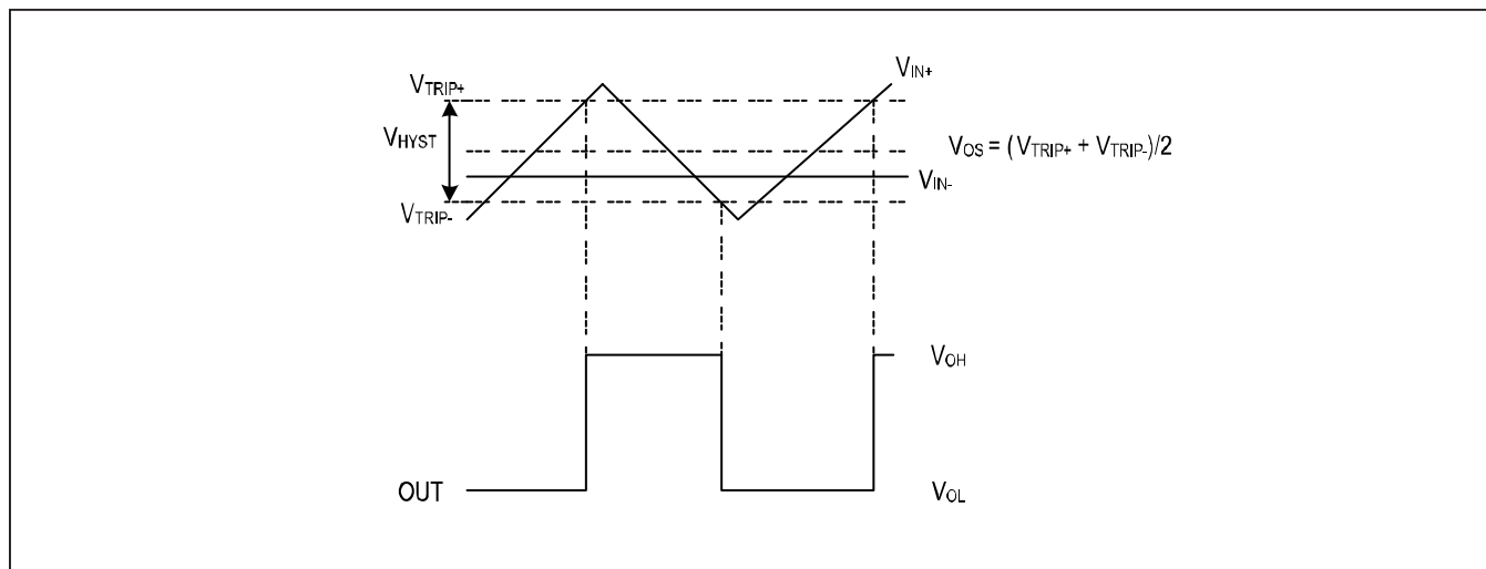
Figure 1. Hysteresis Band
