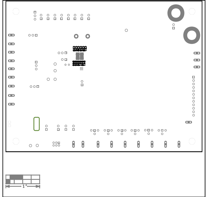
MAX25561 EV Kit Component Placement Guide—Bottom Silkscreen
