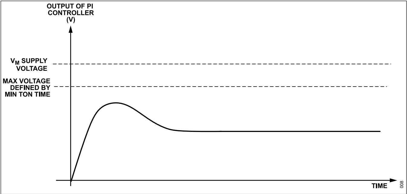
Figure 5. HS Configuration Maximal Voltage Graph
