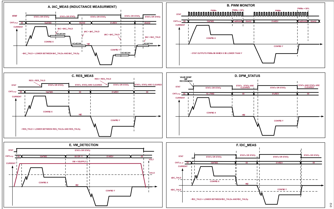
Figure 9. STATUS Output Monitor Pin - Differential
