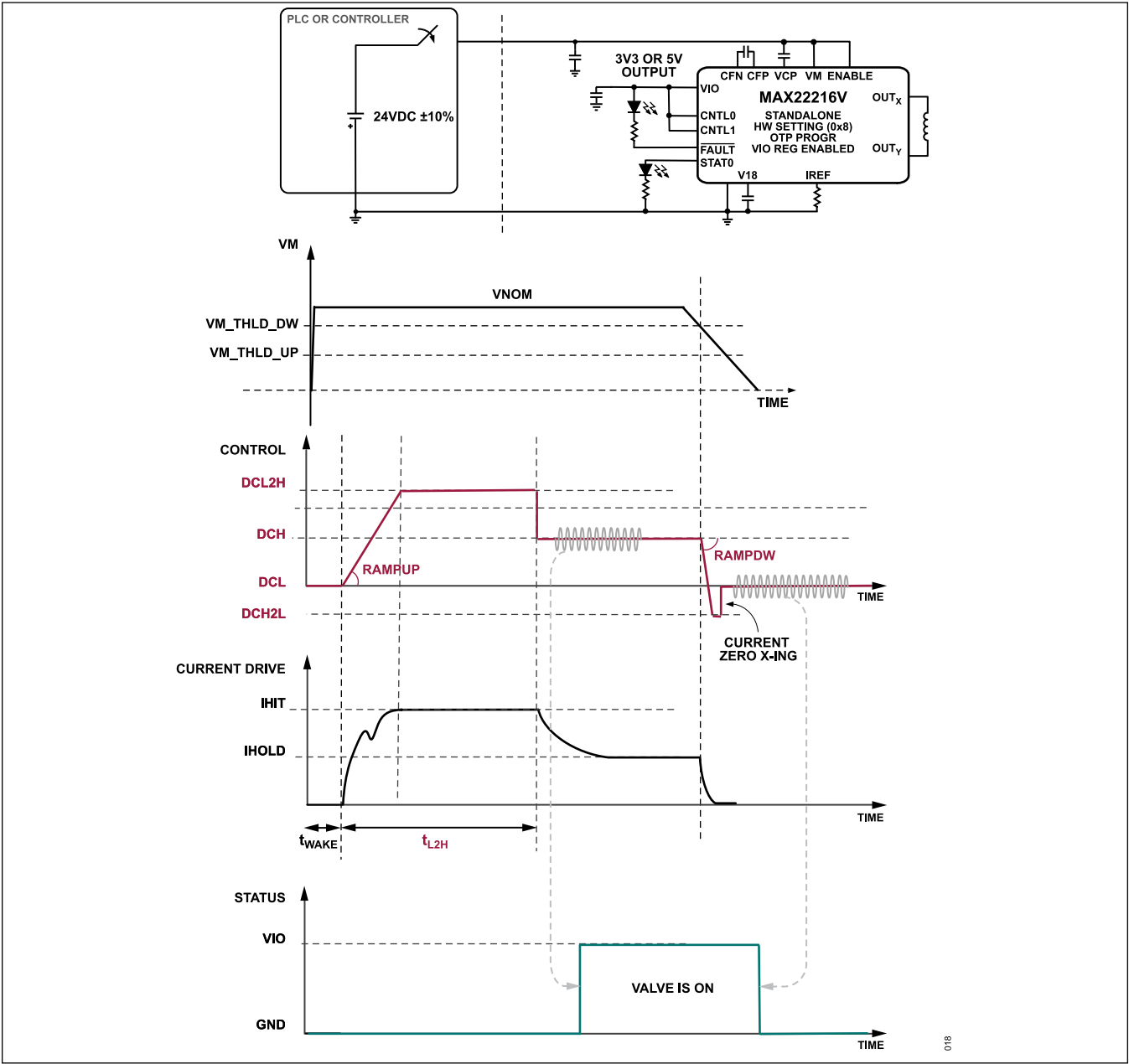
Figure 15. Standalone - V_M Switching
