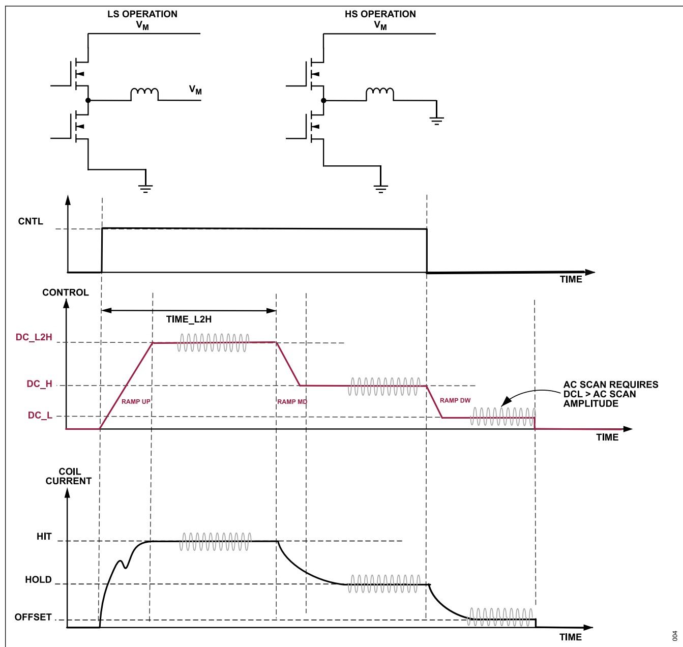
Figure 1. Single-Ended Configuration
