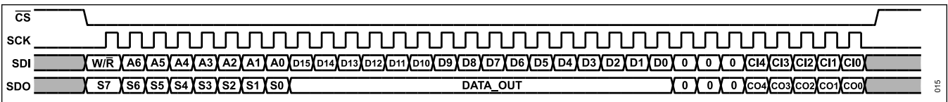
Figure 12. SPI Datagram with CRC
