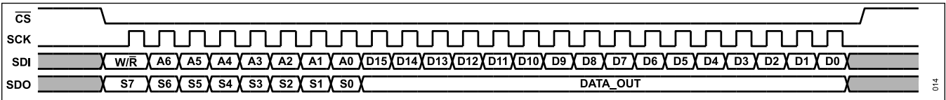
Figure 11. SPI Datagram without CRC
