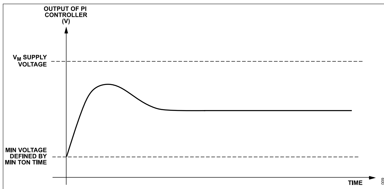
Figure 6. LS Configuration Minimal Voltage Graph
