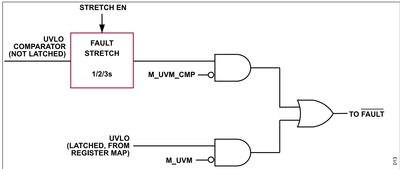
Figure 10. Fault Output Schematic
