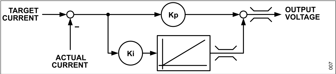
Figure 4. Block Diagram of Current Control Loop
