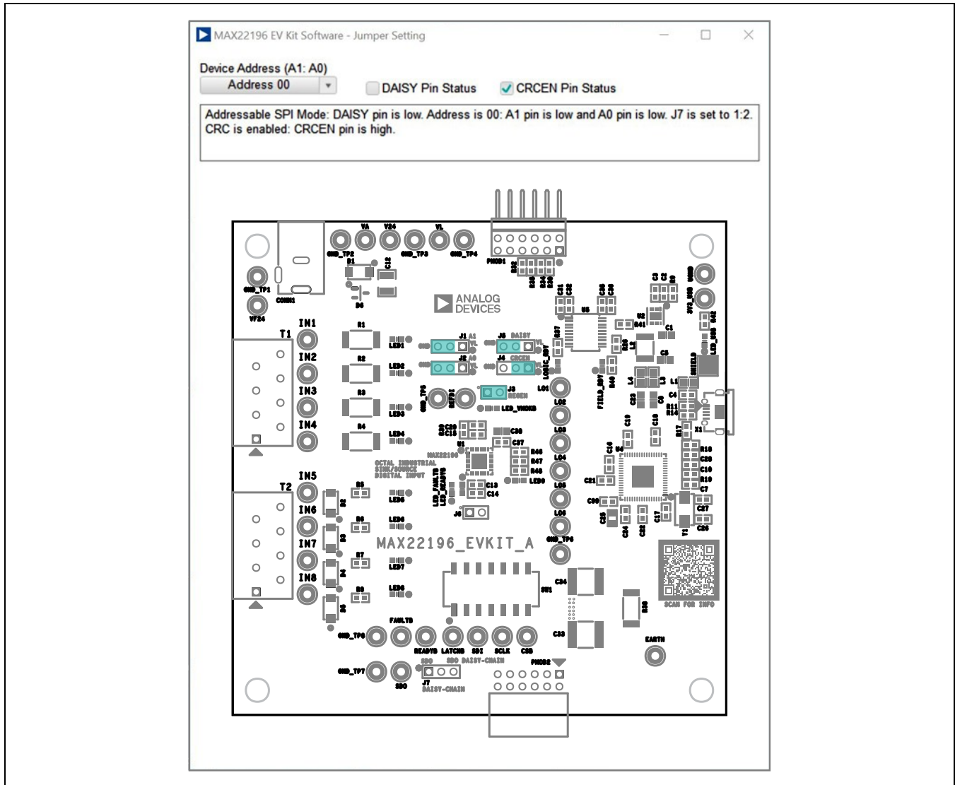
Figure 5. MAX22196 EV Kit Software—Jumper Setting Diagram
