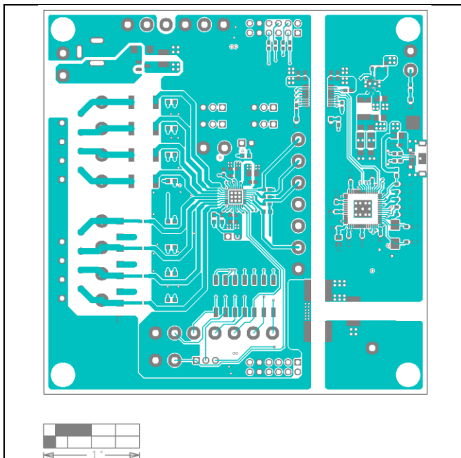
MAX22196 EV Kit PCB Layout—Top
