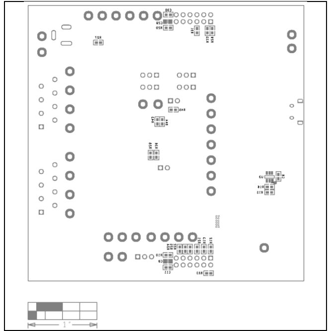
MAX22196 EV Kit Component Placement Guide—Bottom Silkscreen
