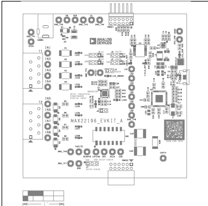
MAX22196 EV Kit Component Placement Guide—Top Silkscreen
