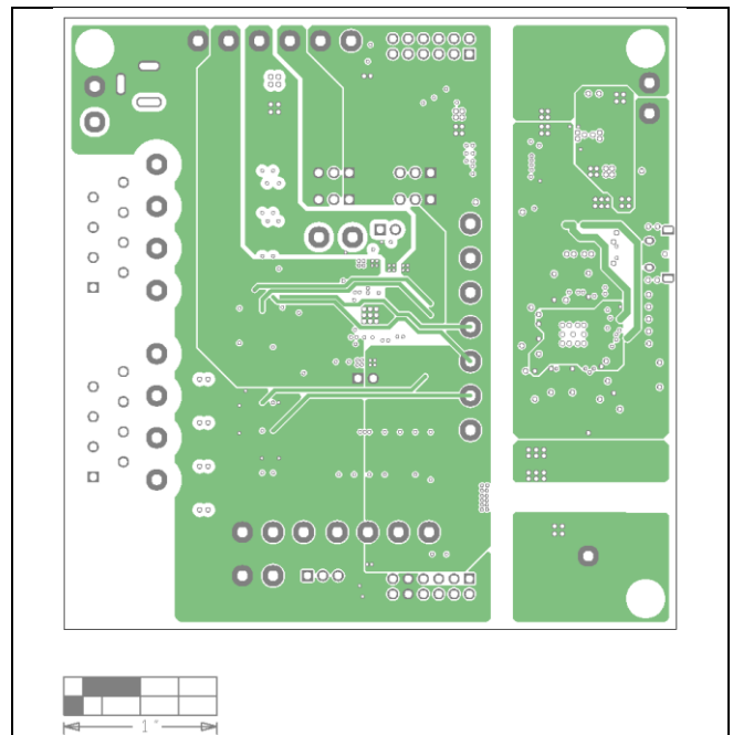
MAX22196 EV Kit PCB Layout—Layer 3
