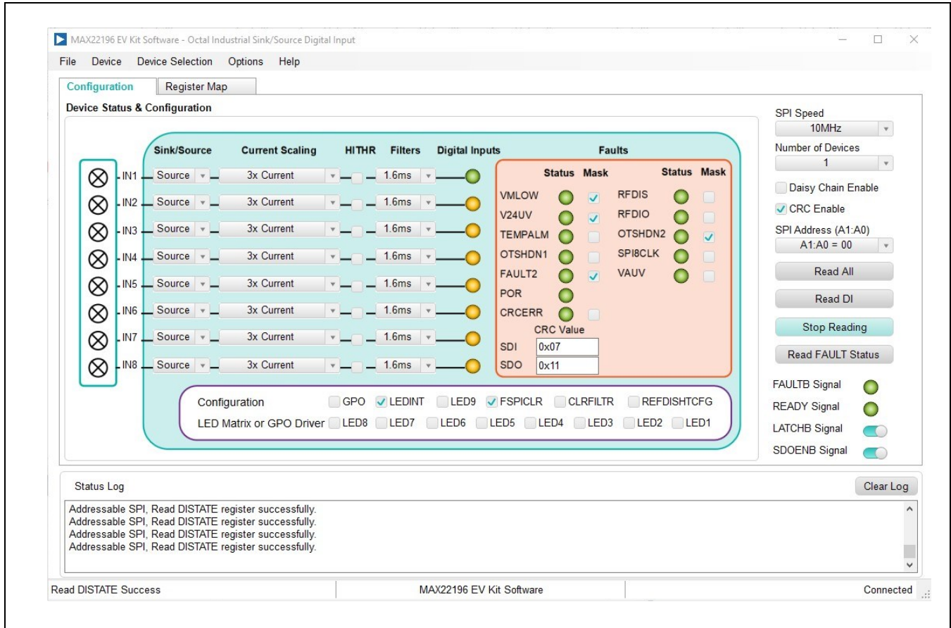
Figure 3. MAX22196 EV Kit Software—Type 2 Source Mode Configuration
