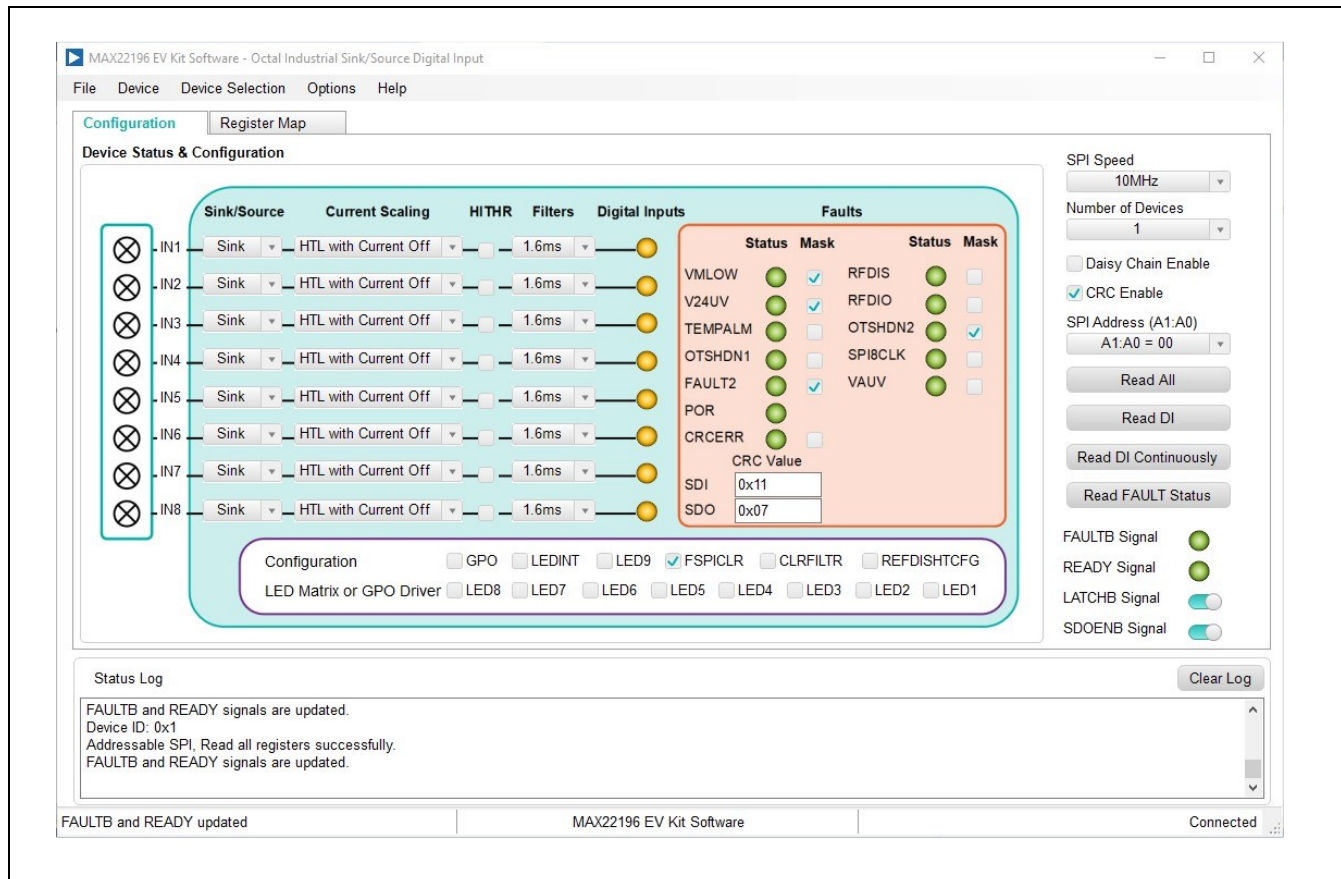
Figure 1. MAX22196 EV Kit Software Startup Window
