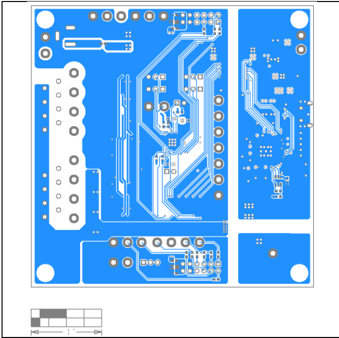
MAX22196 EV Kit PCB Layout—Bottom
