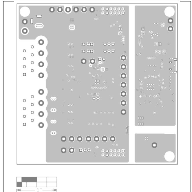
MAX22196 EV Kit PCB Layout—Layer 2
