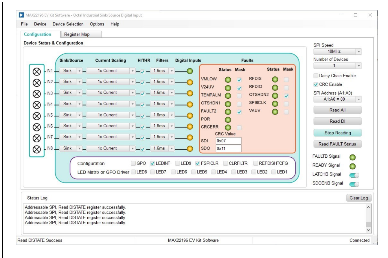
Figure 2. MAX22196 EV Kit Software—Type 1/3 Sink Mode Configuration
