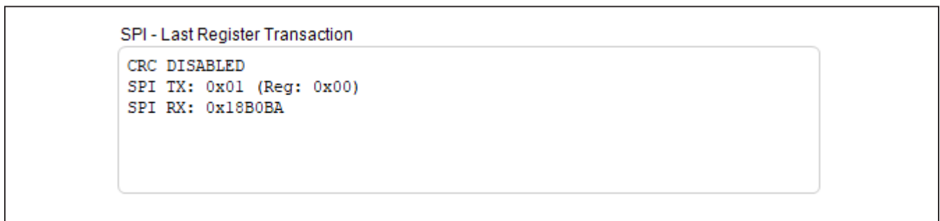
Figure 4. SPI Read Transaction with CRC Disabled
