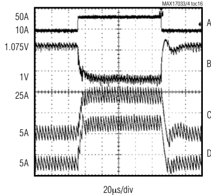
MAX17034 LOAD-TRANSIENT RESPONSE (HFM MODE)
