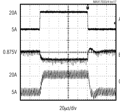
MAX17034 LOAD-TRANSIENT RESPONSE (LFM MODE)
