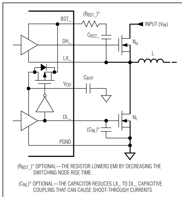
Figure 11. Gate Drive Circuit
