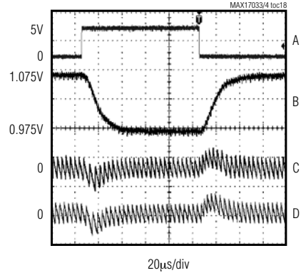
MAX17034 \overline{S\overline{H\overline{D\overline{N}}} = GND , VID CODE CHANGE
