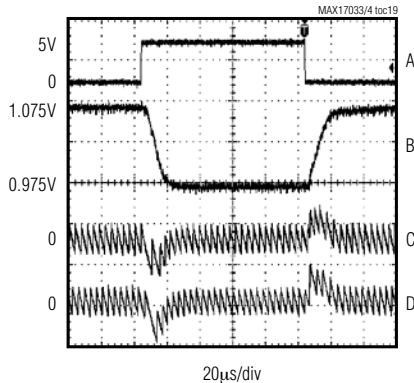
MAX17034 \overline{S\overline{H\overline{D\overline{N}}} = V_{DD} , VID CODE CHANGE
