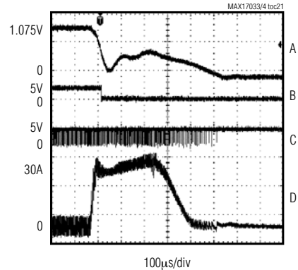
MAX17034 OUTPUT UNDERVOLTAGE FAULT
