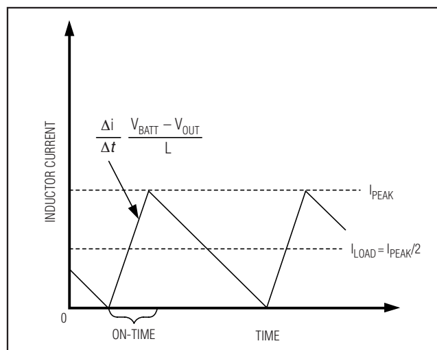
Figure 9. Pulse-Skipping/Discontinuous Crossover Point
