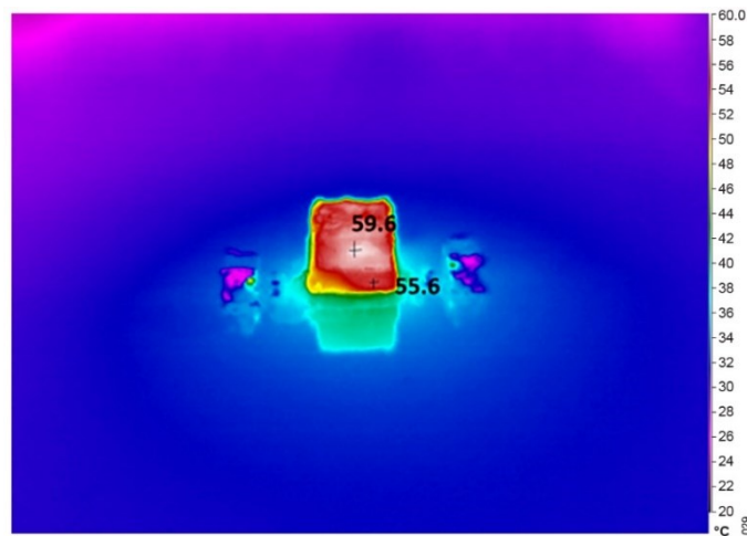
Figure 29. Thermal Image at 12V IN , 1V, 15A Output, No Airflow and Heat Sink, T_A = 25^{\circ}\text{C} .
