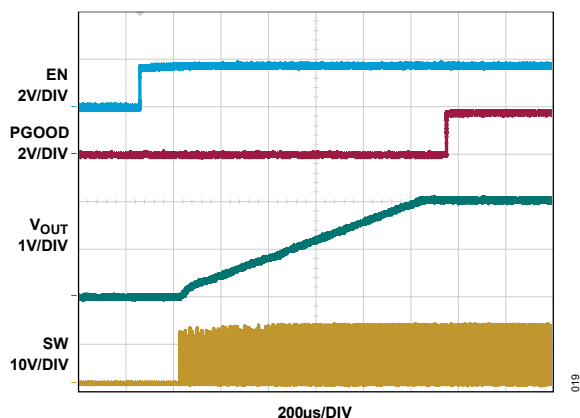
Figure 19. Startup without Pre-Bias
