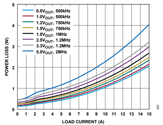
Figure 7. Power Loss, V_{IN} = 12\text{V} , V_{BIAS} = 3.3\text{V}
