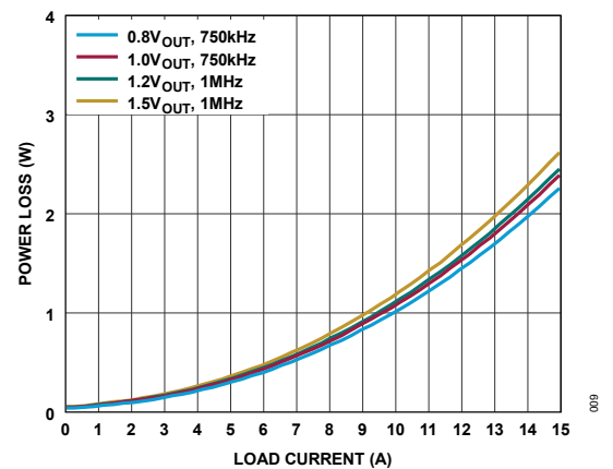
Figure 9. Power Loss, V_{IN} = 3.3\text{V} , V_{BIAS} = 3.3\text{V}
