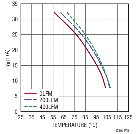
Figure 9. Derating, 4-Channel Paralleled V_{IN} = 3.3V , V_{OUT} = 0.8V DC3164A-B Demo Board
