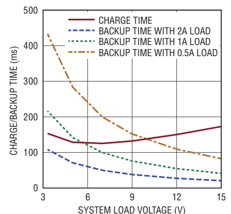
Approximate Charge/Backup Time per 1mF of Storage Cap (40V Backup)
