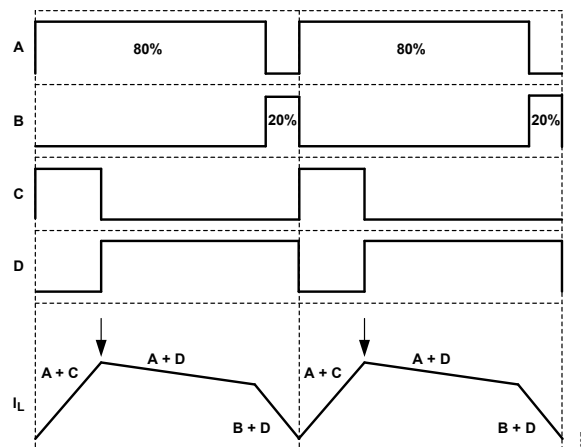
Figure 33. Peak-Boost in Buck-Boost Region ( V_{IN} \lesssim V_{OUT} )
