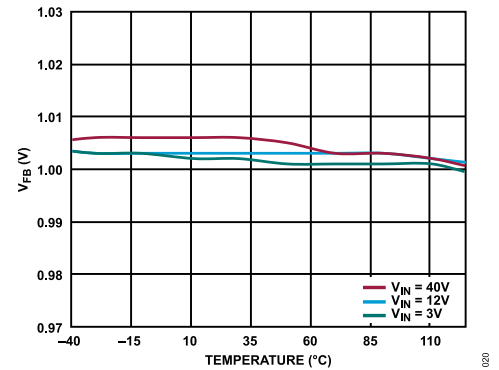
Figure 17. FB Regulation vs Temperature
