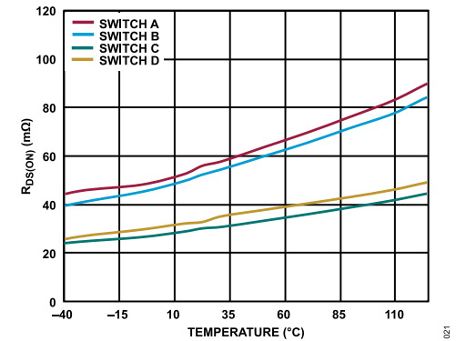
Figure 18. Power Switch R_{DS(ON)}
