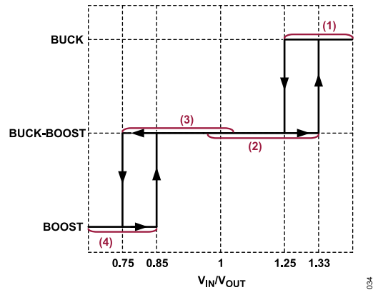
Figure 30. Operation Region vs V_{IN}/V_{OUT} Ratio
