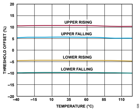
Figure 23. \overline{PGOOD} Threshold
