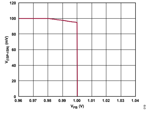
Figure 16. V_{(ISP-ISN)} Regulation vs V_{FB}
