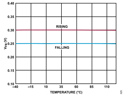
Figure 22. FB Short-Circuit Threshold
