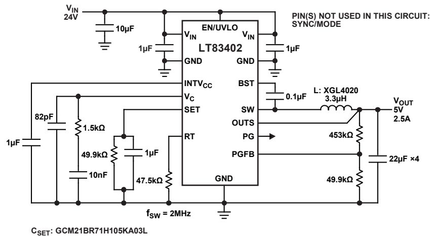
Figure 61. 5V 2.5A 2MHz Step-Down Converter with Fast Start-Up, and Power Good
