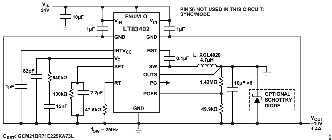
Figure 62. Negative 10V 1.4A 2MHz Step-Down Converter with Fast Start-Up, and Power Good
