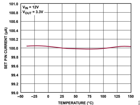
Figure 13. SET Pin Current vs. Temperature
