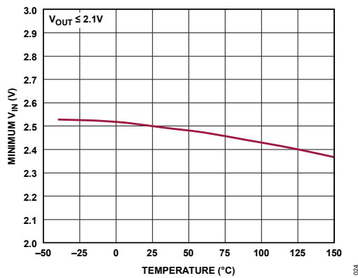
Figure 24. Minimum V_{IN} vs. Temperature
