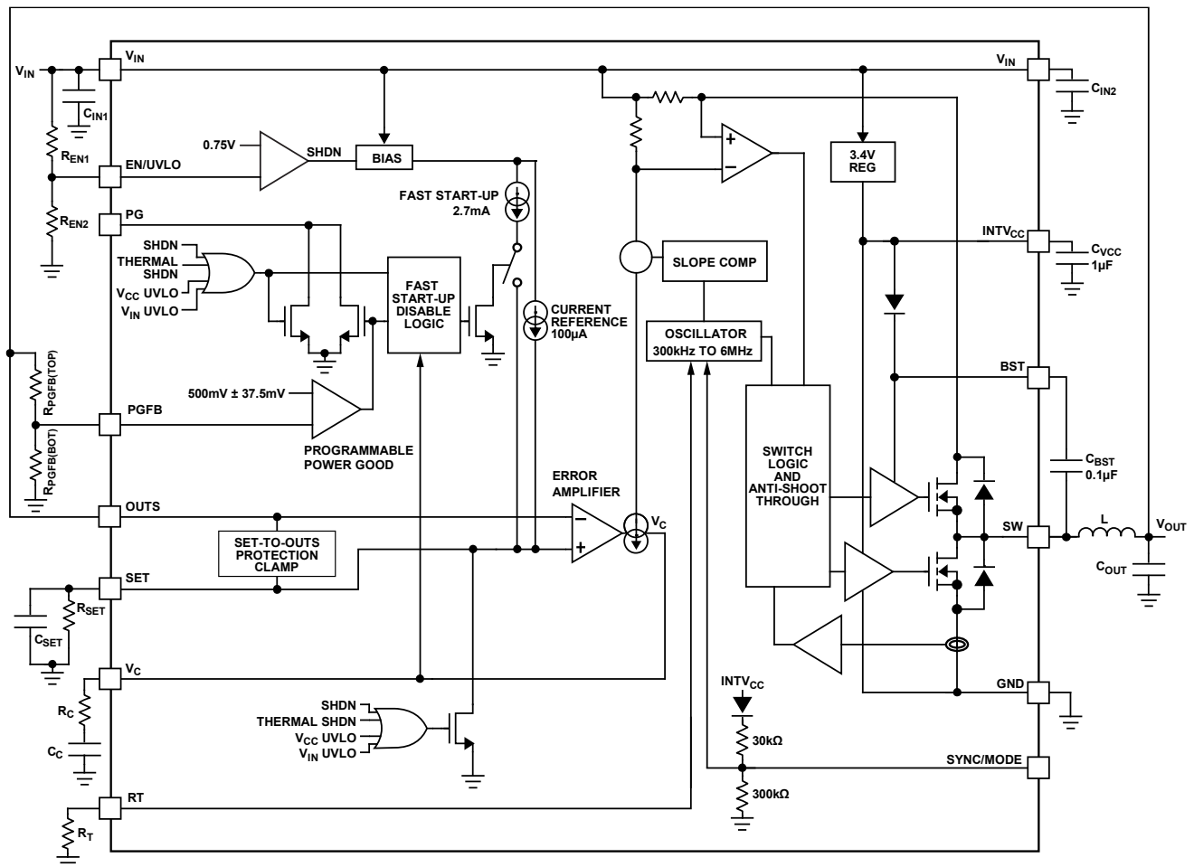
Figure 46. Block Diagram
