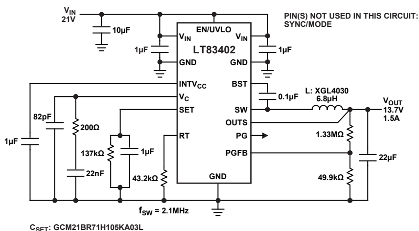
Figure 60. 13.7V 1.5A 2.1MHz Step-Down Converter with Fast Start-Up, and Power Good
