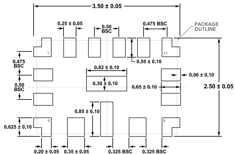
Figure 63. Tiny 15-Lead 3mm x 2mm LFCSP
