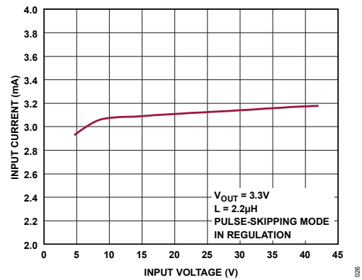
Figure 26. No-Load Supply Current
