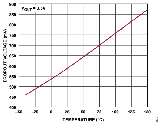
Figure 22. V_{IN} to V_{SET} Dropout Voltage vs. Temperature
