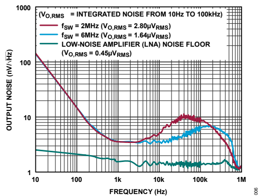
Figure 6. Noise Spectral Density vs. f_{SW} See Typical Application Circuit (Figure 59)
