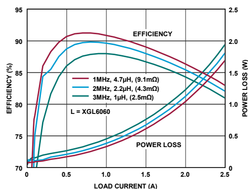
Figure 2. 12V to 3.3V Efficiency
