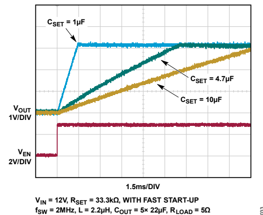
Figure 33. Soft-Start Waveforms
