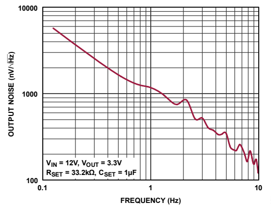
Figure 7. Noise Spectral Density (0.1Hz to 10Hz)
