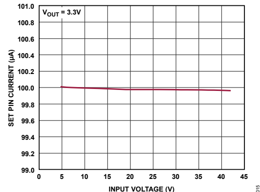
Figure 15. Set Pin Current vs. V_{IN}
