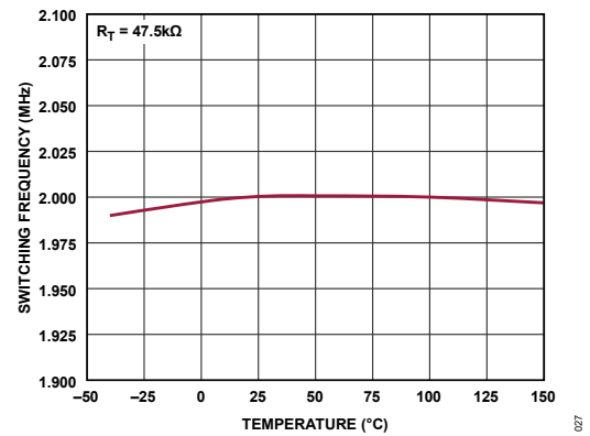
Figure 27. Switching Frequency vs. Temperature
