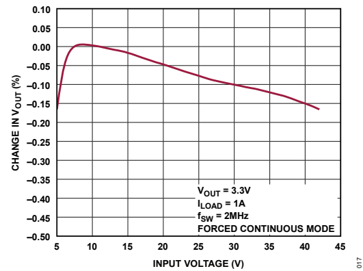
Figure 17. Line Regulation
