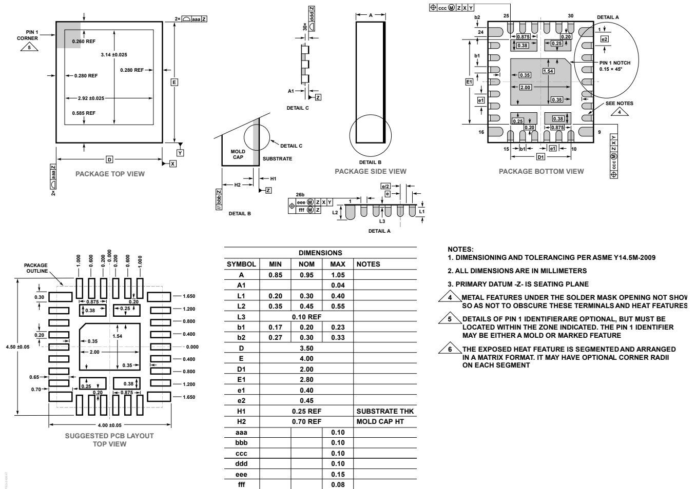
Figure 42. 30-Lead (3.5mm x 4mm) LQFN Package (CC-30-10) Dimensions Shown in Millimeters
