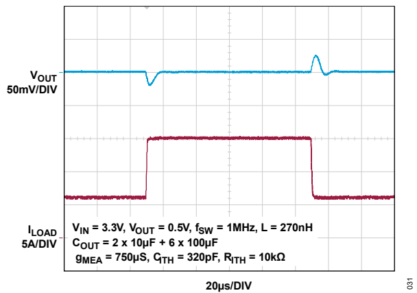
Figure 31. LT7176P-1, Dual Phase, Transient Response: Load Current Step, 6A to 15A
