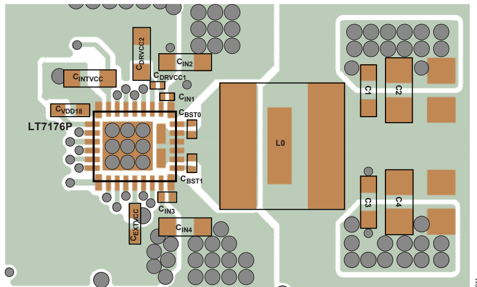
Figure 38. LT7176P Recommended PCB Layout
