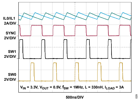
Figure 29. LT7176P-1 Inductor Currents, Switch Pins, and SYNC Output Waveforms
