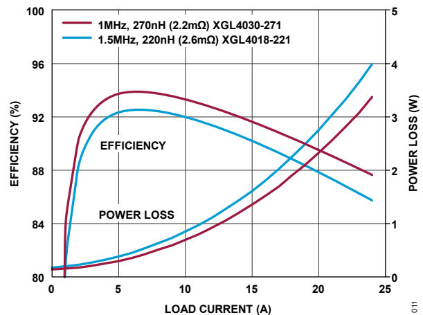
Figure 11. LT7176P-1 3.3V IN to 1.0V OUT Efficiency
