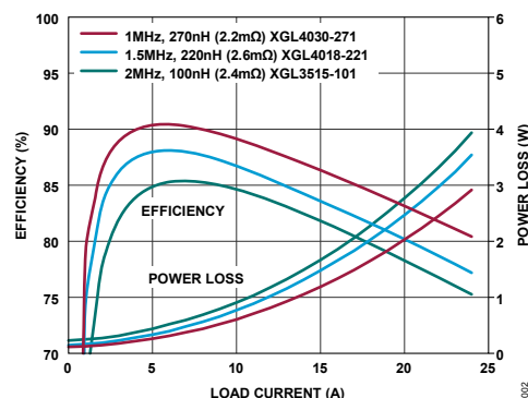
Figure 2. LT7176P-1 3.3V IN to 0.5V OUT Efficiency
