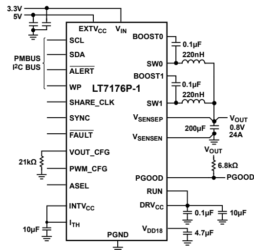
Figure 41. LT7176P-1 3.3V to 0.8V, 1MHz, 24A Dual-Phase Regulator
