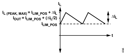
Figure 32. Positive Valley Current Limit
