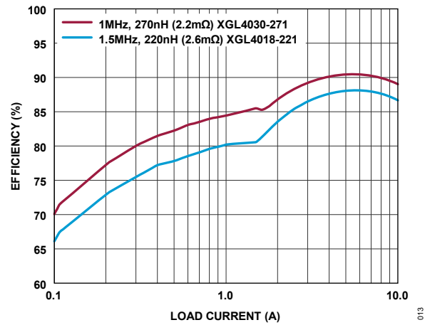
Figure 13. LT7176P-1 3.3V IN to 0.5V OUT PSM Efficiency
