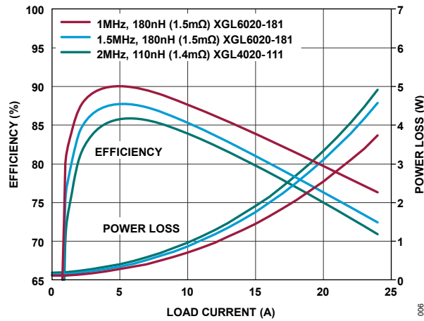
Figure 6. LT7176P 3.3V IN to 0.5V OUT Efficiency
