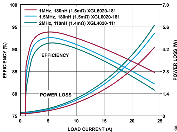
Figure 8. LT7176P 3.3V IN to 1.0V OUT Efficiency
