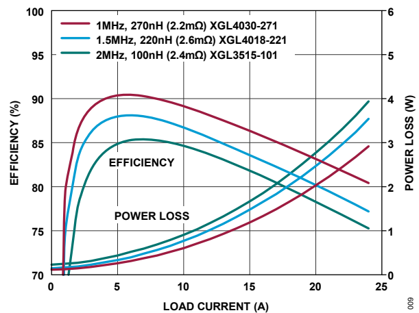
Figure 9. LT7176P-1 3.3V IN to 0.5V OUT Efficiency
