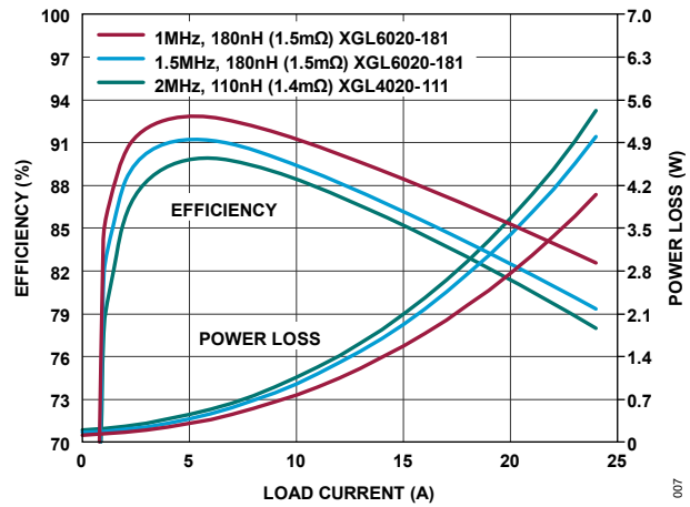
Figure 7. LT7176P 3.3V IN to 0.8V OUT Efficiency
