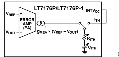
Figure 35. Programmable Internal Compensation
