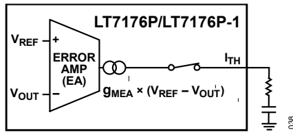
Figure 34. External Compensation with Programmable g_{MEA}
