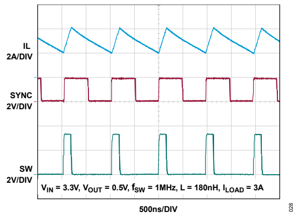
Figure 28. LT7176P Inductor Current, Switch Pin, and SYNC Output Waveforms
