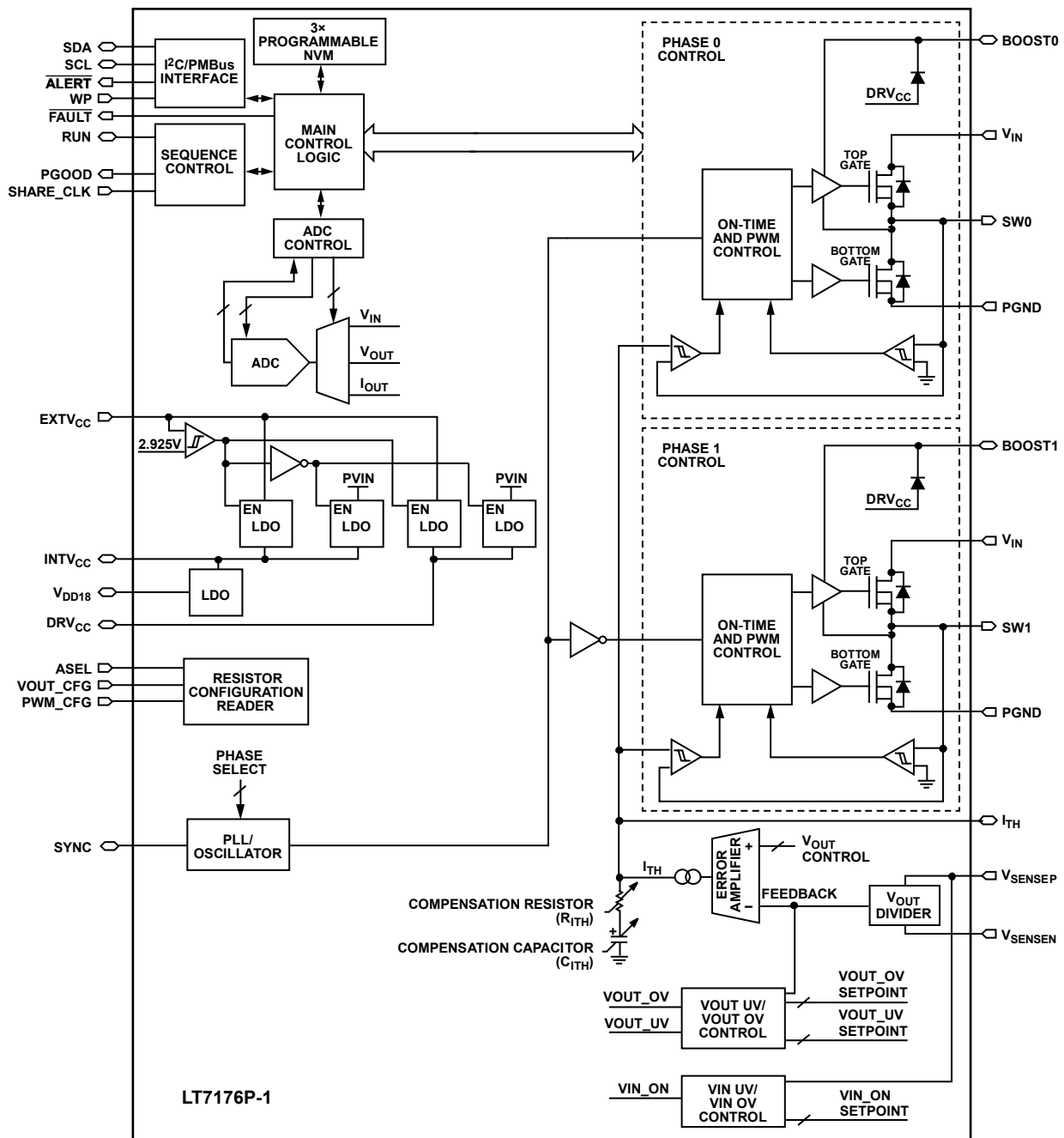
Figure 4. LT7176P-1 Functional Block Diagram
