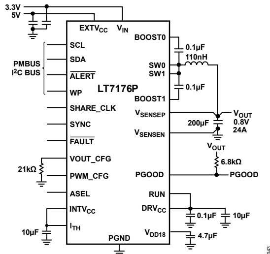
Figure 40. LT7176P 3.3V to 0.8V, 1MHz, 24A Single-Phase Regulator
