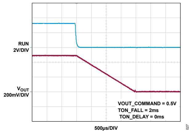
Figure 27. Soft-Off Ramp
