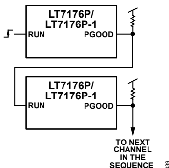
Figure 36. Event-Based Sequencing
