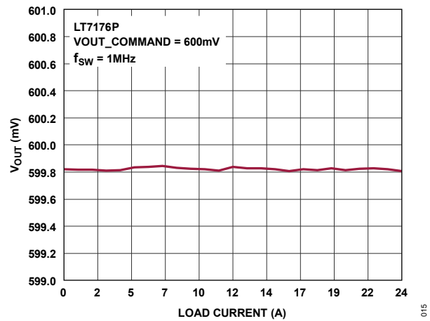
Figure 15. Load Regulation
