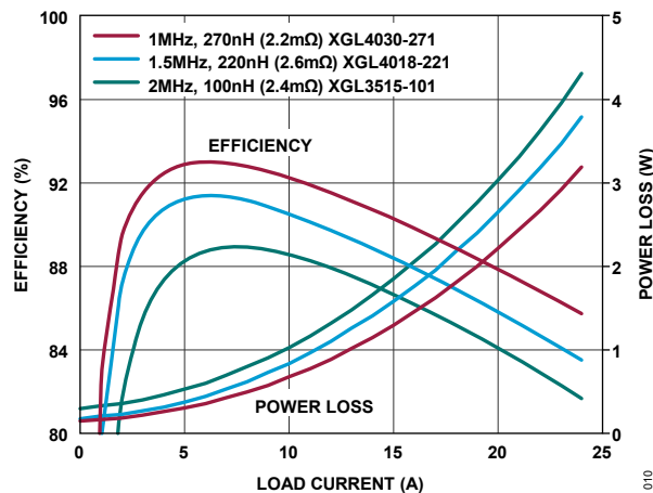
Figure 10. LT7176P-1 3.3V IN to 0.8V OUT Efficiency
