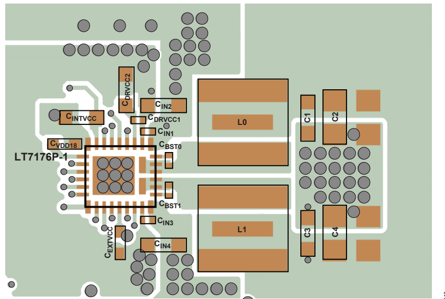
Figure 39. LT7176P-1 Recommended PCB Layout
