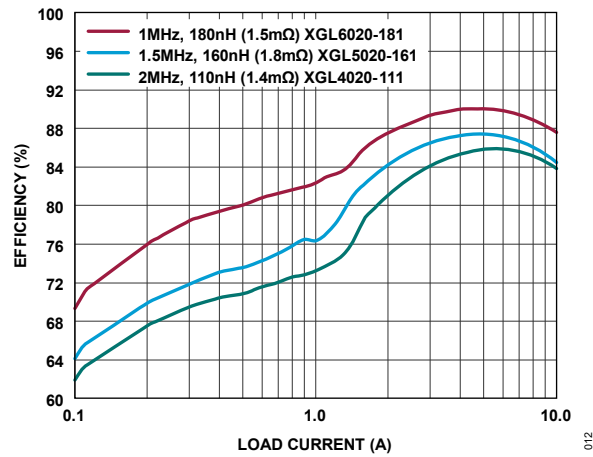
Figure 12. LT7176P 3.3V IN to 0.5V OUT PSM Efficiency
