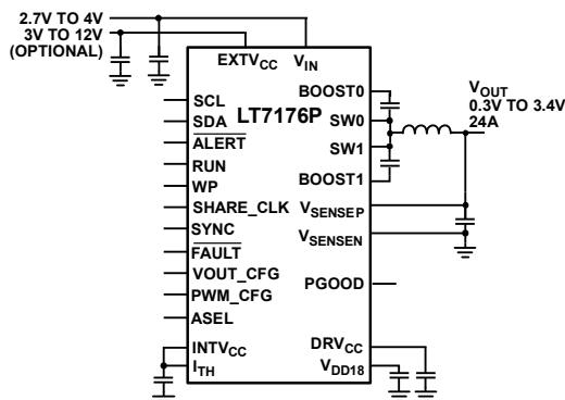
Figure 1. Typical Application for the LT7176P
