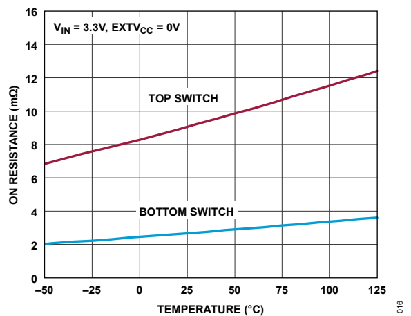
Figure 16. LT7176P-1 Switch On Resistance Per-Phase vs. Temperature
