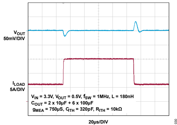
Figure 30. LT7176P, Single Phase, Transient Response: Load Current Step, 6A to 15A
