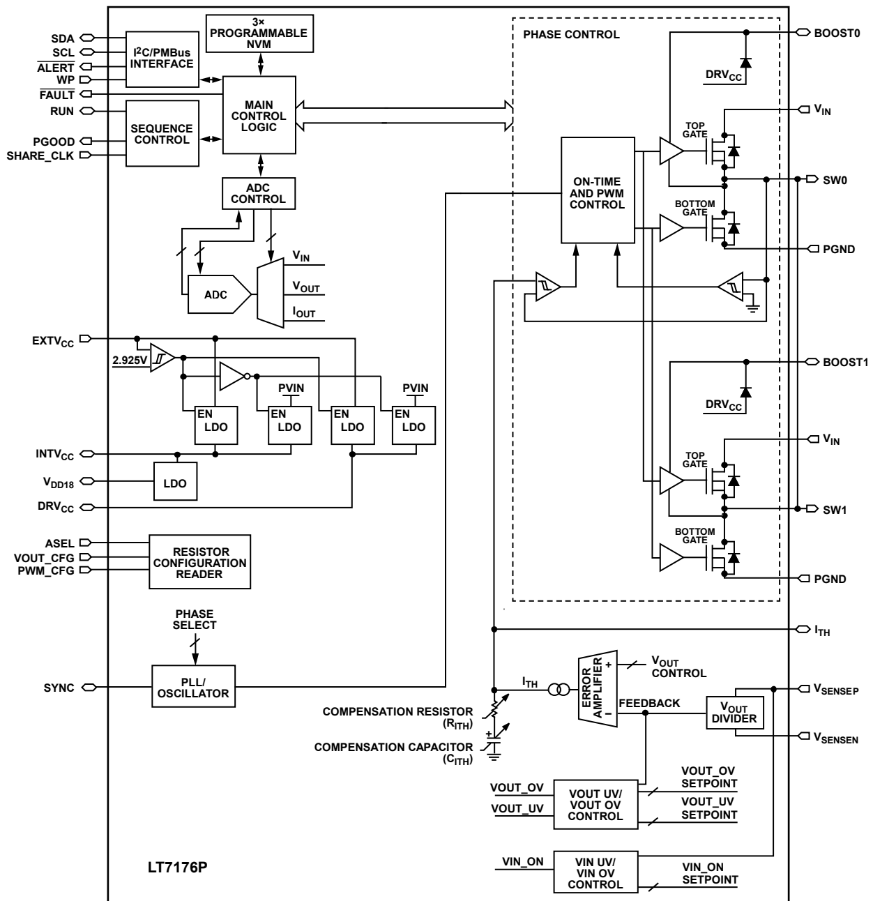
Figure 3. LT7176P Functional Block Diagram
