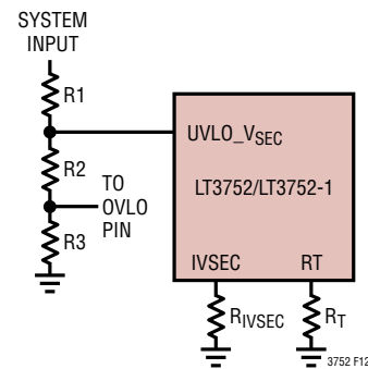
Figure 12. Programming D_{VSEC}
