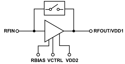
Figure 129. Simplified Schematic
