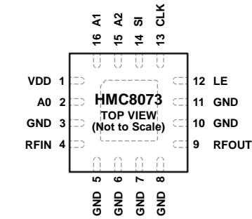
Figure 3. Pin Configuration
