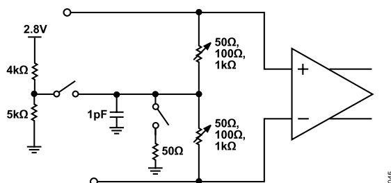
Figure 50. On-Chip Termination Network for VCXO and Reference Buffers
