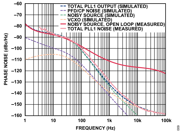
Figure 7. Closed-Loop Phase Noise at 122.88 MHz, PLL1 Measurement vs. Simulated, Noisy Reference Source, ~70 Hz Loop Bandwidth, 80° Phase Margin
