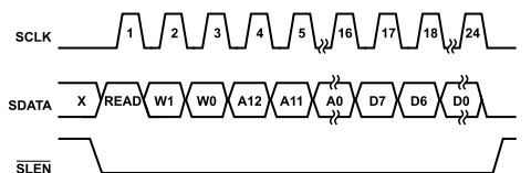
Figure 51. SPI Timing Diagram, Read Operation
