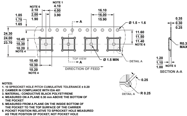
Figure 54. LFCSP Tape and Reel Outline Dimensions Dimensions shown in millimeters
