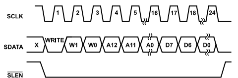
Figure 52. SPI Timing Diagram, Write Operation
