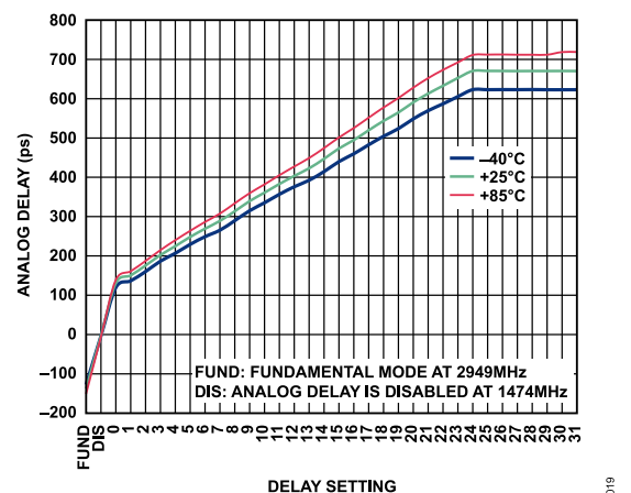
Figure 19. Analog Delay vs. Delay Setting over Temperature, LVPECL at 1474.56 MHz
