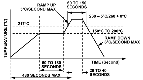
Figure 53. Pb-Free Reflow Solder Profile
