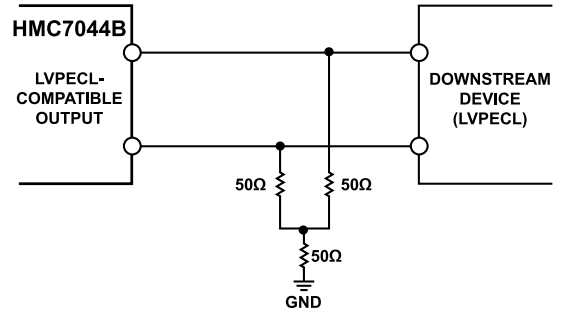
Figure 33. DC-Coupled LVPECL Output Driver
