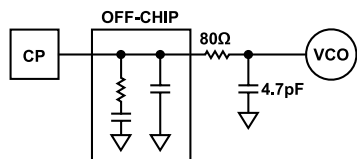
Figure 44. On-Chip RC Circuit
