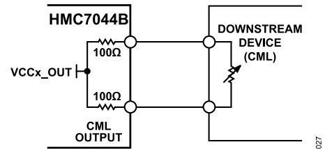
Figure 35. DC-Coupled CML (Internal) Output Driver
