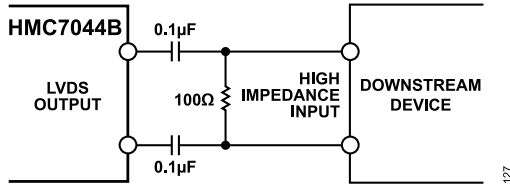
Figure 27. AC-Coupled LVDS Output Driver
