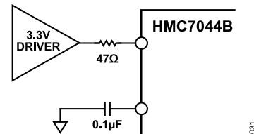
Figure 36. CLKIN0, CLKIN1, CLKIN2, CLKIN3, and OSCIN Input, Single-Ended Mode
