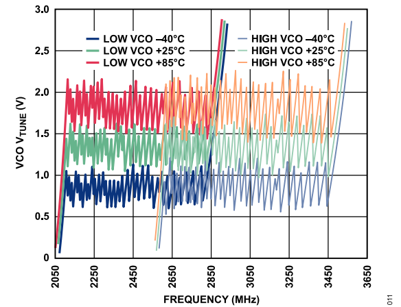
Figure 12. VCO V_{TUNE} vs. Frequency
