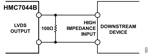
Figure 32. DC-Coupled LVDS Output Driver
