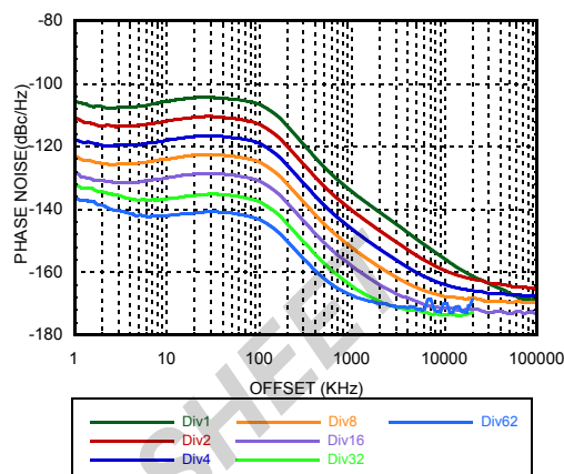
Figure 52. Auxiliary LO Output, Fractional Mode Closed Loop Phase Noise @4100 MHz with various divider ratios [1]
