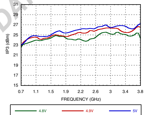
Figure 4. High Side LO Input IP3 vs. VGATE [1]
