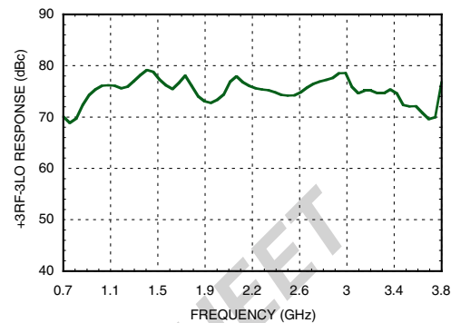
Figure 14. +3RF -3LO Response vs. Frequency over Temperature [1][2][3]
