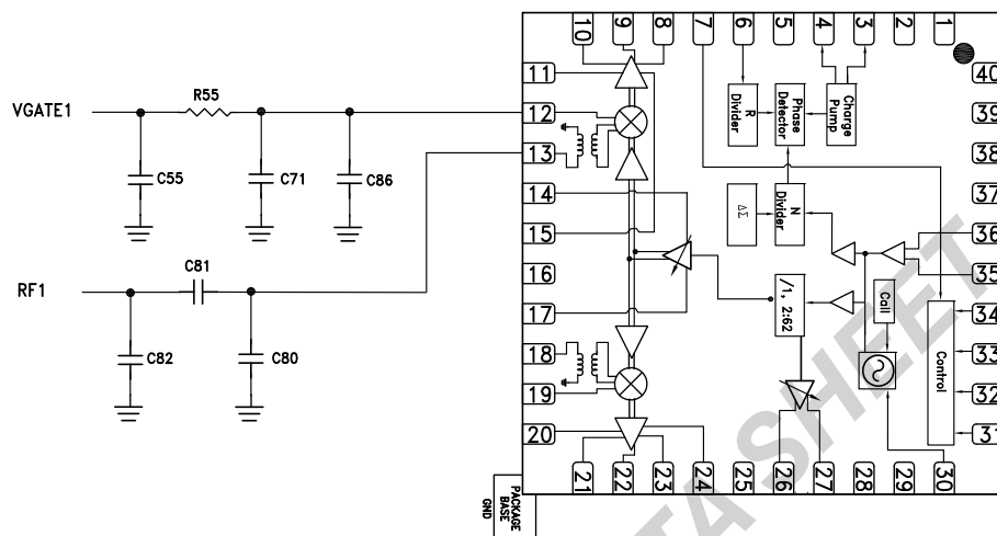
Figure 80. Application Circuit for Narrowband RF Input Matching
