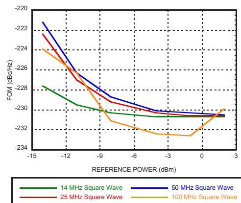
Figure 59. Reference Input Sensitivity, Square Wave, 50 \Omega [3]
