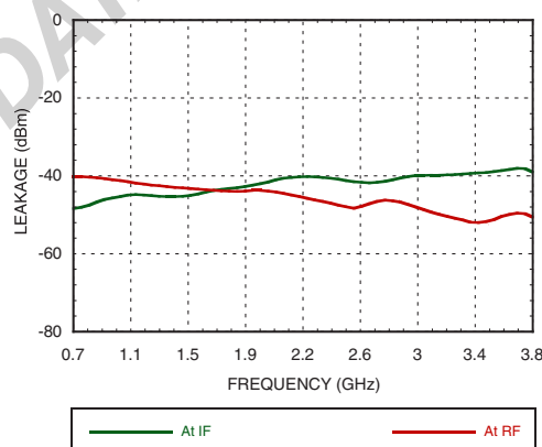
Figure 10. LO Leakage vs. Frequency [2][3]
