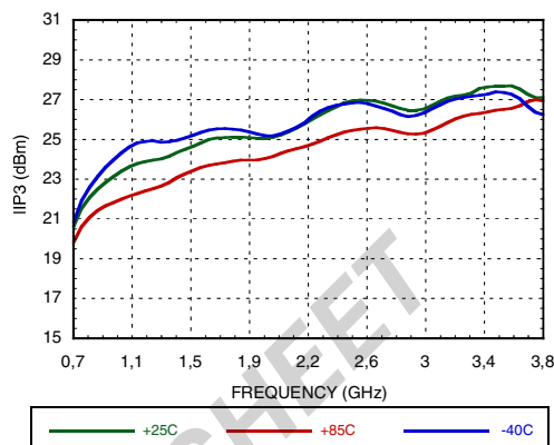
Figure 32. Low Side LO Input IP3 vs. Frequency @ VGATE=4.8V[2]
