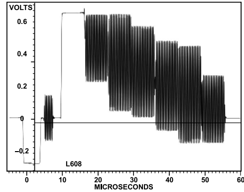
Figure 137. PAL Color Bars (75%)
