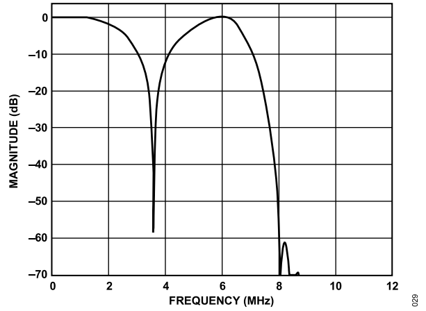
Figure 33. SD NTSC, Luma Notch Filter Response
