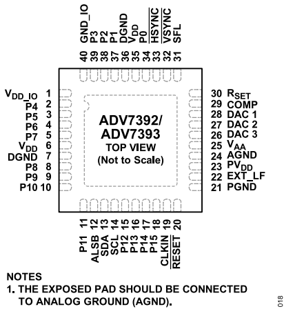
Figure 19. ADV7392/ADV7393 Pin Configuration (CP-40-9)
