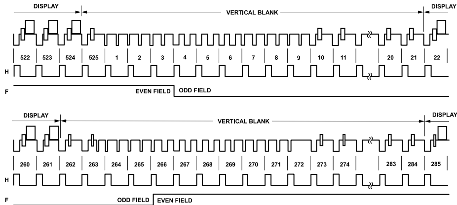
Figure 107. SD Timing Mode 0, Main Option, NTSC
