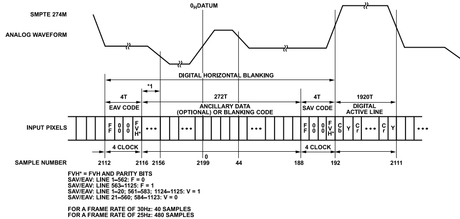
Figure 140. EAV/SAV Input Data Timing Diagram (SMPTE 274M)
