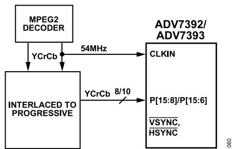
Figure 64. ED (at 54 MHz) Example Application
