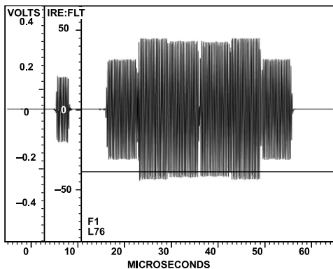
Figure 135. NTSC Luma
