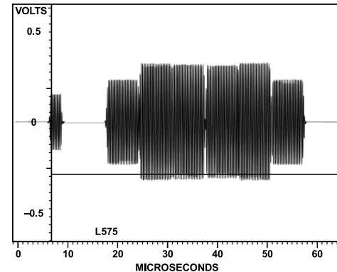
Figure 138. PAL Luma
