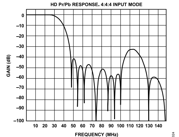
Figure 28. HD 4× Oversampling, PrPb (SSAF) Filter Response (4:4:4 Input)
