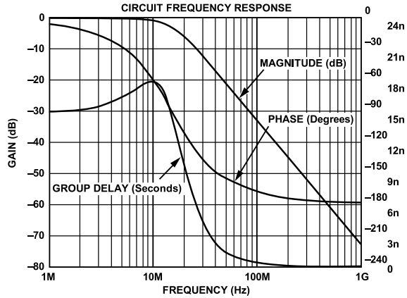
Figure 92. Output Filter Plot for SD, 16× Oversampling
