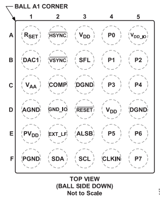
Figure 22. ADV7390BCBZ-A Pin Configuration
