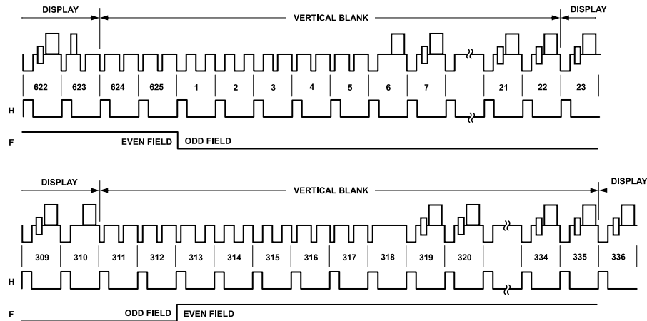
Figure 108. SD Timing Mode 0, Main Option, PAL
