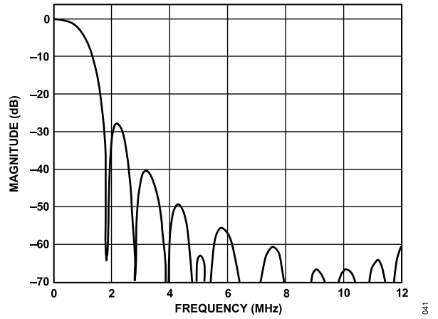
Figure 45. SD Chroma 1.0 MHz Low-Pass Filter Response
