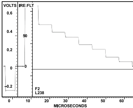
Figure 134. NTSC Color Bars (75%)
