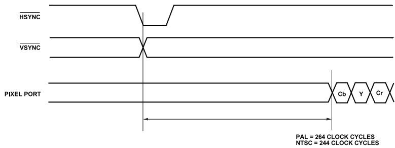
Figure 16. SD Input Timing Diagram (Timing Mode 1)
