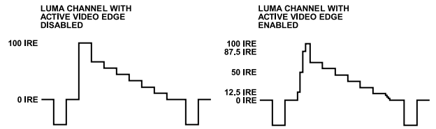
Figure 84. Example of Active Video Edge Functionality
