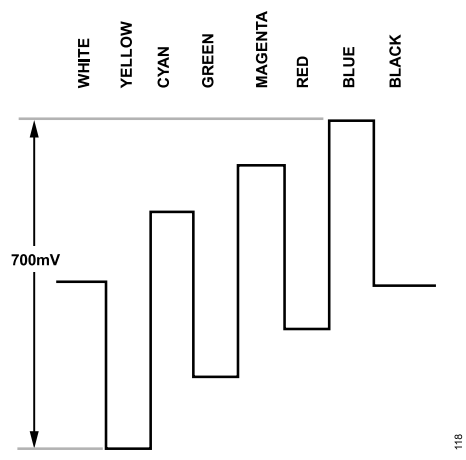
Figure 122. Pb Levels—NTSC
