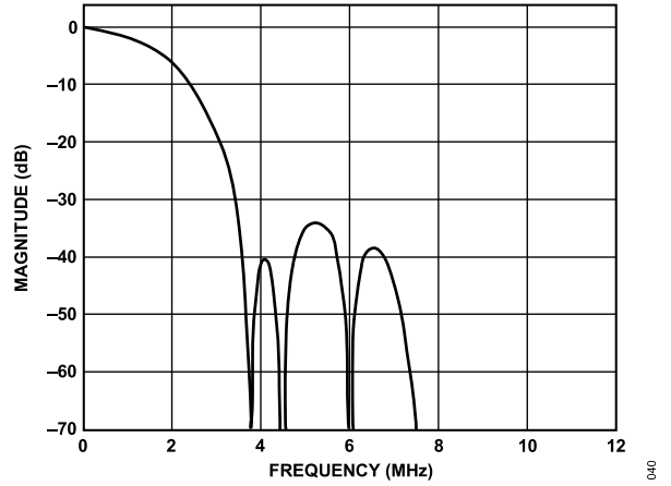
Figure 44. SD Chroma 1.3 MHz Low-Pass Filter Response
