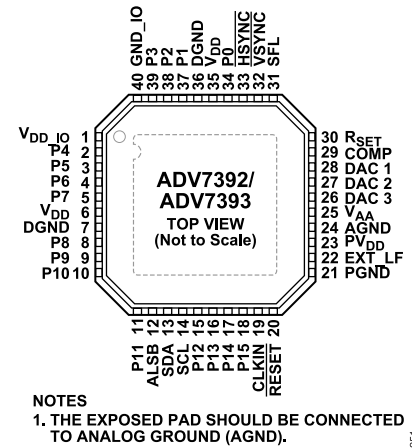
Figure 21. ADV7392/ADV7393 Pin Configuration (CP-40-1)
