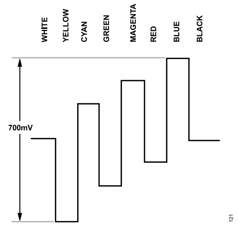
Figure 125. Pb Levels—PAL
