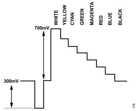
Figure 123. Y Levels—PAL
