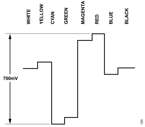
Figure 124. Pr Levels—PAL
