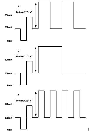
Figure 133. HD RGB Output Levels—RGB Sync Enabled
