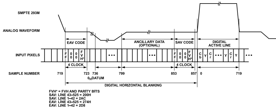
Figure 141. EAV/SAV Input Data Timing Diagram (SMPTE 293M)
