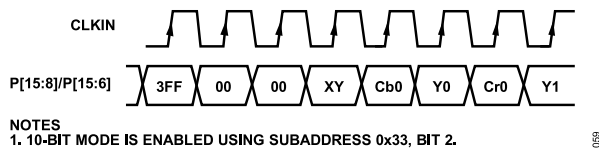
Figure 63. ED (at 54 MHz) Input Sequence (EAV/SAV)
