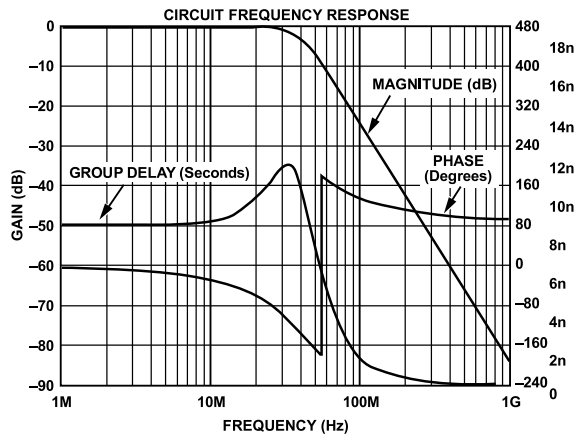
Figure 93. Output Filter Plot for ED, 8× Oversampling
