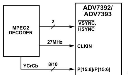
Figure 58. SD Example Application
