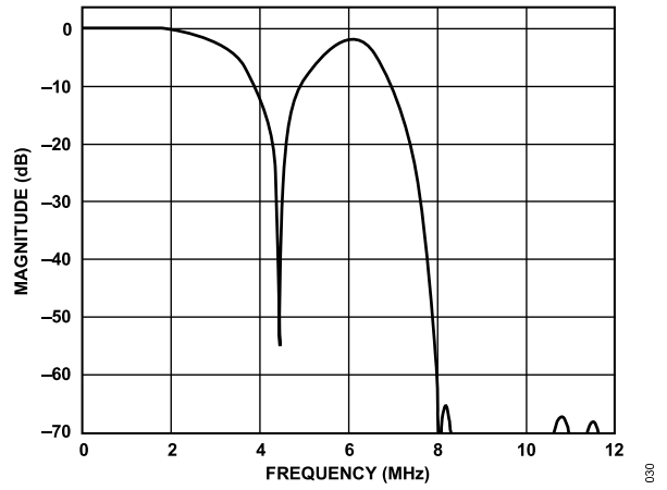
Figure 34. SD PAL, Luma Notch Filter Response
