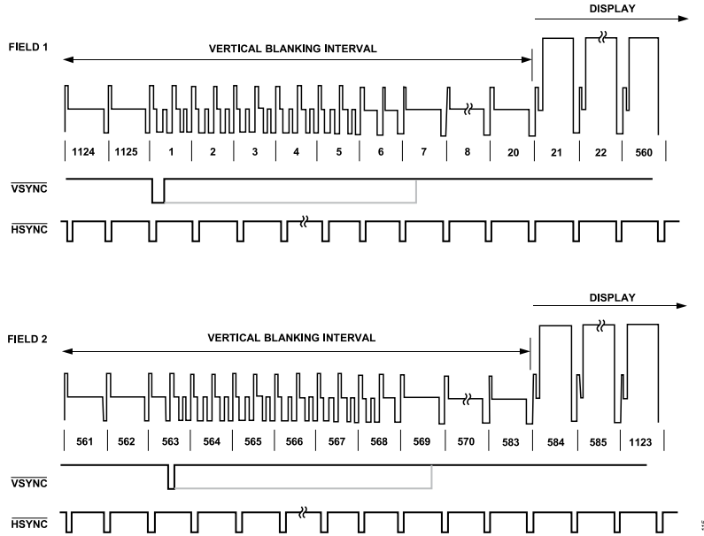
Figure 119. 1080i HSYNC and VSYNC Input Timing
