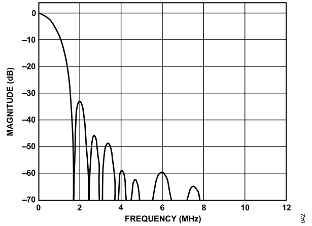
Figure 46. SD Chroma 0.65 MHz Low-Pass Filter Response
