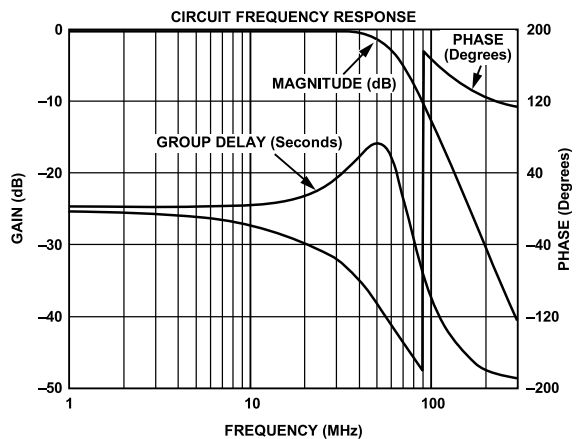
Figure 94. Output Filter Plot for HD, 4× Oversampling
