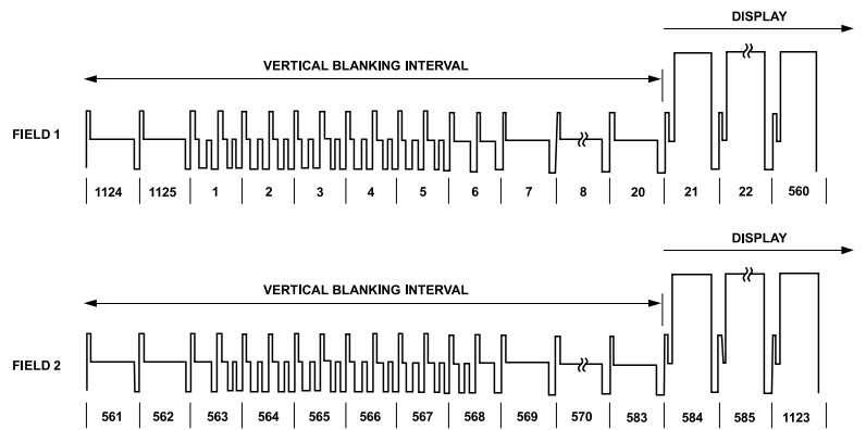
Figure 145. SMPTE 274M (1080i)
