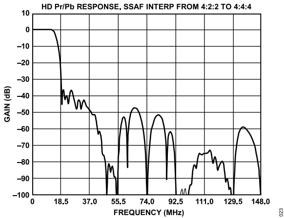
Figure 27. HD 4× Oversampling, PrPb (SSAF) Filter Response (4:2:2 Input)
