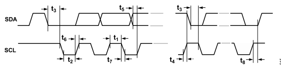
Figure 17. MPU Port Timing Diagram (I 2 C Mode)
