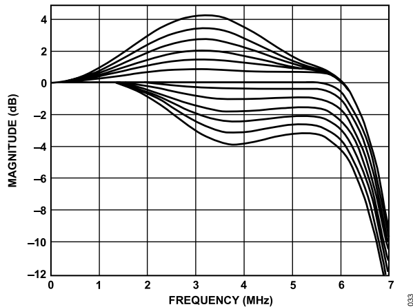
Figure 37. SD Luma SSAF Filter, Programmable Responses
