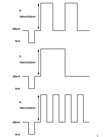
Figure 131. SD/ED RGB Output Levels—RGB Sync Enabled
