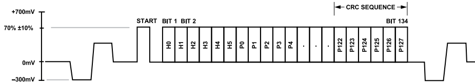
Figure 102. Enhanced Definition (525p) CGMS Type B Waveform
