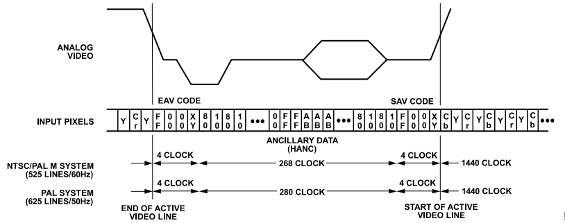
Figure 106. SD Timing Mode 0, Subordinate Option
