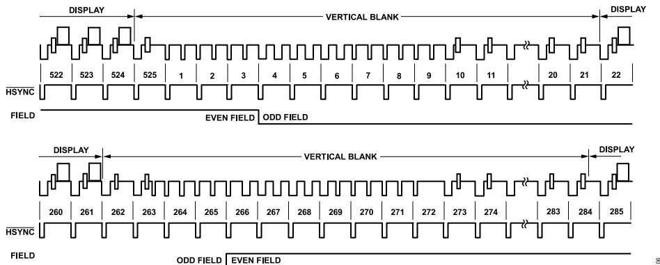
Figure 110. SD Timing Mode 1, Subordinate Option, NTSC
