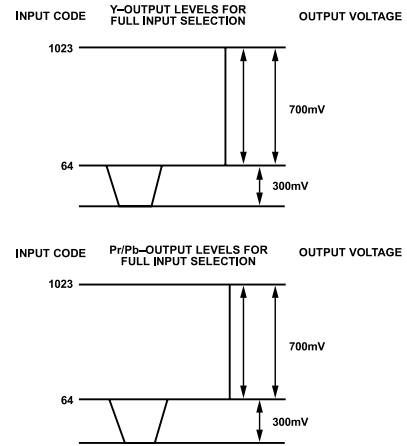
Figure 129. Output Levels for Full Input Selection
