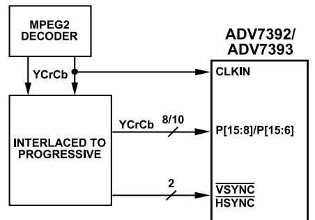
Figure 62. ED/HD-DDR Example Application
