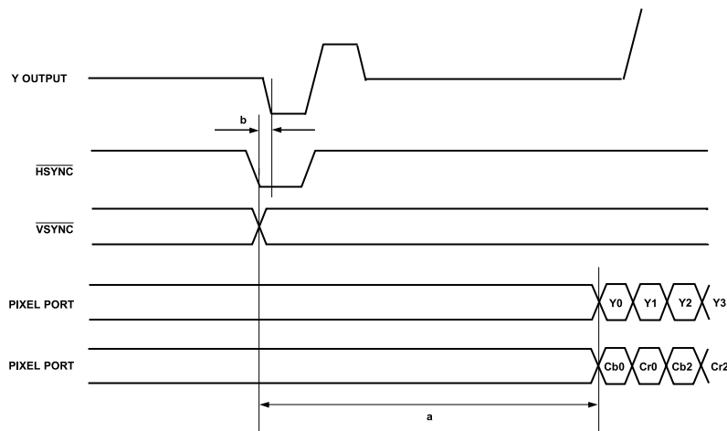
Figure 13. ED-DDR, 8-/10-Bit 4:2:2 YCrCb (HSYNC/VSYNC) Input Timing Diagram
