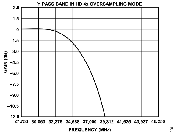
Figure 30. HD 4x Oversampling, Y Filter Response (Focus on Pass Band)
