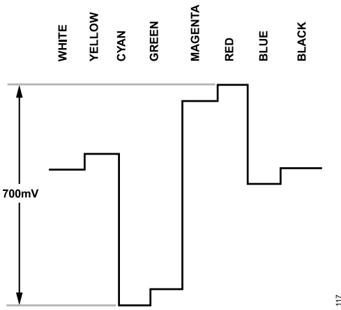
Figure 121. Pr Levels—NTSC
