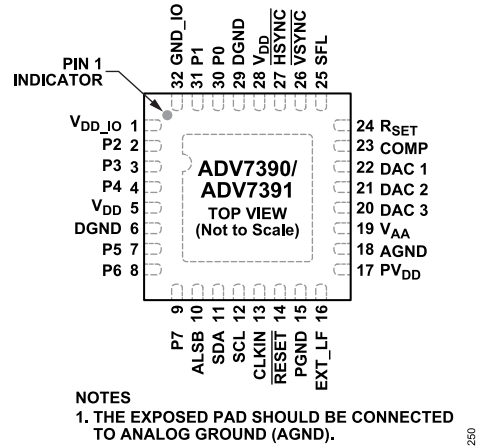
Figure 20. ADV7390/ADV7391 Pin Configuration (CP-32-13)
