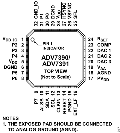
Figure 18. ADV7390/ADV7391 Pin Configuration (CP-32-3)
