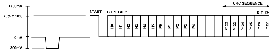
Figure 102. Enhanced Definition (525p) CGMS Type B Waveform
