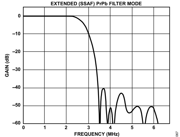
Figure 68. PrPb SSAF Filter
