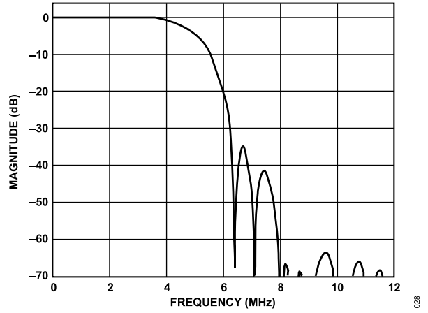
Figure 32. SD PAL, Luma Low-Pass Filter Response
