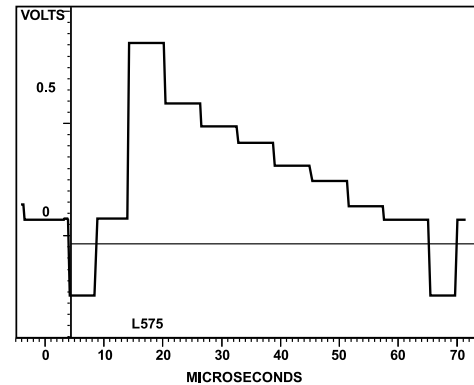
Figure 137. PAL Color Bars (75%)
