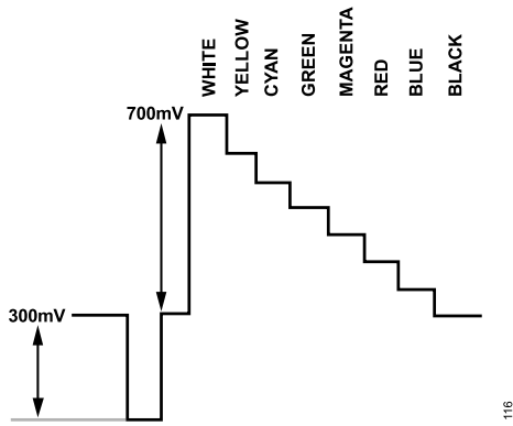
Figure 120. Y Levels—NTSC
