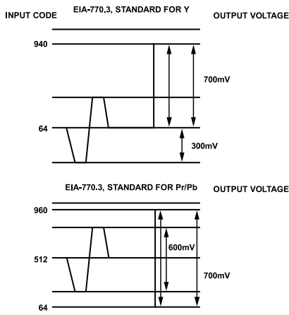
Figure 128. EIA-770.3 Standard Output Signals (1080i/720p)
