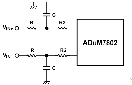
Figure 33. RC Low-Pass Filter Input Network
