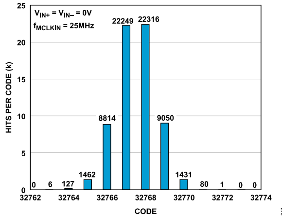
Figure 11. Histogram of Codes at the Code Center
