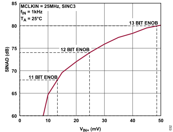
Figure 32. SINAD vs. V_{IN+} AC Input Signal Amplitude
