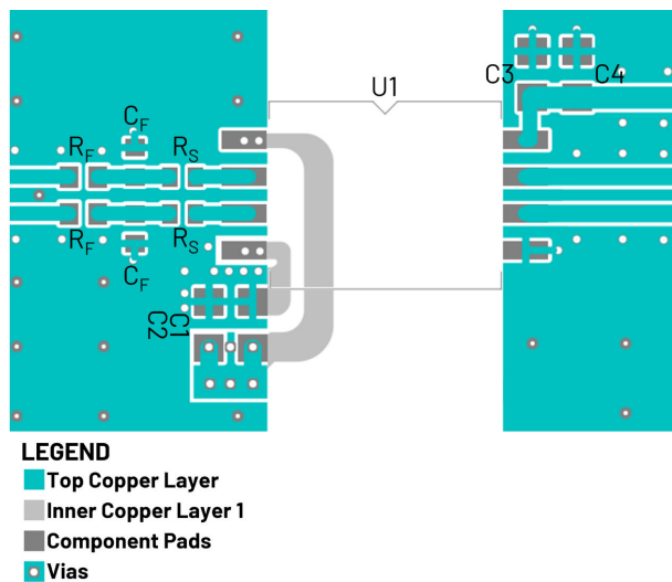
Figure 35. Recommended Layout of the ADuM7802
