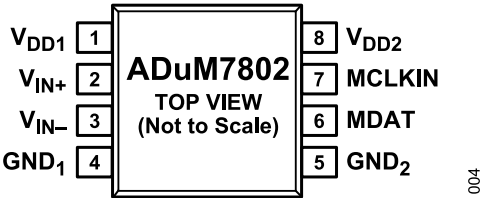
Figure 4. ADuM7802, Pin Configuration
