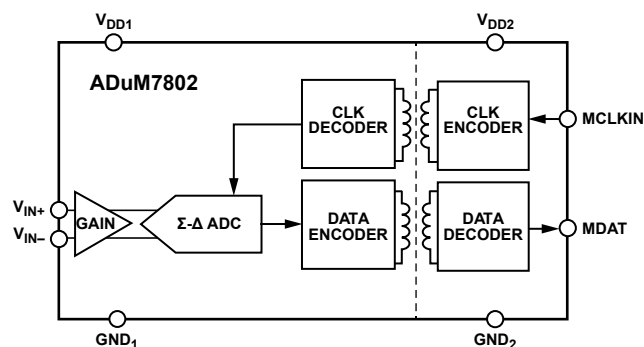
Figure 1. ADuM7802 Functional Block Diagram
