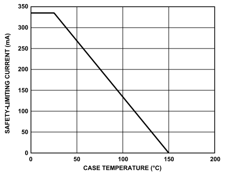
Figure 4. Thermal Derating Curve, Dependence of Safety-Limiting Values with Case Temperature per DIN V VDE V 0884-17
