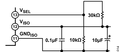
Figure 17. V_{ISO} Bias and Bypass Components
