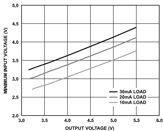
Figure 13. Relationship Between Output Voltage and Required Input Voltage, Under Load, to Maintain >80% Duty Factor in the PWM
