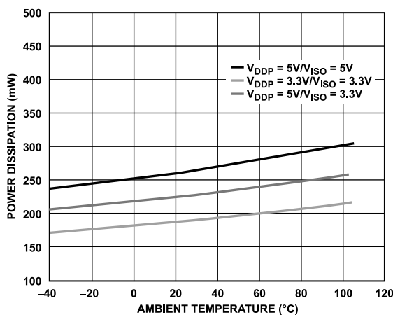
Figure 15. Power Dissipation with a 20 mA Load vs. Temperature
