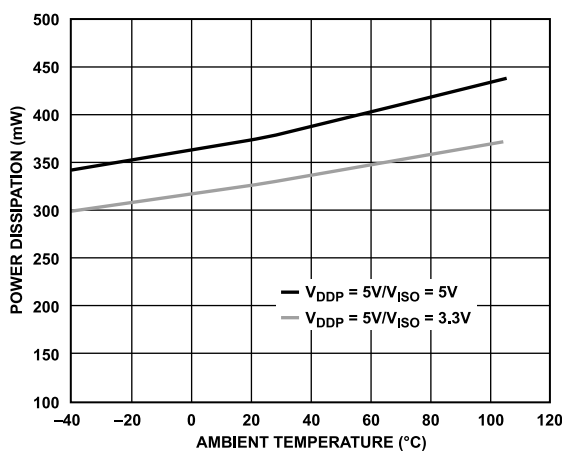
Figure 14. Power Dissipation with a 30 mA Load vs. Temperature
