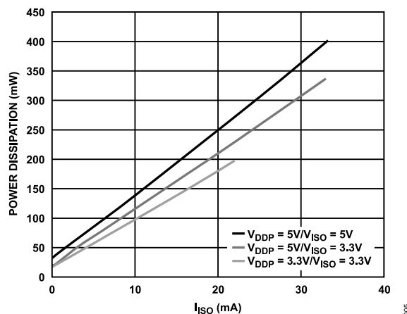
Figure 5. Typical Total Power Dissipation vs. I_{ISO}
