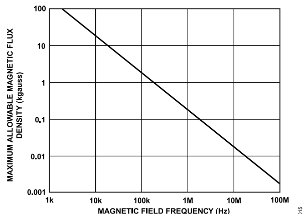
Figure 15. Maximum Allowable External Magnetic Flux Density
