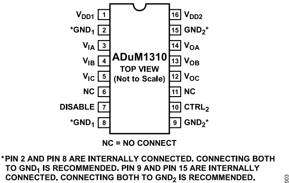
Figure 4. ADuM1310 Pin Configuration
