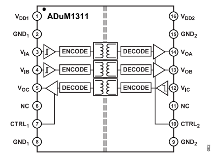
Figure 2. ADuM1311
