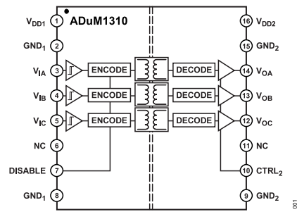
Figure 1. ADuM1310
