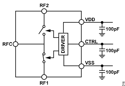
Figure 16. Recommended Schematic
