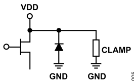
Figure 5. VDD Interface Schematic
