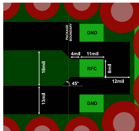
Figure 19. Recommended RF Pin Transition
