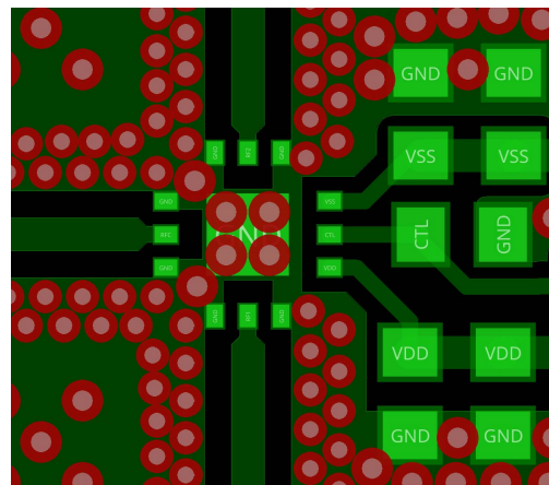
Figure 18. PCB Layout
