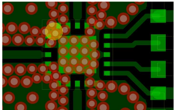
Figure 20. PCB Routings
