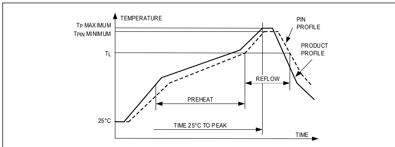
Figure 10. Recommended Reflow Profile
