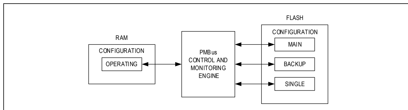
Figure 8. Configuration Data Management
