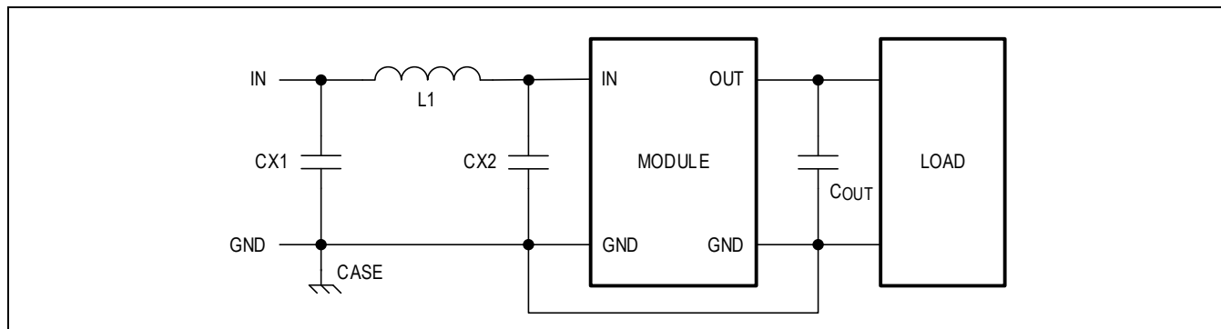
Figure 4. EMC Testing Typical Application Circuit
