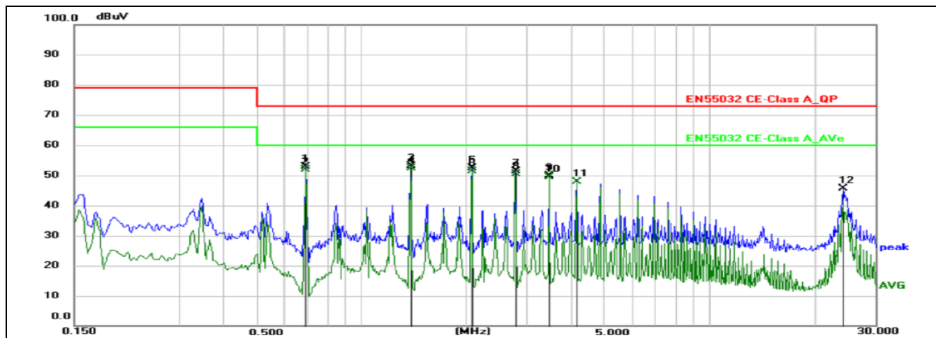
Figure 5. EMC Test Result ( V_{IN} = 54V , I_{OUT} = 133.3A )
