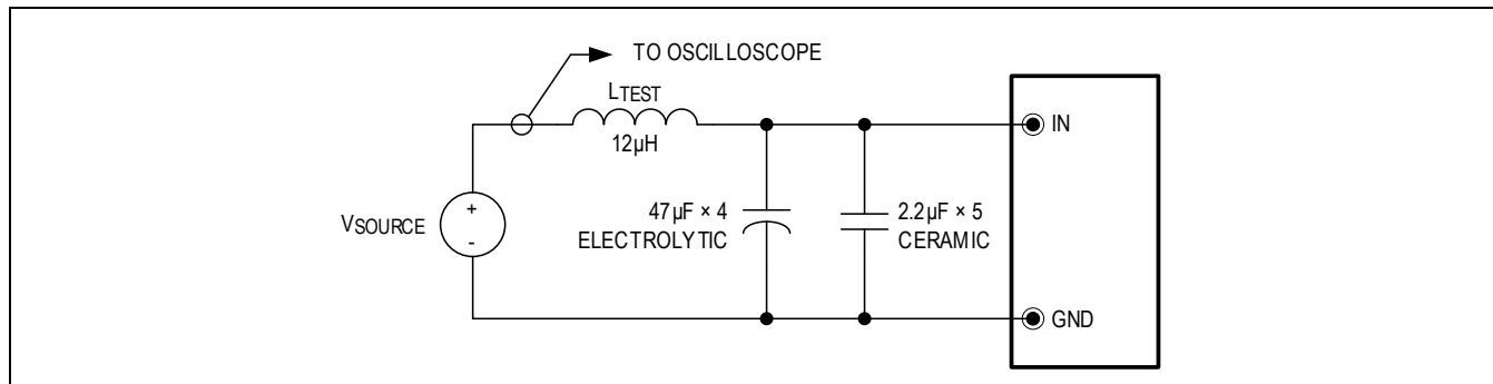
Figure 1. Input Reflected Ripple Current Test Setup
