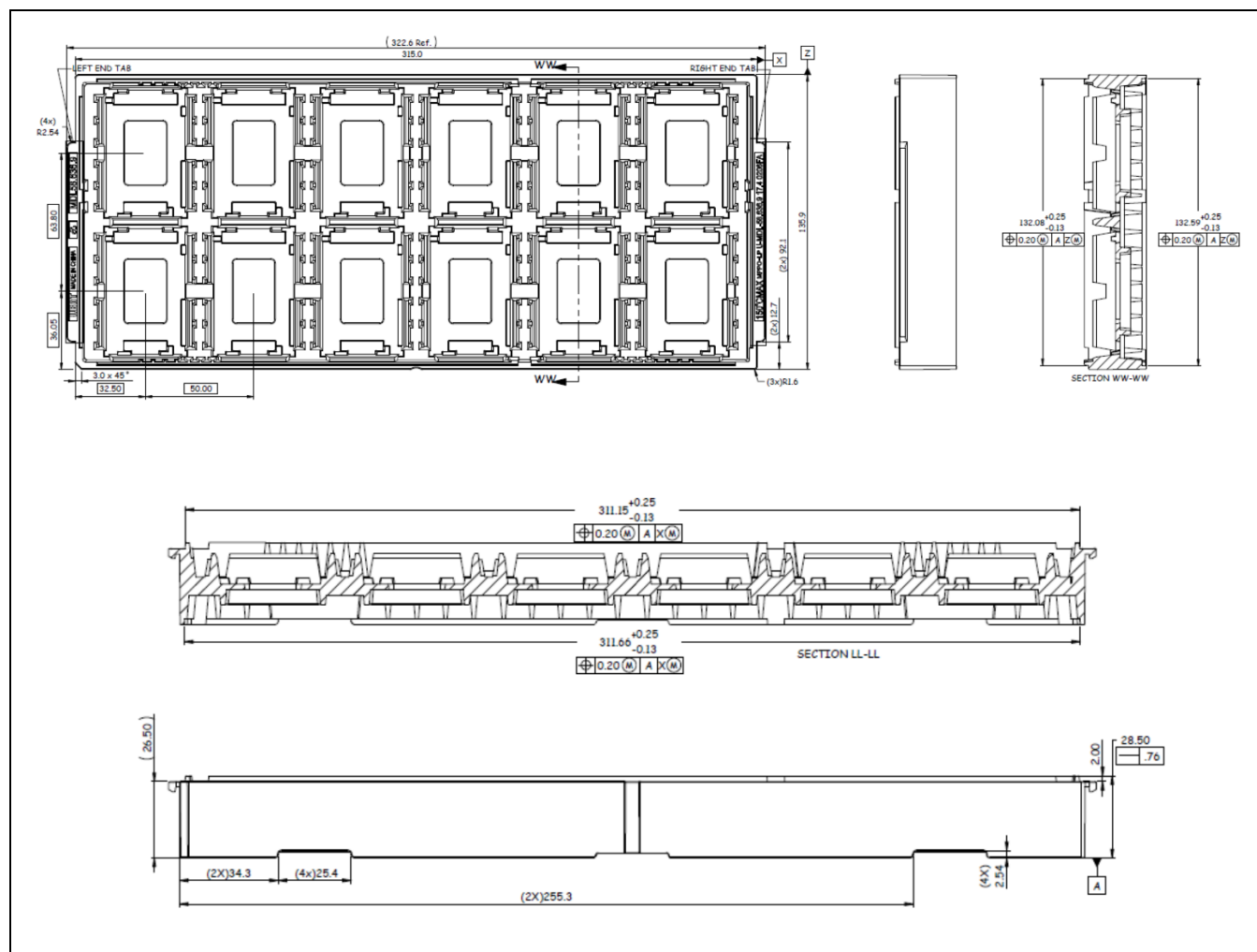
Figure 11. Packaging Tray Diagram
