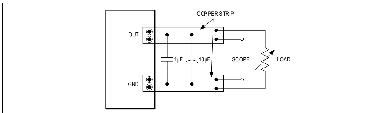
Figure 2. Output Ripple and Noise Test Setup
