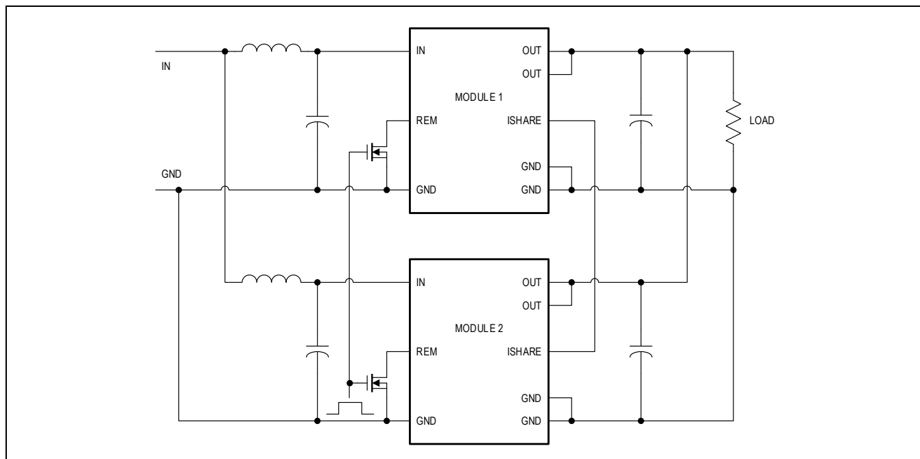
Figure 3. Active Current-Sharing Diagram with Two Modules
