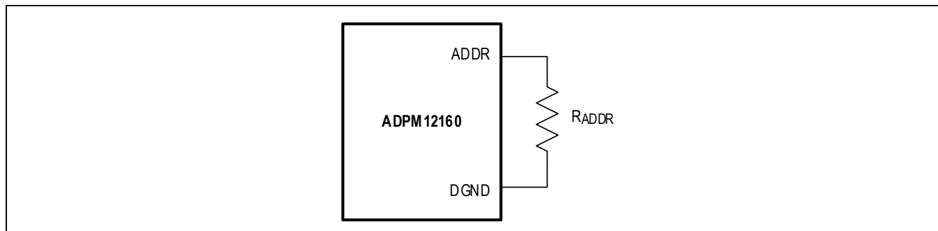
Figure 7. PMBus Address Select
