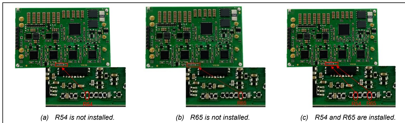
Figure 6. Configuration of the Calibration Resistors
