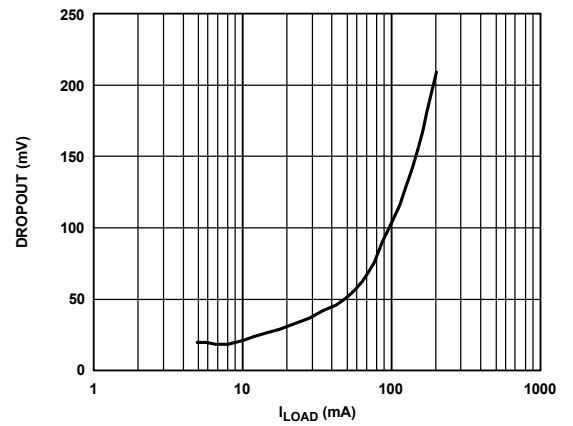
Figure 10. Dropout Voltage ( V_{DROPOUT} ) vs. Load Current ( I_{LOAD} ), V_{OUT} = 5V
