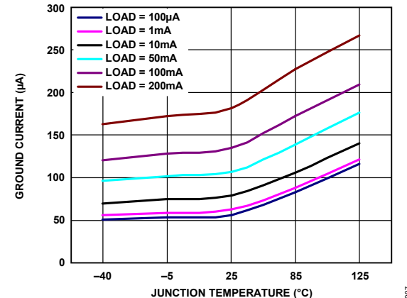
Figure 8. Ground Current ( I_{GND} ) vs. Junction Temperature ( T_J )
