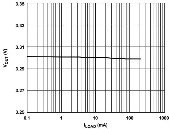
Figure 13. Output Voltage ( V_{OUT} ) vs. Load Current ( I_{LOAD} ), V_{OUT} = 3.3V
