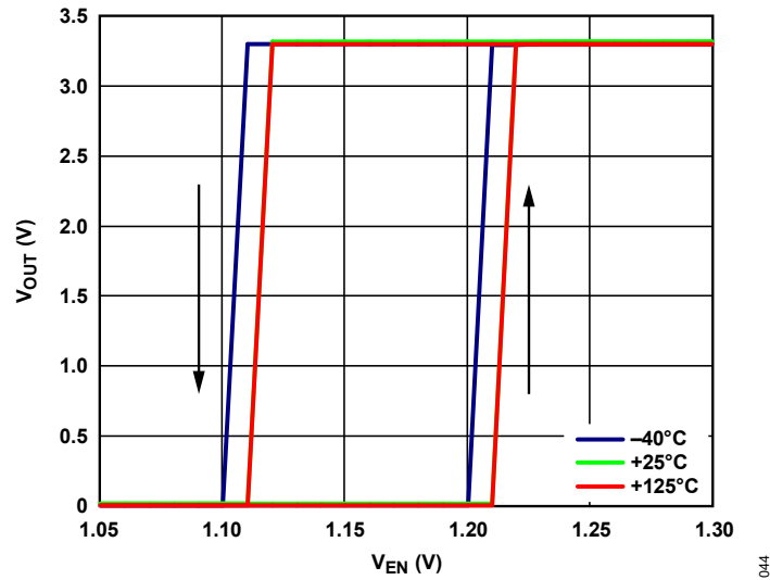
Figure 28. Typical V OUT Response to EN Pin Operation
