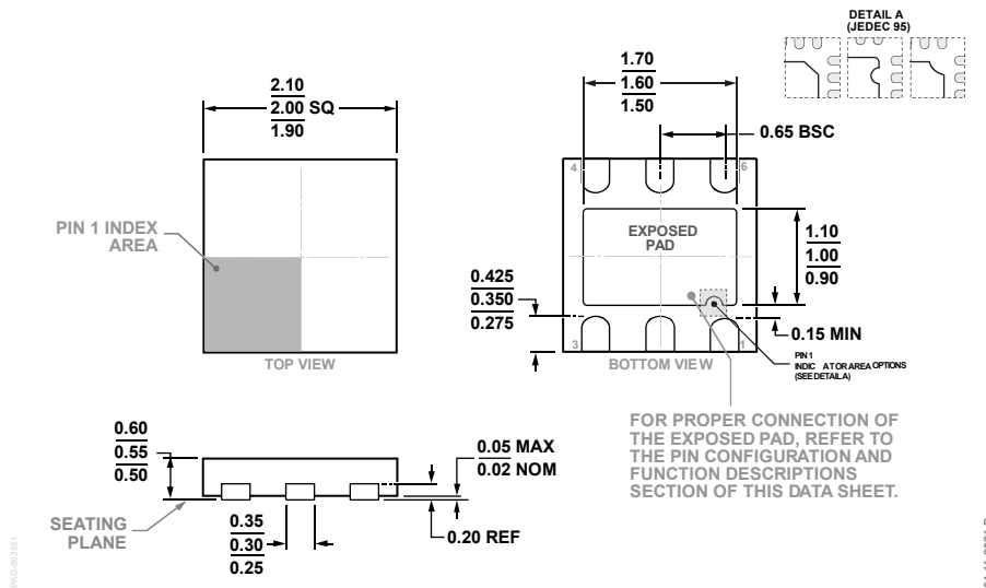
Figure 35. 6-Lead Lead Frame Chip Scale Package [LFCSP] 2.00mm × 2.00mm Body and 0.55mm Package Height (CP-6-3) Dimensions shown in millimeters
