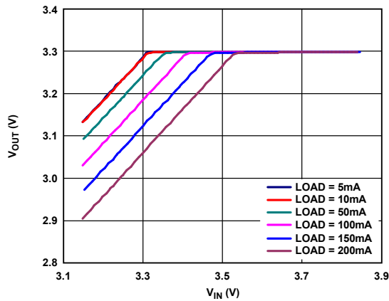
Figure 17. Output Voltage ( V_{OUT} ) vs. Input Voltage ( V_{IN} ) in Dropout, V_{OUT} = 3.3V
