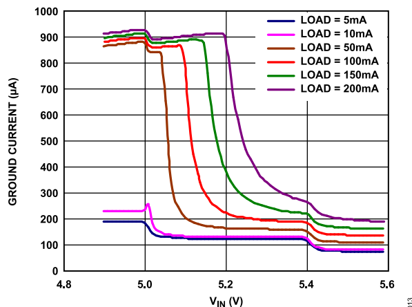
Figure 15. Ground Current ( I_{GND} ) vs. Input Voltage ( V_{IN} ) in Dropout, V_{OUT} = 5 V
