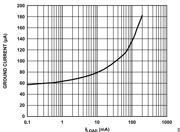
Figure 10. Ground Current ( I_{GND} ) vs. Load Current ( I_{LOAD} )
