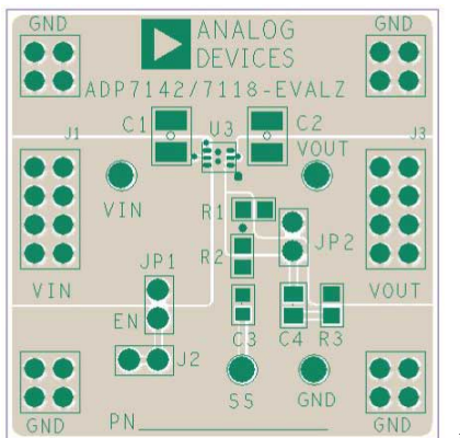
Figure 64. Example LFCSP PCB Layout
