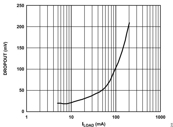
Figure 13. Dropout Voltage ( V_{DROP-OUT} ) vs. Load Current ( I_{LOAD} ), V_{OUT} = 5 V
