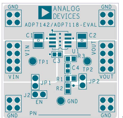
Figure 65. Example SOIC PCB Layout
