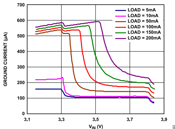
Figure 24. Ground Current ( I_{GND} ) vs. Input Voltage ( V_{IN} ) in Dropout, V_{OUT} = 3.3\text{ V}
