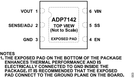
Figure 3. 6-Lead LFCSP Pin Configuration
