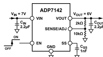
Figure 2. ADP7142 with 5 V Output Adjusted to 6 V
