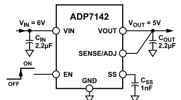
Figure 1. ADP7142 with Fixed Output Voltage, 5 V
