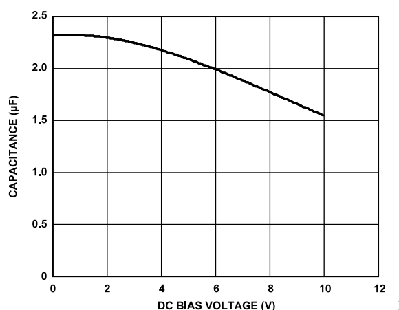
Figure 45. Capacitance vs. Voltage Characteristic
