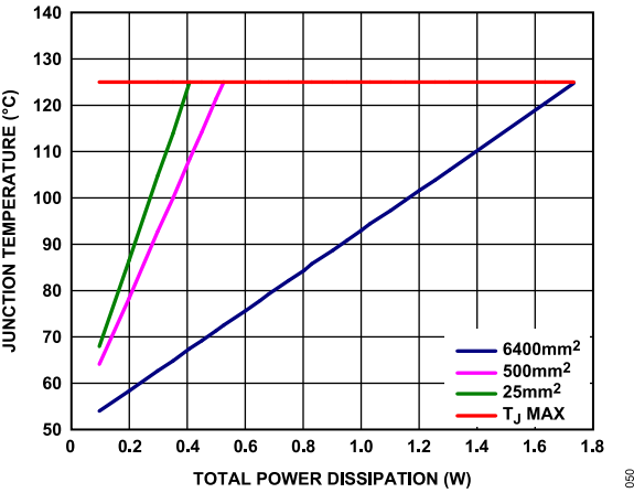
Figure 53. LFCSP, T_A = 50^\circ\text{C}
