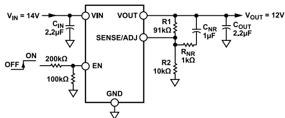
Figure 50. Noise Reduction Modification
