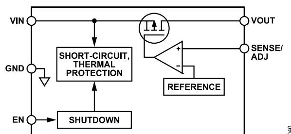
Figure 42. Internal Block Diagram
