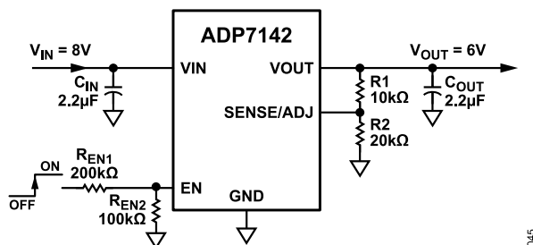
Figure 47. Typical EN Pin Voltage Divider
