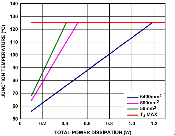
Figure 56. SOIC, T_A = 50^\circ\text{C}
