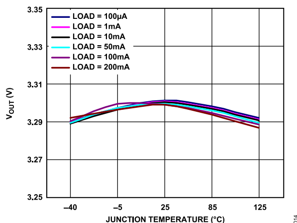
Figure 16. Output Voltage ( V_{OUT} ) vs. Junction Temperature ( T_J ), V_{OUT} = 3.3 V
