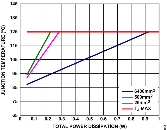
Figure 54. LFCSP, T_A = 85^\circ\text{C}
