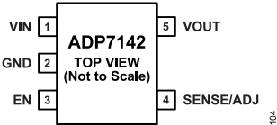
Figure 4. 5-Lead TSOT Pin Configuration
