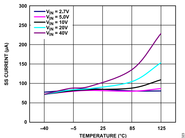
Figure 25. Soft Start (SS) Current vs. Temperature ( T_J ), Multiple Input Voltages ( V_{IN} ), V_{OUT} = 5\text{ V}
