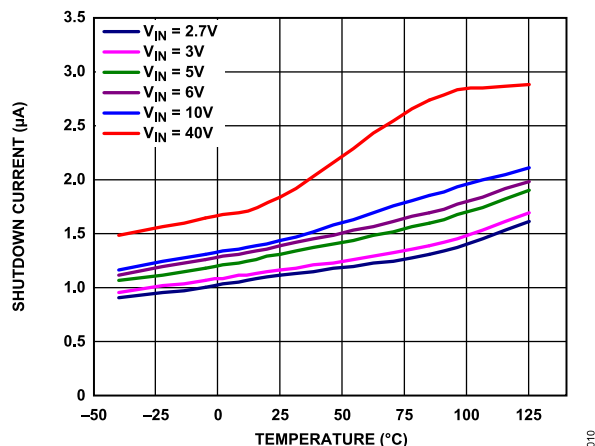
Figure 12. Shutdown Current ( I_{GND-SD} ) vs. Temperature at Various Input Voltages ( V_{IN} )
