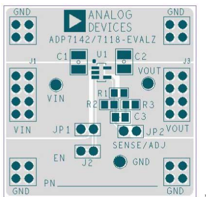
Figure 66. Example TSOT PCB Layout
