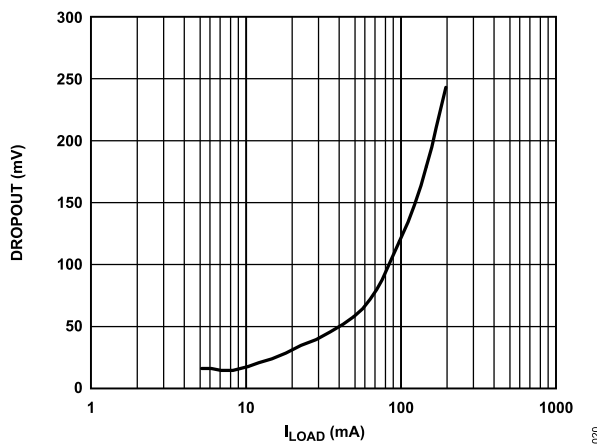
Figure 22. Dropout Voltage ( V_{DROP} ) vs. Load Current ( I_{LOAD} ), V_{OUT} = 3.3\text{ V}
