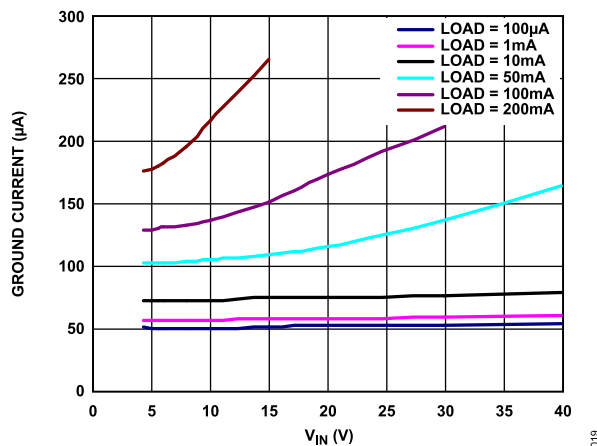
Figure 21. Ground Current ( I_{GND} ) vs. Input Voltage ( V_{IN} ), V_{OUT} = 3.3\text{ V}
