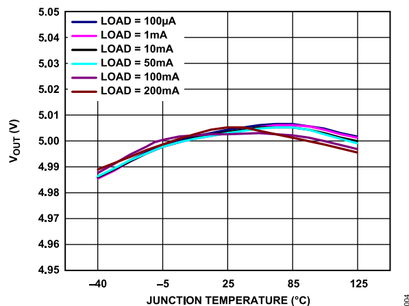
Figure 6. Output Voltage ( V_{OUT} ) vs. Junction Temperature ( T_J )
