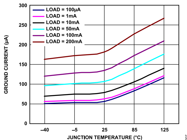
Figure 9. Ground Current ( I_{GND} ) vs. Junction Temperature ( T_J )
