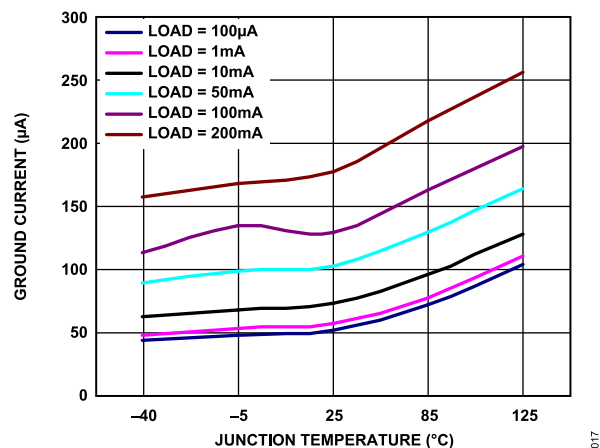
Figure 19. Ground Current ( I_{GND} ) vs. Junction Temperature ( T_J ), V_{OUT} = 3.3\text{ V}
