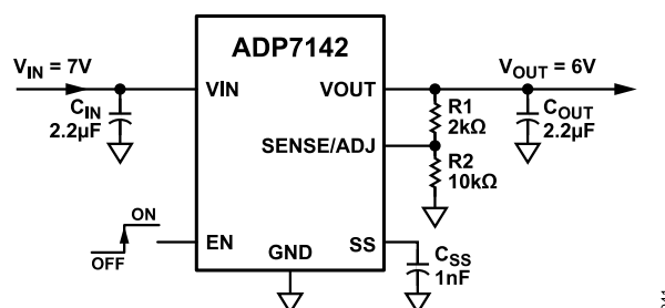
Figure 43. Typical Adjustable Output Voltage Application Schematic
