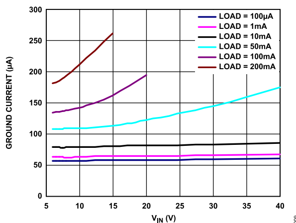
Figure 11. Ground Current ( I_{GND} ) vs. Input Voltage ( V_{IN} )
