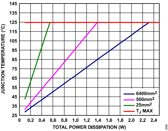
Figure 52. LFCSP, T_A = 25^\circ\text{C}
