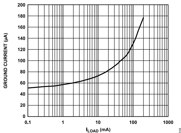
Figure 20. Ground Current ( I_{GND} ) vs. Load Current ( I_{LOAD} ), V_{OUT} = 3.3\text{ V}
