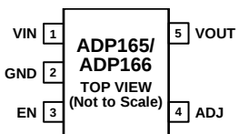
Figure 5. 5-Lead TSOT, Adjustable Output Pin Configuration
