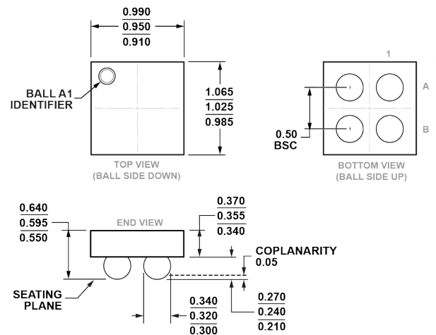
Figure 62. 4-Ball Wafer Level Chip Scale Package [WLCSP] (CB-4-4)
