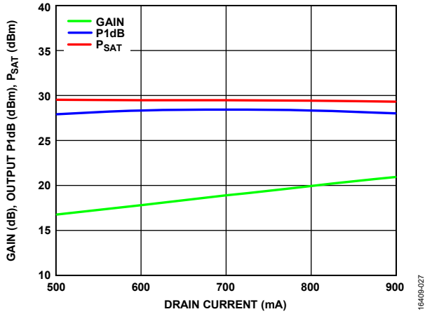
Figure 27. Gain, Output P1dB, and P_{SAT} vs. I_{DD} , RF = 86 GHz
