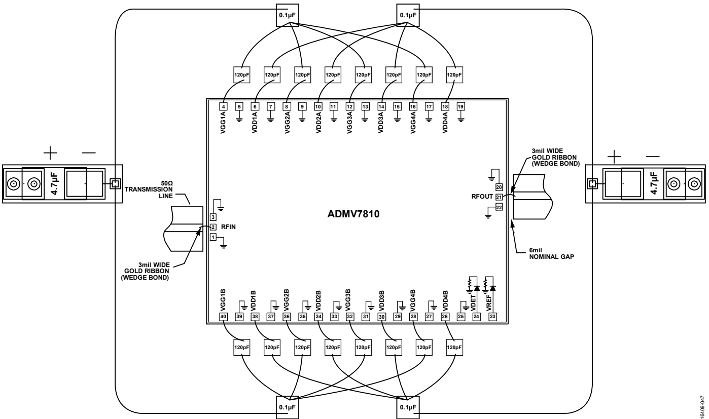
Figure 48. Assembly Diagram
