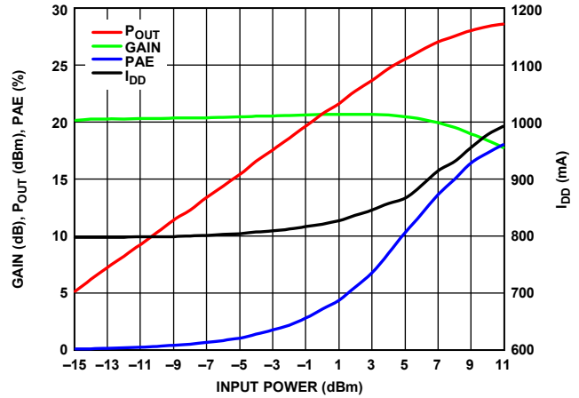
Figure 31. Gain, P_{OUT} , PAE, and I_{DD} vs. Input Power, RF = 81 GHz, I_{DD} = 800 mA
