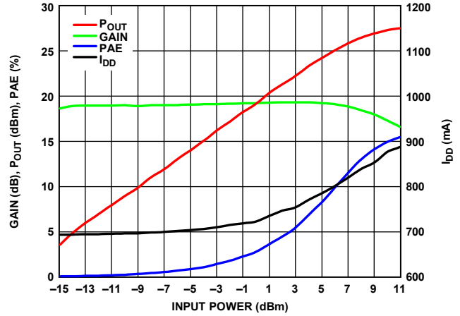
Figure 30. Gain, P_{OUT} , PAE, and I_{DD} vs. Input Power, RF = 86 GHz, I_{DD} = 700 mA
