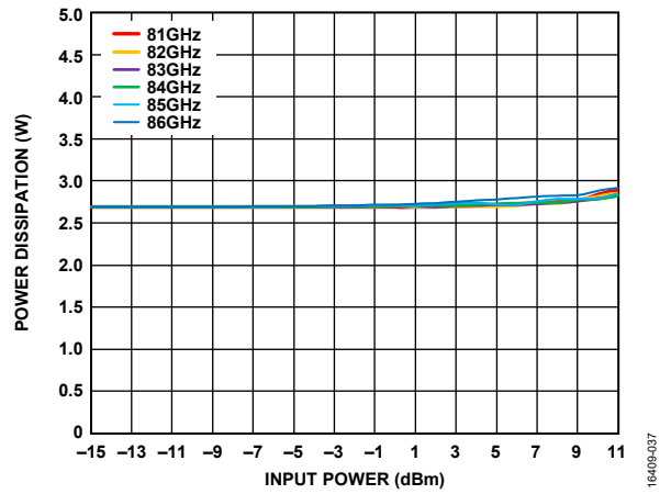
Figure 37. Power Dissipation vs. Input Power over Various Frequencies, I_{DD} = 700 mA, T_A = 85°C
