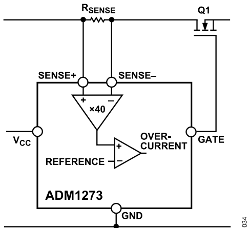
Figure 34. Hot-Swap Current Sense Amplifier
