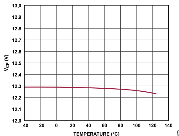
Figure 25. V_{CP} Voltage vs. Temperature
