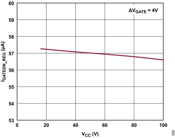
Figure 9. GATE Regulation Pull-Down Current ( I_{GATEDN\_REG} ) vs. V_{CC}
