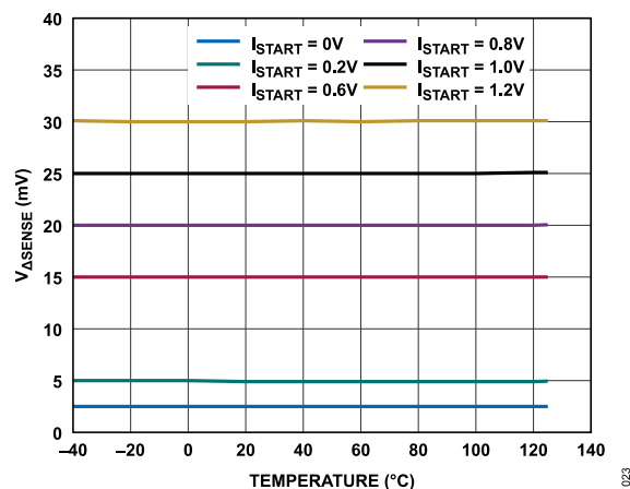
Figure 23. V_{\Delta SENSE} vs. Temperature, V_{ISTART} with 1Ω Sense Resistor
