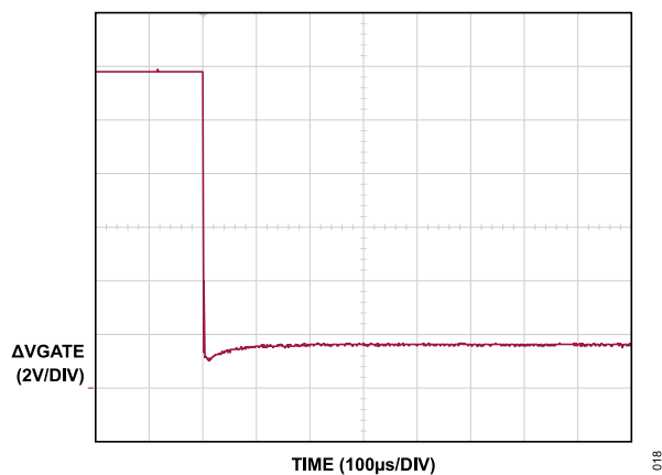
Figure 18. \Delta V_{GATE} Response to Severe Overcurrent Event (GATE Fast Pull-Down)
