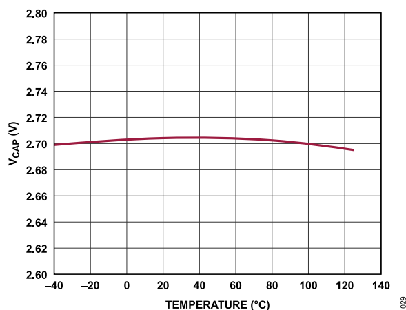
Figure 29. VCAP Voltage vs. Temperature
