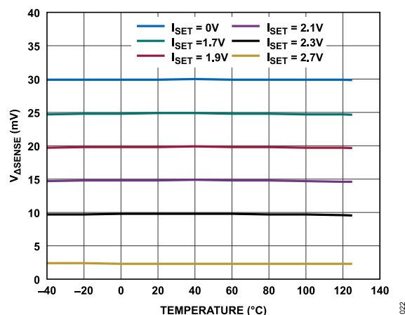
Figure 22. V_{\Delta SENSE} vs. Temperature, V_{ISET} with 1Ω Sense Resistor
