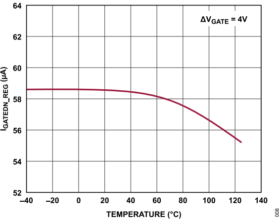
Figure 8. GATE Regulation Pull-Down Current ( I_{GATEDN\_REG} ) vs. Temperature
