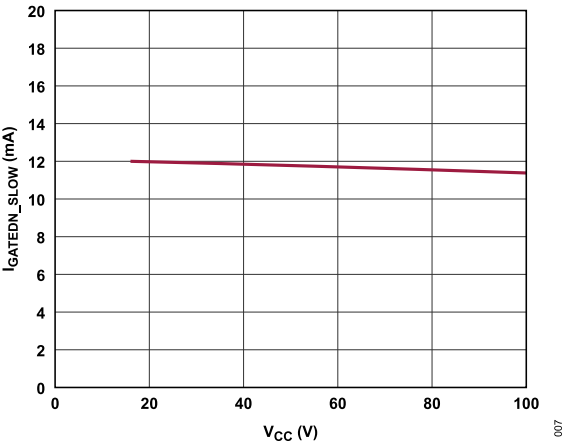
Figure 7. GATE Slow Pull-Down Current ( I_{GATEDN\_SLOW} ) vs. V_{CC}
