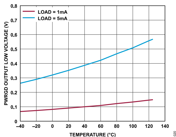
Figure 20. PWRGD Output Low Voltage ( V_{OL\_PWRGD} ) vs. Temperature
