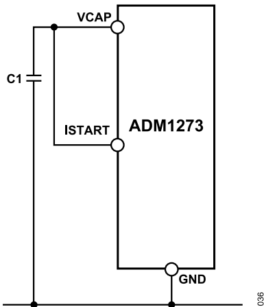
Figure 36. Fixed 25mV ISTART Current Sense Limit
