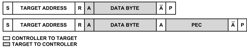
Figure 44. Receive Byte and Receive Byte with PEC
