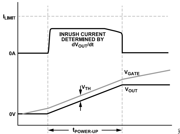
Figure 40. Linear Voltage Ramp Power-Up
