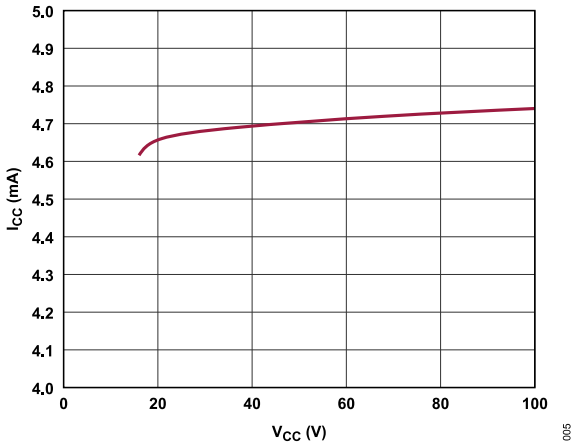
Figure 5. Supply Current ( I_{CC} ) vs. V_{CC}
