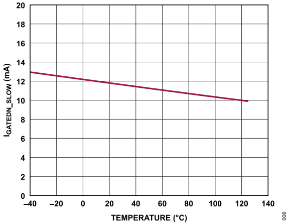
Figure 6. GATE Slow Pull-Down Current ( I_{GATEDN\_SLOW} ) vs. Temperature
