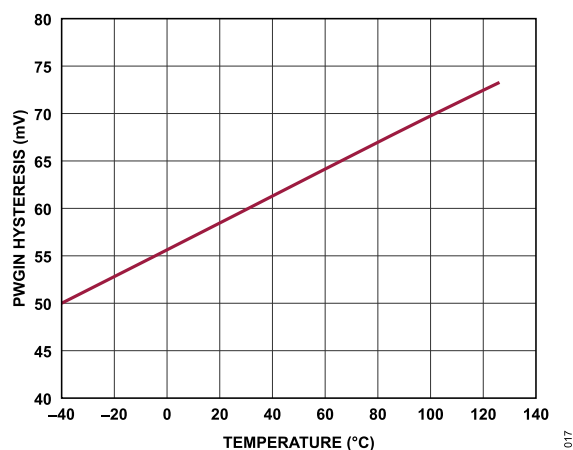
Figure 17. PWGIN Threshold Hysteresis vs. Temperature
