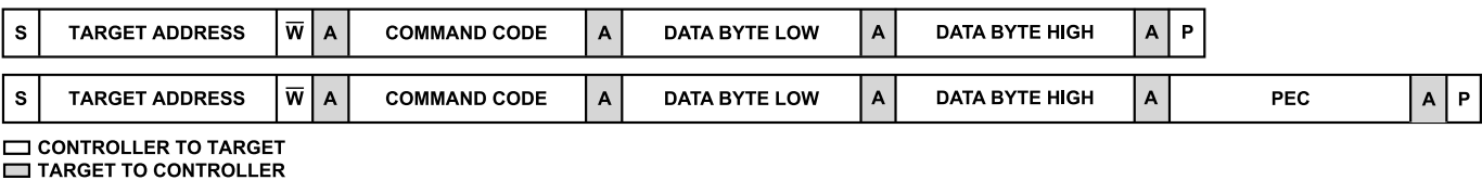
Figure 47. Write Word and Write Word with PEC
