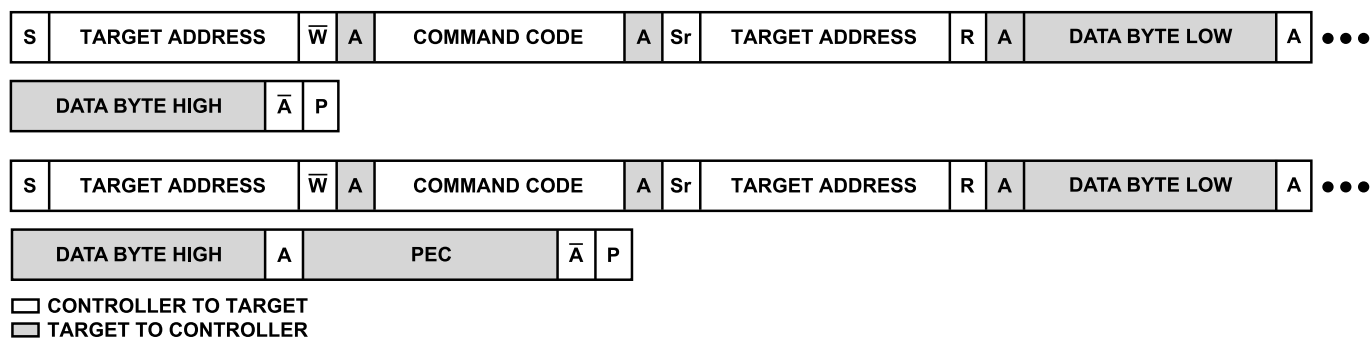
Figure 48. Read Word and Read Word with PEC
