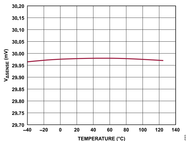
Figure 32. VASENSE vs. Temperature at ISET = 0
