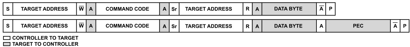
Figure 46. Read Byte and Read Byte with PEC
