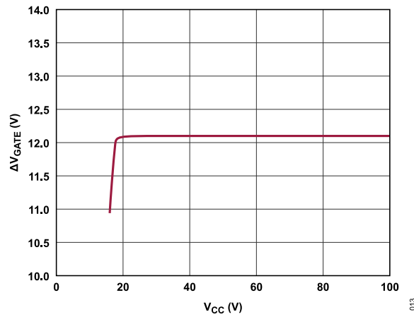
Figure 13. \Delta V_{GATE} (5 \mu A Load) vs. V_{CC}
