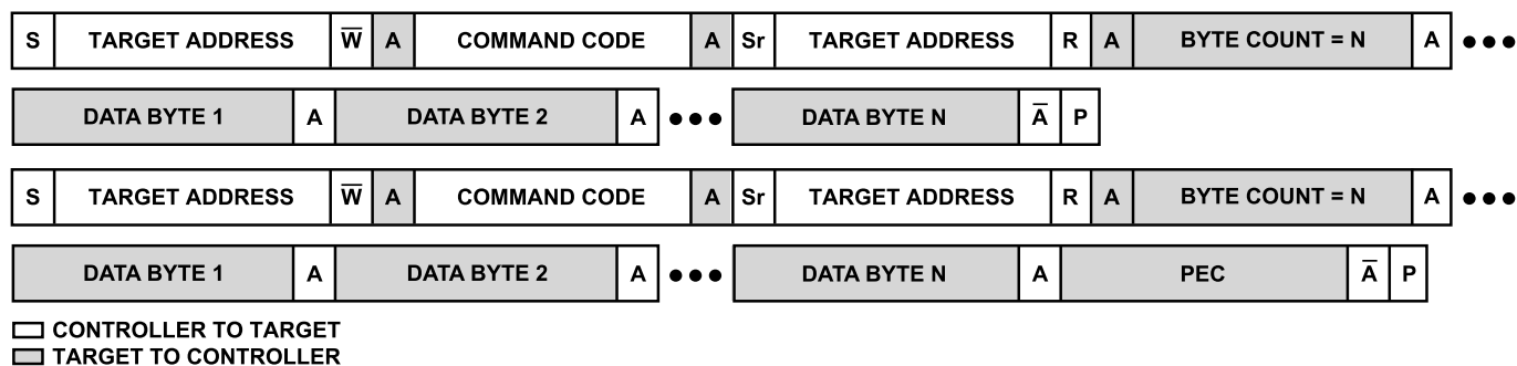
Figure 49. Block Read and Block Read with PEC
