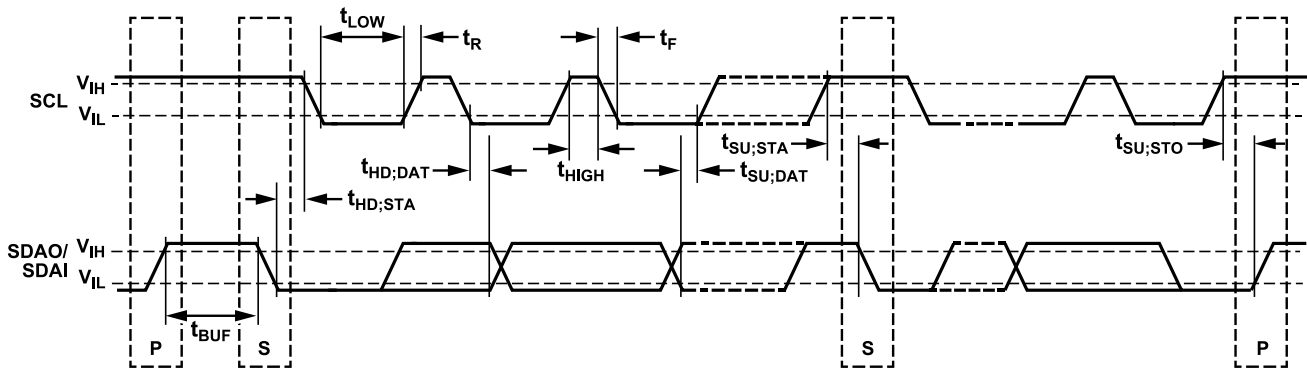
Figure 2. Serial Bus Timing Diagram
