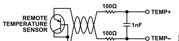
Figure 42. Filter Between Remote Sensor and ADM1273
