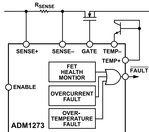
Figure 41. \overline{\text{FAULT}} Pin Operation
