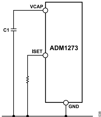
Figure 38. Fixed 30mV ISET Current Sense Limit
