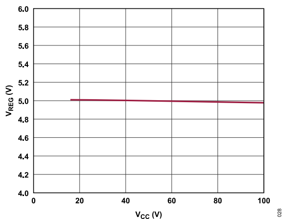
Figure 28. VREG Voltage vs. VCC
