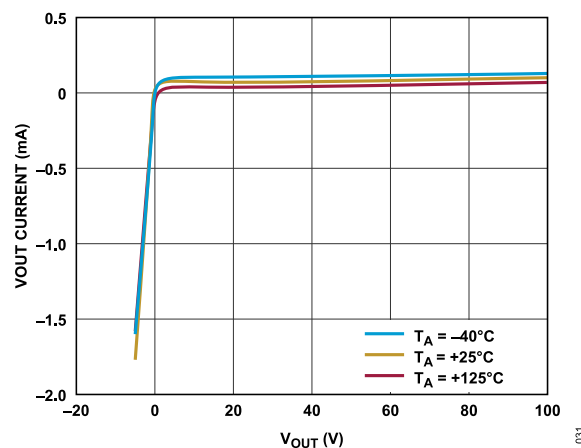
Figure 31. VOUT Current vs. Voltage
