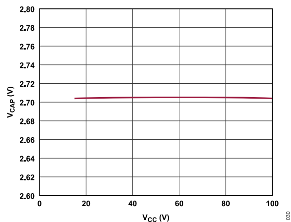
Figure 30. VCAP Voltage vs. VCC
