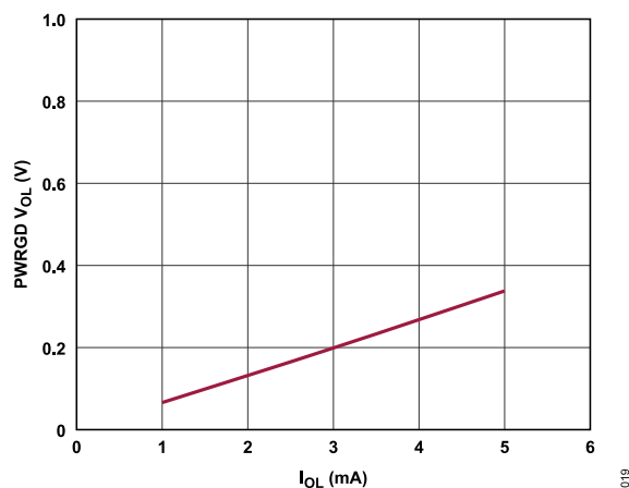
Figure 19. PWRGD Output Low Voltage ( V_{OL\_PWRGD} ) vs. I_{OL}
