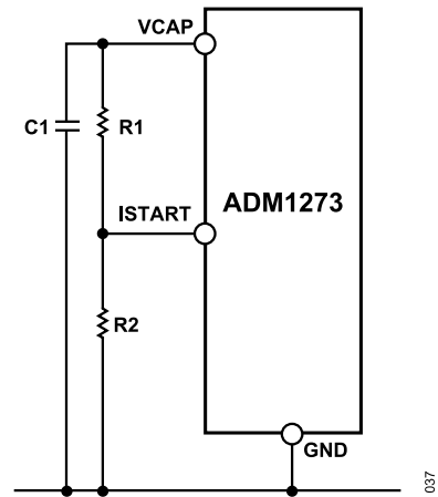
Figure 37. Adjustable 5mV to 30mV Current Sense Limit
