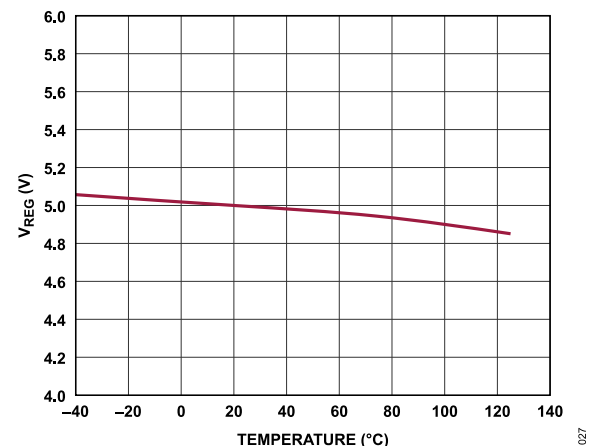
Figure 27. V_{REG} Voltage vs. Temperature
