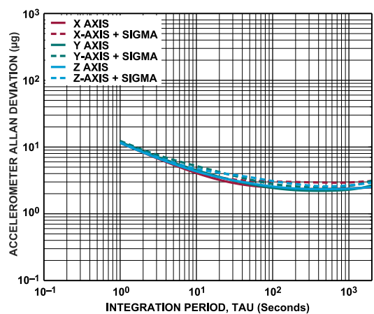
Figure 18. Accelerometer Allan Deviation ADIS16545
