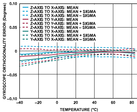
Figure 12. Gyroscope Orthogonality Error vs. Temperature
