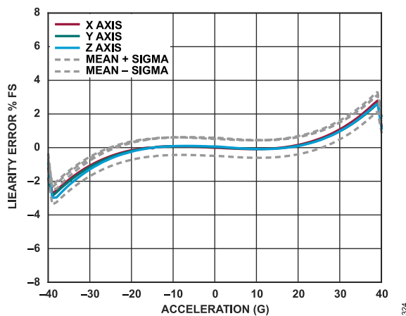
Figure 24. Accelerometer Linearity Error vs. Acceleration, ADIS16547
