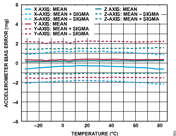
Figure 25. Accelerometer Bias Error vs. Temperature, ADIS16547
