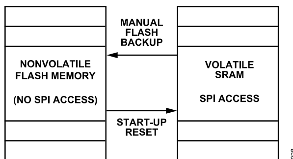
Figure 42. SRAM and Flash Memory Diagram
