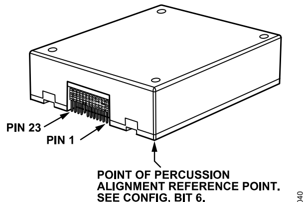
Figure 54. Point of Percussion Reference Point
