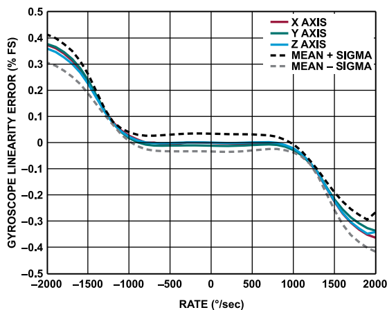
Figure 17. Gyroscope Linearity Error vs. Rate, ADIS16545-3 and ADIS16547-3
