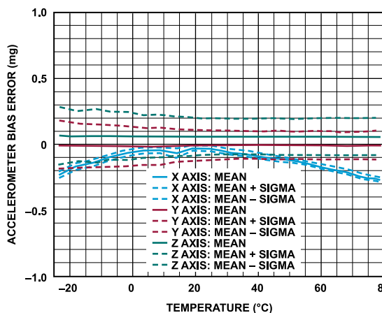
Figure 19. Accelerometer Bias Error vs. Temperature, ADIS16545
