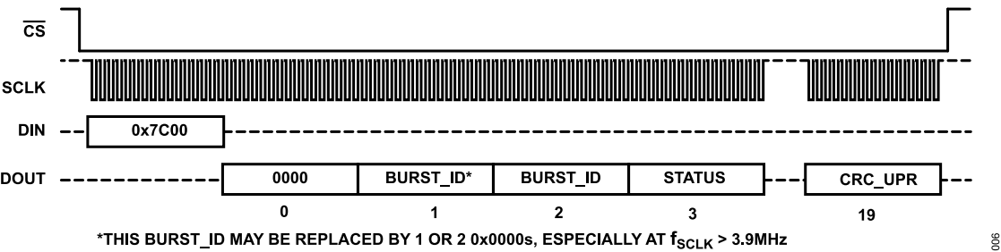
Figure 6. Burst Read Function Sequence Diagram
