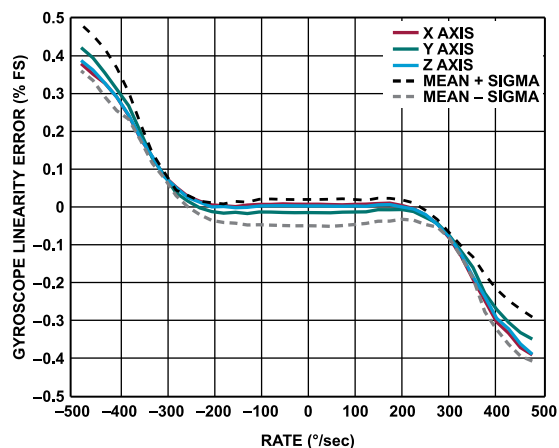
Figure 16. Gyroscope Linearity Error vs. Rate, ADIS16545-2 and ADIS16547-2
