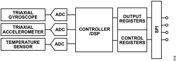
Figure 33. Basic Operation
