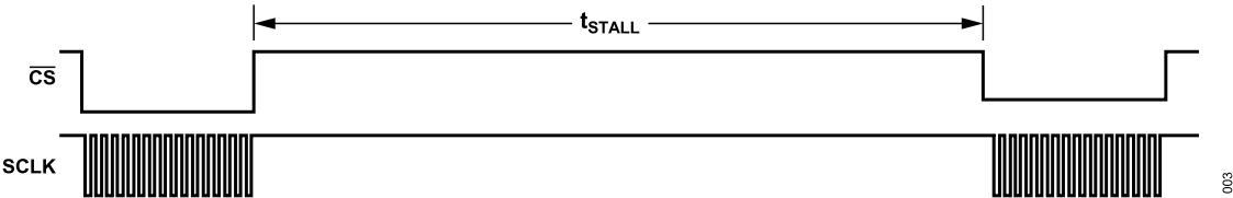
Figure 3. Stall Time and Data Rate
