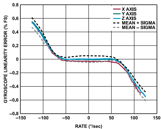
Figure 15. Gyroscope Linearity Error vs. Rate, ADIS16545-1 and ADIS16547-1
