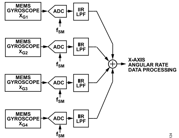
Figure 29. Gyroscope Data Sampling
