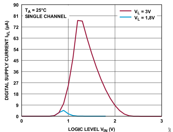
Figure 47. Digital Supply Current vs. Logic Level
