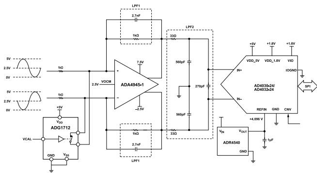
Figure 58. Typical Application
