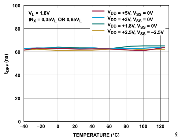
Figure 45. T_{OFF} Times vs. Temperature
