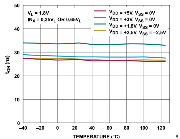
Figure 46. T_{ON} Times vs. Temperature
