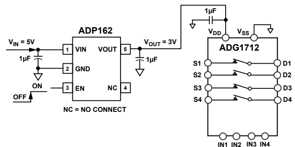
Figure 60. Power Supply Recommendation
