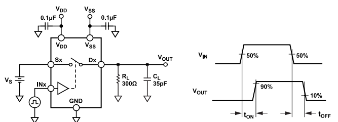
Figure 56. Switching Times
