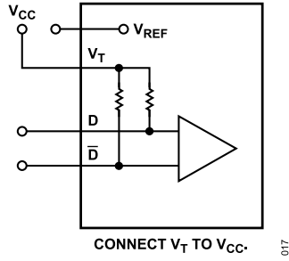
Figure 15. Interfacing to CML Inputs
