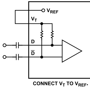
Figure 16. AC Coupling Differential Signals
