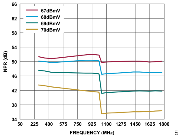
Figure 11. NPR vs. Frequency Over TCP, 10 dB Tilt, V_{DD} = 8.0 V
