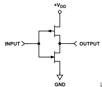
Figure 18. Inverter Circuit
