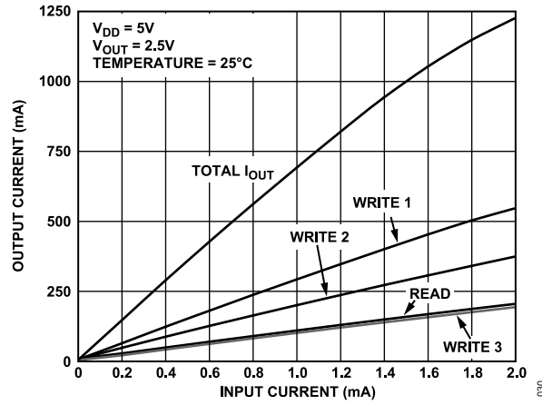
Figure 10. Output Current vs. Input Current for Each Channel, V_{OUT} = 2.5 V
