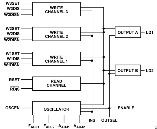
Figure 1. 4-Channel, LVDS, Laser Driver Block Diagram
