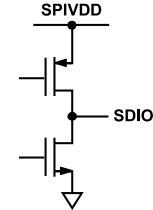
Figure 8. Equivalent SDIO Output Circuit
