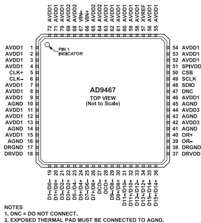
Figure 3. Pin Configuration, Top View
