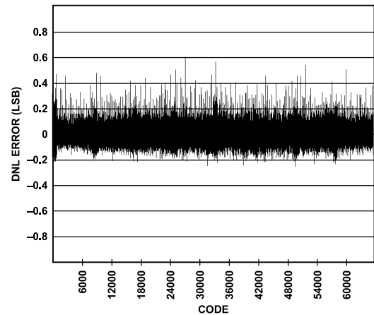
Figure 39. DNL, f_{IN} = 4.3 MHz, 2.5 V p-p FS, AD9467-250
