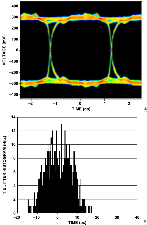
Figure 65. Data Eye for LVDS Outputs in ANSI-644 Mode with 6-Inch Trace Lengths on Standard FR-4, AD9467-250
