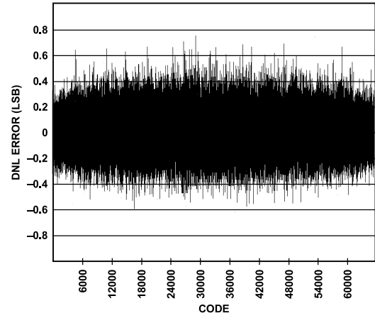
Figure 37. DNL, f_{IN} = 4.3 MHz, 2.5 V p-p FS, AD9467-200
