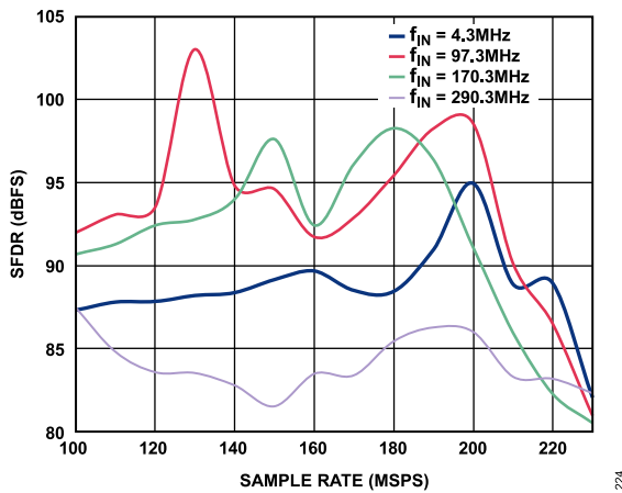
Figure 24. SFDR vs. f_{SAMPLE} , 2.5 V p-p FS, AD9467-200
