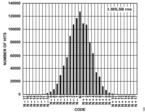
Figure 45. Input-Referred Noise Histogram, 2.5 V p-p FS, AD9467-250
