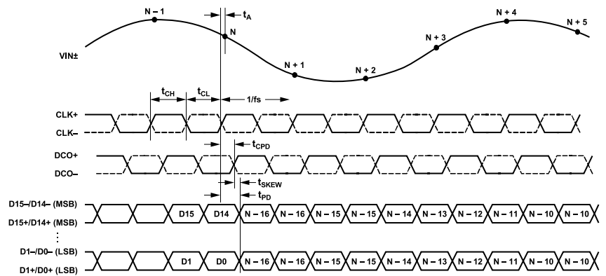
Figure 2. 16-Bit Output Data Timing
