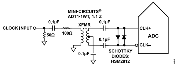
Figure 58. Transformer-Coupled Differential Clock
