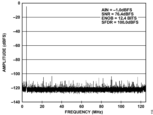
Figure 16. Single-Tone FFT with f_{IN} = 4.3 MHz, 2.5 V p-p FS, AD9467-250
