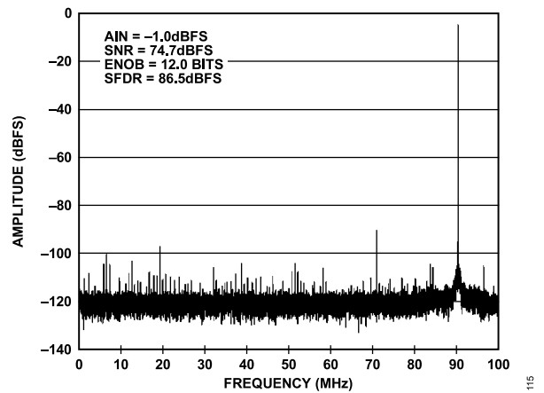
Figure 15. Single-Tone FFT with f_{IN} = 290.3 MHz, 2.5 V p-p FS, AD9467-200
