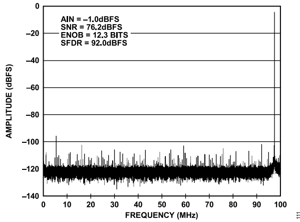
Figure 11. Single-Tone FFT with f_{IN} = 97.3 MHz, 2.5 V p-p FS, AD9467-200
