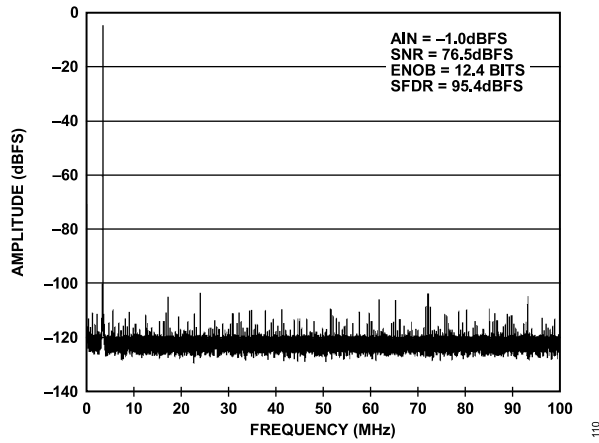
Figure 10. Single-Tone FFT with f_{IN} = 4.3 MHz, 2.5 V p-p FS, AD9467-200
