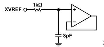
Figure 9. Equivalent External VREF Input Circuit (When Enabled)
