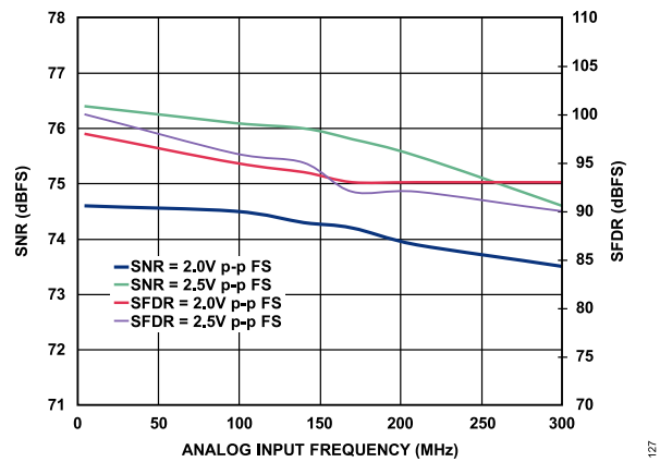
Figure 27. SNR/SFDR vs. f_{IN} , 2.0/2.5 V p-p FS, AD9467-250
