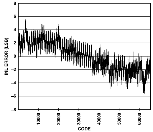
Figure 38. INL, f_{IN} = 4.3 MHz, 2.5 V p-p FS, AD9467-250
