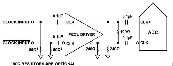
Figure 59. Differential PECL Sample Clock
