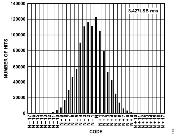
Figure 44. Input-Referred Noise Histogram, 2.5 V p-p FS, AD9467-200
