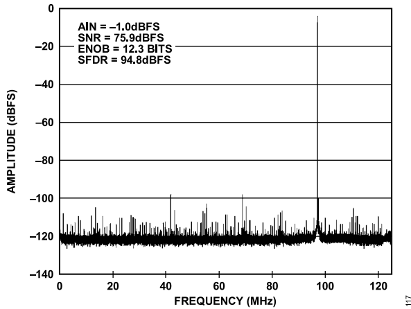
Figure 17. Single-Tone FFT with f_{IN} = 97.3 MHz, 2.5 V p-p FS, AD9467-250
