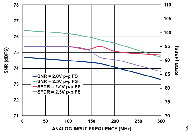
Figure 26. SNR/SFDR vs. f_{IN} , 2.0/2.5 V p-p FS, AD9467-200
