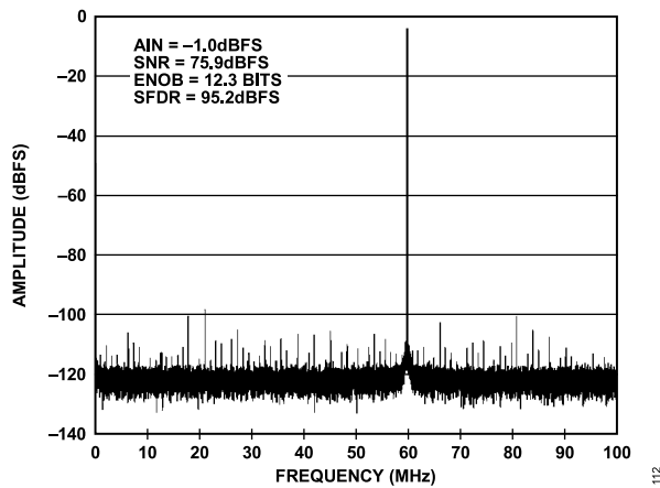
Figure 12. Single-Tone FFT with f_{IN} = 140.3 MHz, 2.5 V p-p FS, AD9467-200
