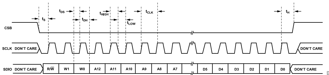
Figure 68. Serial Timing Details
