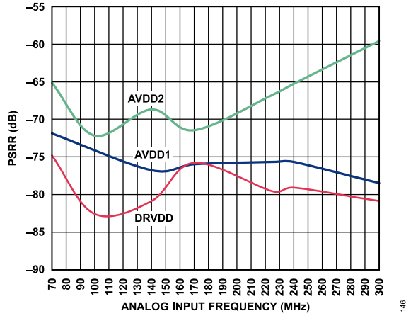
Figure 46. Power Supply Rejection (PSR), AD9467-250
