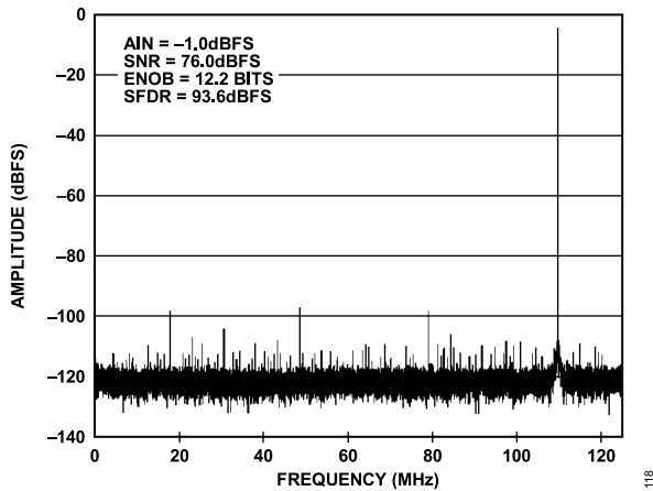
Figure 18. Single-Tone FFT with f_{IN} = 140.3 MHz, 2.5 V p-p FS, AD9467-250
