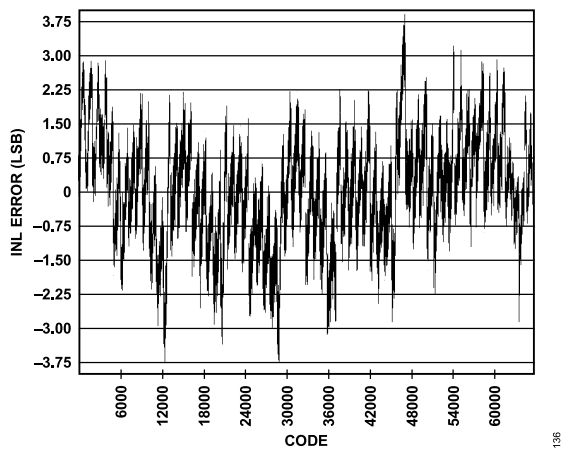
Figure 36. INL, f_{IN} = 4.3 MHz, 2.5 V p-p FS, AD9467-200
