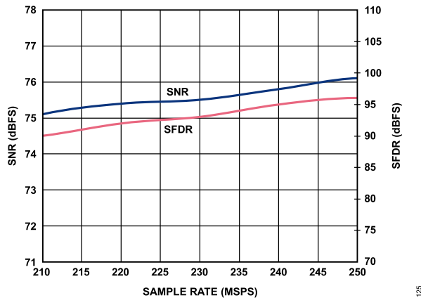
Figure 23. SNR/SFDR vs. f_{SAMPLE} , f_{IN} = 97.3 MHz, 2.5 V p-p FS, AD9467-250
