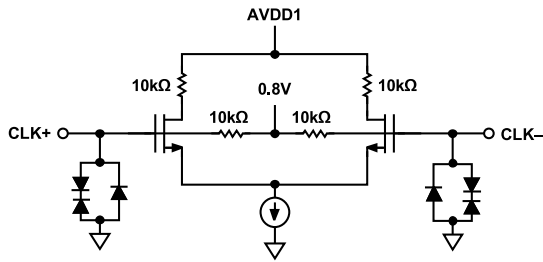
Figure 5. Equivalent Clock Input Circuit
