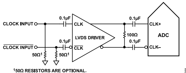
Figure 60. Differential LVDS Sample Clock
