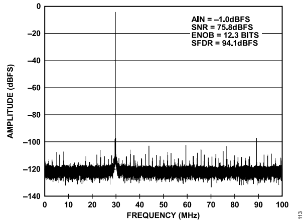
Figure 13. Single-Tone FFT with f_{IN} = 170.3 MHz, 2.5 V p-p FS, AD9467-200
