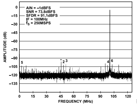
Figure 55. Single-Tone FFT Performance Plot Using the ADL5562 Amplifier, Gain = 6 dB, and the AD9467-250
