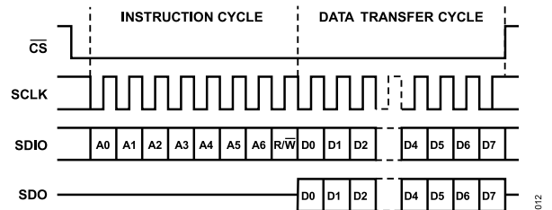
Figure 39. Serial Port Interface Timing, LSB First
