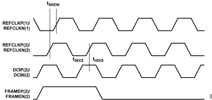
Figure 81. Timing Diagram Required for Synchronizing Devices
