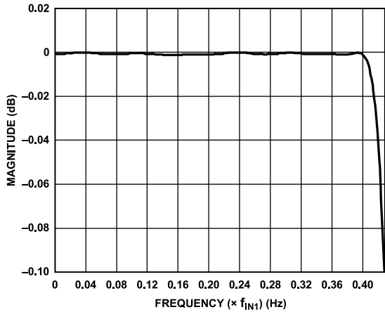
Figure 51. Pass-Band Detail of HB1
