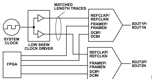
Figure 80. Typical Circuit Diagram for Synchronizing Devices
