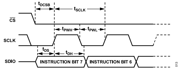
Figure 40. Timing Diagram for Serial Port Register Write
