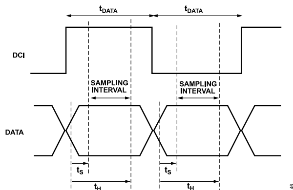
Figure 44. Timing Diagram for Input Data Port
