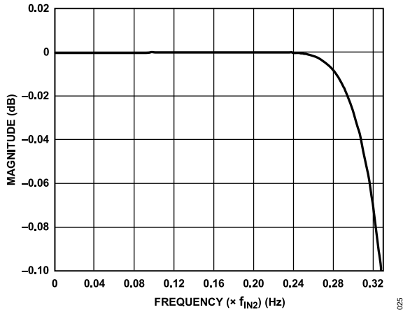
Figure 54. Pass-Band Detail of HB2
