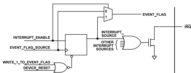
Figure 86. Simplified Schematic of \overline{\text{IRQ}} Circuitry
