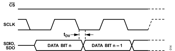
Figure 41. Timing Diagram for Serial Port Register Read
