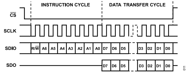
Figure 38. Serial Port Interface Timing, MSB First
