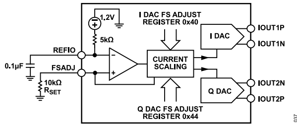
Figure 65. Simplified Block Diagram of DAC Core
