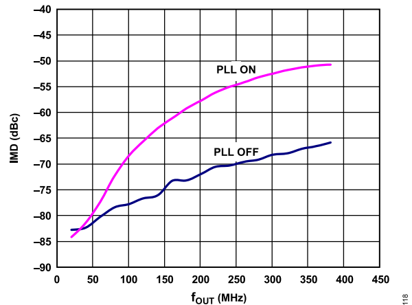
Figure 21. IMD vs. f_{OUT} , 4× Interpolation, f_{DATA} = 200\text{ MSPS} , Digital Scale = 0 dBFS, I_{FS} = 20\text{ mA} , PLL On and PLL Off
