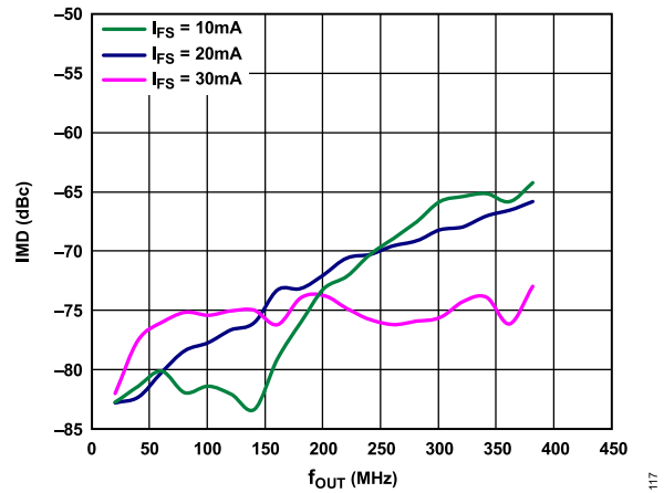
Figure 20. IMD vs. f_{OUT} over I_{FS} , 2× Interpolation, f_{DATA} = 400\text{ MSPS} , Digital Scale = 0 dBFS
