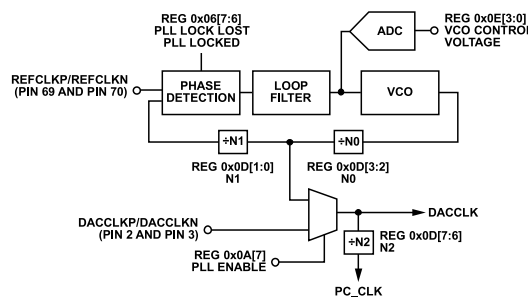
Figure 63. PLL Clock Multiplication Circuit
