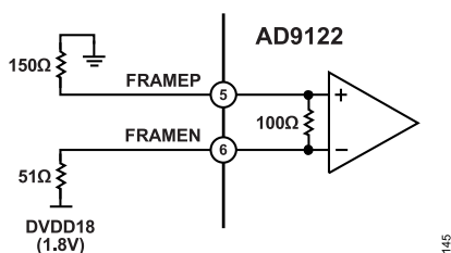
Figure 45. External Bias Circuit
