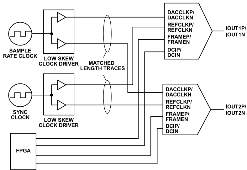
Figure 82. Typical Circuit Diagram for Synchronizing Devices to a System Clock
