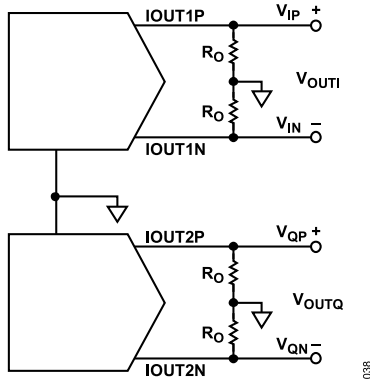
Figure 67. Basic Transmit DAC Output Circuit
