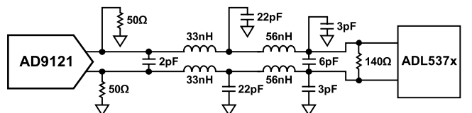
Figure 74. DAC Modulator Interface with Fifth-Order, Low-Pass Filter
