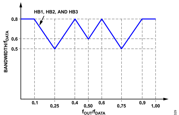
Figure 58. Signal Bandwidth vs. Center Frequency of the Output Signal, 8x Interpolation
