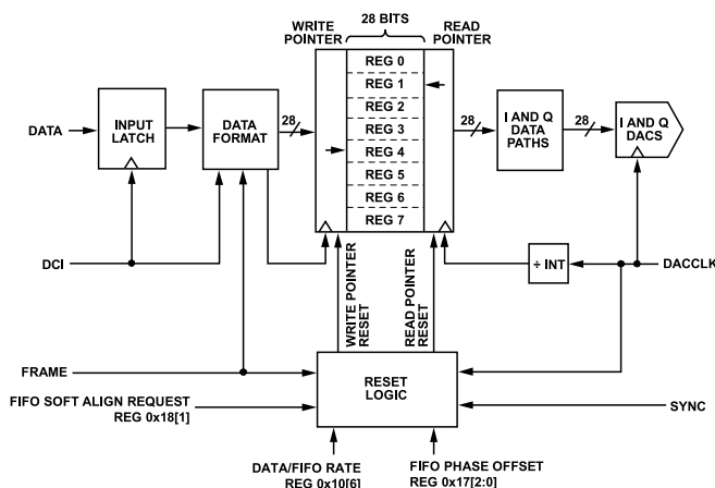
Figure 46. Block Diagram of FIFO
