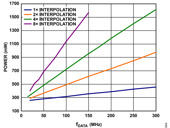
Figure 75. Total Power Dissipation vs. f_{\text{DATA}} Without PLL, Fine NCO, or Inverse Sinc
