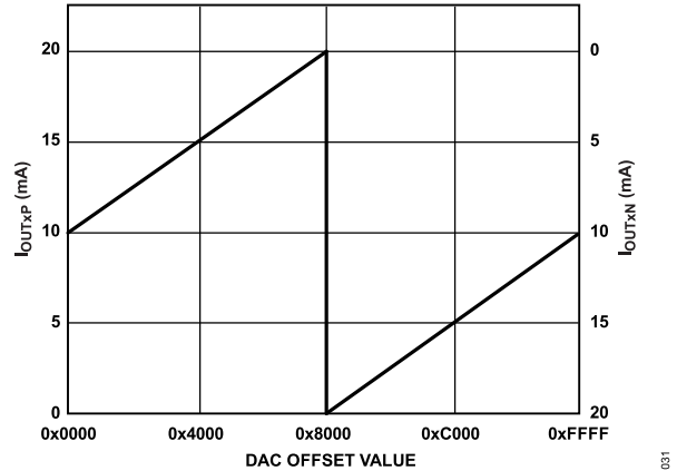
Figure 60. DAC Output Currents vs. DAC Offset Value
