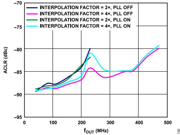
Figure 34. One-Carrier W-CDMA ACLR vs. f_{OUT} over Interpolation, Second Alternate Channel, PLL On and PLL Off
