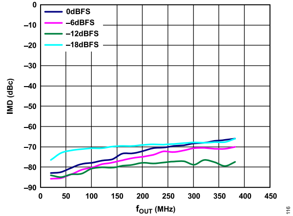
Figure 19. IMD vs. f_{OUT} over Digital Scale, 2× Interpolation, f_{DATA} = 400\text{ MSPS} , I_{FS} = 20\text{ mA}
