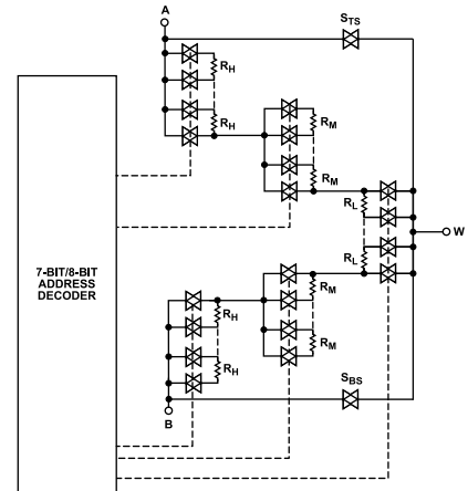
Figure 45. AD5121/AD5141 Simplified RDAC Circuit
