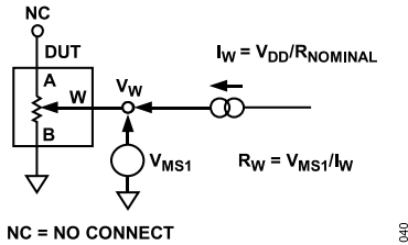
Figure 37. Wiper Resistance
