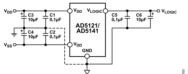
Figure 49. Power Supply Bypassing
