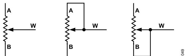
Figure 46. Rheostat Mode Configuration
