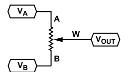
Figure 47. Potentiometer Mode Configuration
