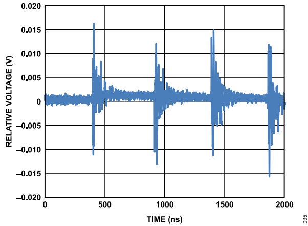
Figure 32. Digital Feedthrough
