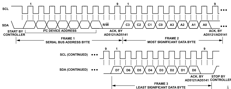
Figure 42. AD5121/AD5141 Interface Write Command
