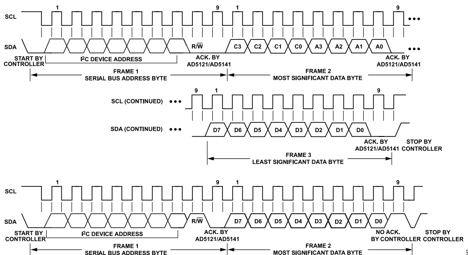
Figure 44. AD5121/AD5141 Interface Read Command
