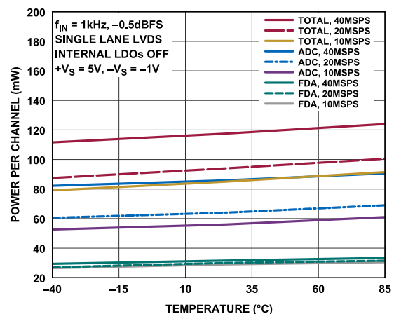
Figure 44. Power per Channel vs. Temperature, Normal Mode
