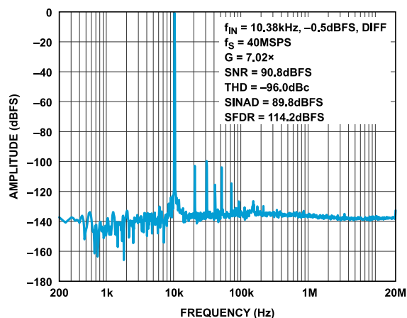
Figure 17. FFT 40MSPS, f_{IN} = 10.38\text{kHz} , Differential, -0.5\text{dBFS} , G = 7.02
