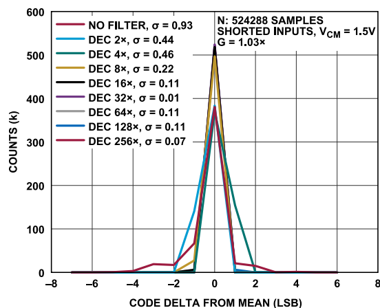
Figure 11. Histogram of Output Codes, Sinc5 + Compensation Filter
