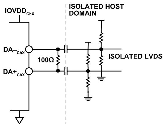
Figure 114. Isolated LVDS
