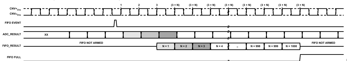
Figure 122. FIFO Data Capture Example, \text{WATERMARK} = 1000
