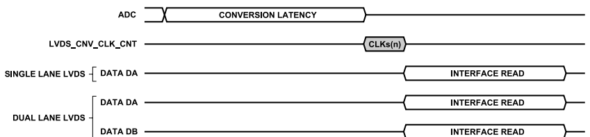
Figure 117. LVDS Data Transfer Latency
