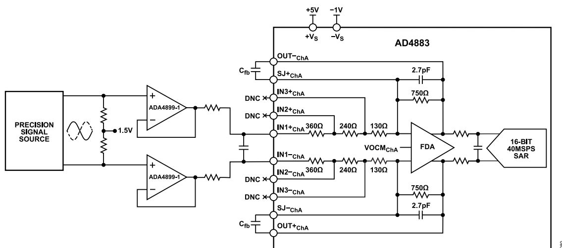
Figure 81. Typical Diagram for Minimum Distortion Laboratory Measurement
