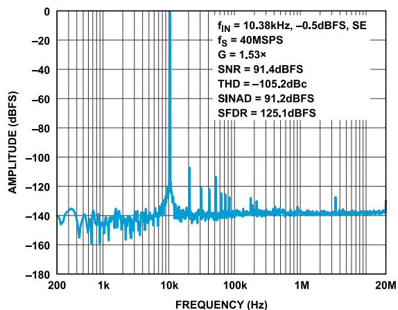
Figure 19. FFT 40MSPS, f_{IN} = 10.38\text{kHz} , Single-Ended, -0.5\text{dBFS} , G = 1.53
