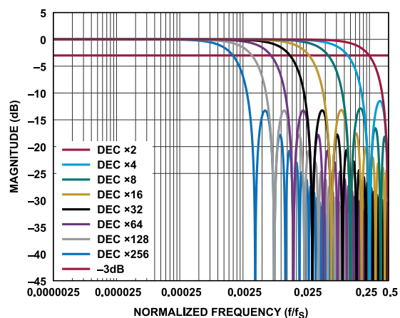
Figure 139. Sinc1 Filter Response, All Decimation Rates
