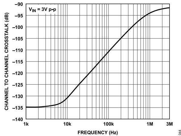
Figure 46. Channel-to-Channel Crosstalk
