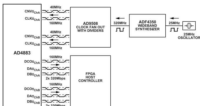
Figure 84. Dual Lane, LVDS Data Interface Clocking Example
