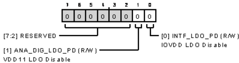
Figure 165. Power Control Register
