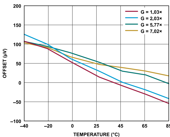
Figure 39. Offset Error vs. Temperature
