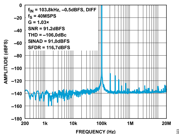
Figure 23. FFT 40MSPS, f_{IN} = 103.8\text{kHz} , Differential, -0.5\text{dBFS} , G = 1.03
