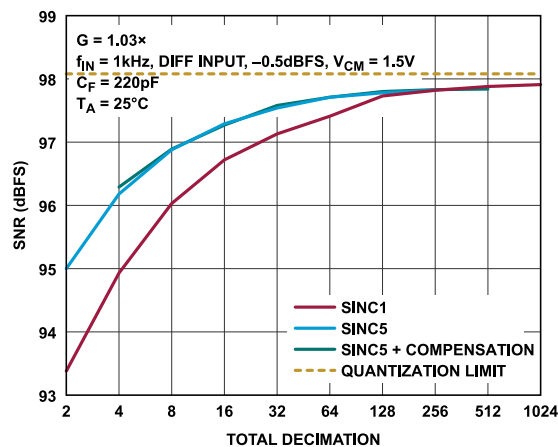
Figure 37. SNR vs. Total Decimation
