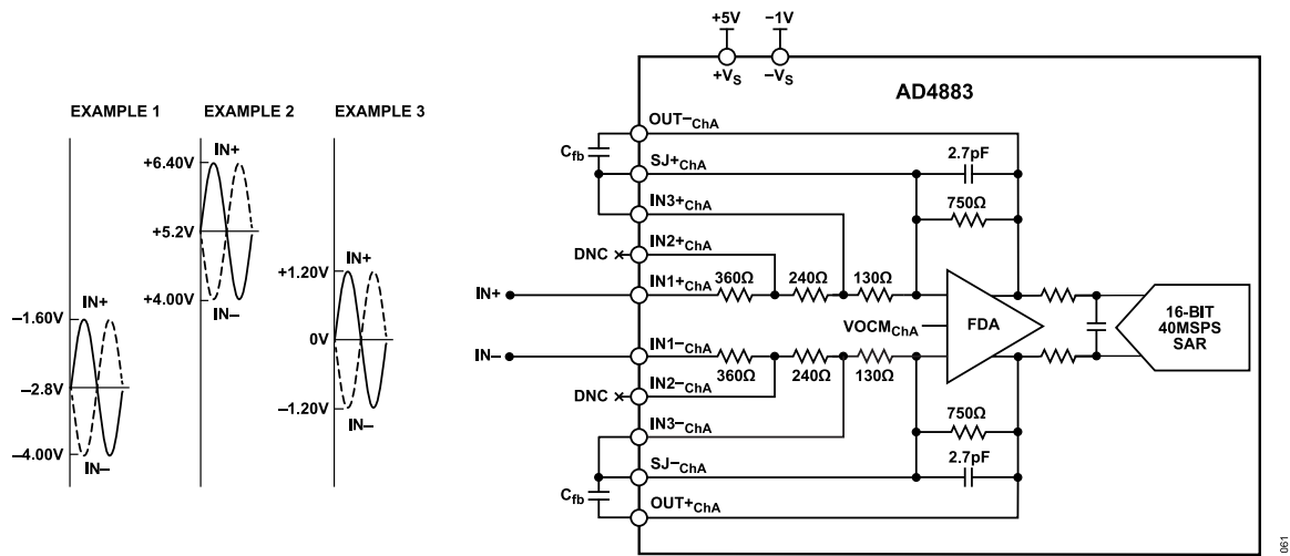
Figure 62. AD4883 Differential Input Configuration with Gain = 1.25, ±2.40V Input Range
