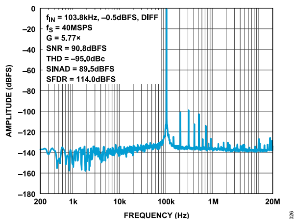
Figure 26. FFT 40MSPS, f_{IN} = 103.8\text{kHz} , Differential, -0.5\text{dBFS} , G = 5.77
