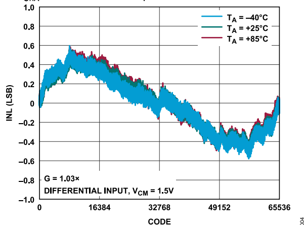
Figure 4. INL vs. Output Code, Differential Input Drive
