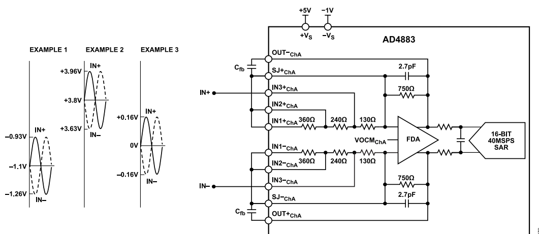
Figure 73. AD4883 Differential Input Configuration with Gain = 8.92, \pm 0.34\text{V} Input Range
