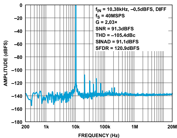
Figure 15. FFT 40MSPS, f_{IN} = 10.38\text{kHz} , Differential, -0.5\text{dBFS} , G = 2.03
