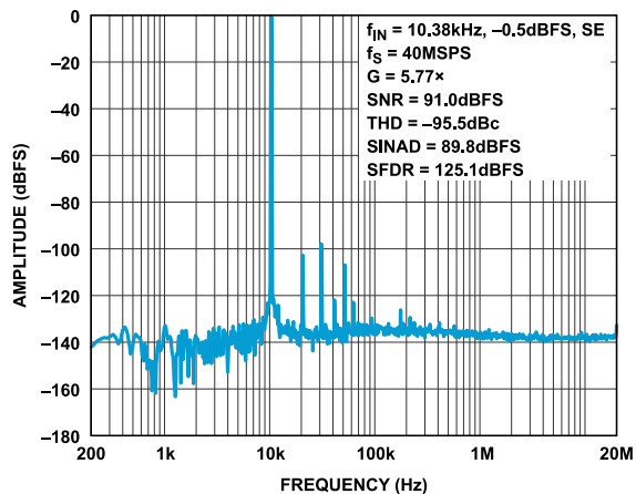
Figure 21. FFT 40MSPS, f_{IN} = 10.38\text{kHz} , Single-Ended, -0.5\text{dBFS} , G = 5.77
