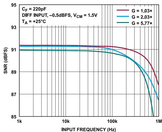
Figure 33. SNR vs. Input Frequency
