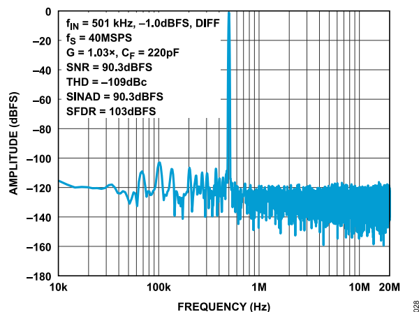
Figure 28. FFT 40MSPS, f_{IN} = 501\text{kHz} , Differential, -1\text{dBFS} , G = 1.03
