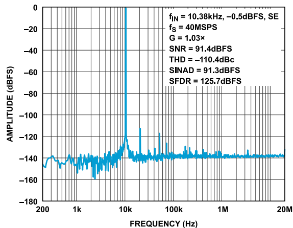
Figure 18. FFT 40MSPS, f_{IN} = 10.38\text{kHz} , Single-Ended, -0.5\text{dBFS} , G = 1.03
