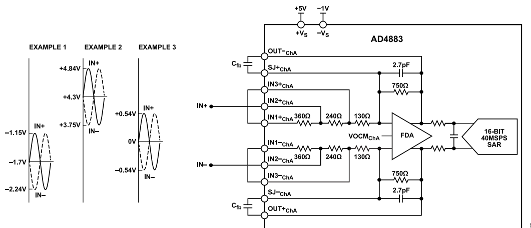
Figure 66. AD4883 Differential Input Configuration with Gain = 2.74, \pm 1.10\text{V} Input Range
