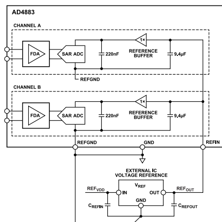
Figure 82. AD4883 General External Reference Design Functional Diagram
