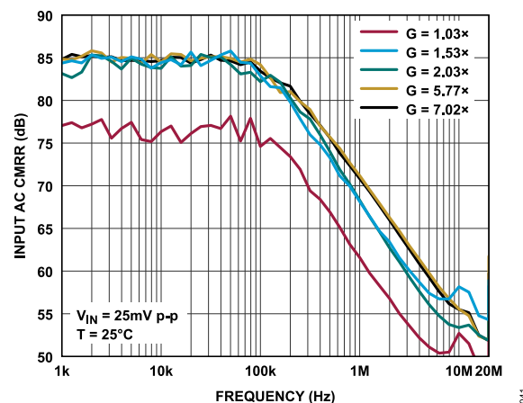
Figure 41. Input AC Common-Mode Rejection Ratio (CMRR) vs. Frequency
