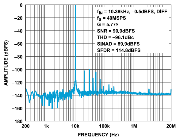
Figure 16. FFT 40MSPS, f_{IN} = 10.38\text{kHz} , Differential, -0.5\text{dBFS} , G = 5.77
