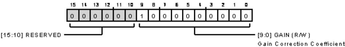
Figure 175. Gain Correction Register
