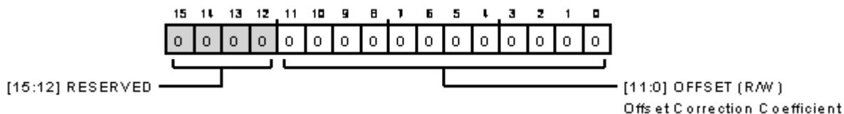
Figure 174. Offset Correction Register
