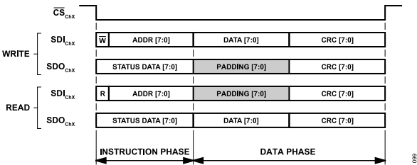
Figure 100. Short Instruction Mode, Data Status Enabled, CRC Enabled
