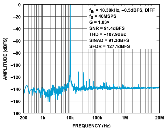
Figure 13. FFT 40MSPS, f_{IN} = 10.38\text{kHz} , Differential, -0.5\text{dBFS} , G = 1.03
