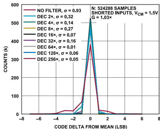
Figure 10. Histogram of Output Codes, Sinc5 Filter
