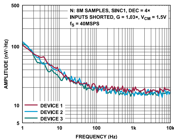
Figure 38. Low Frequency Noise, Inputs Shorted
