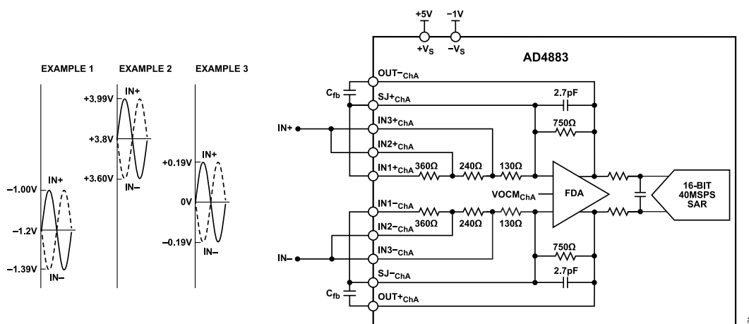
Figure 72. AD4883 Differential Input Configuration with Gain = 7.86, \pm 0.38\text{V} Input Range
