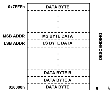
Figure 93. Generic Byte Wide Memory, Multibyte Register Example
