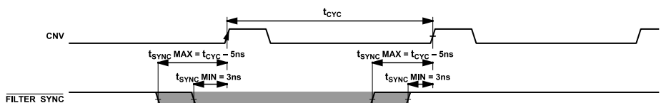
Figure 134. Filter Reset Timing
