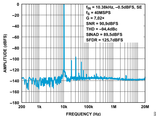
Figure 22. FFT 40MSPS, f_{IN} = 10.38\text{kHz} , Single-Ended, -0.5\text{dBFS} , G = 7.02
