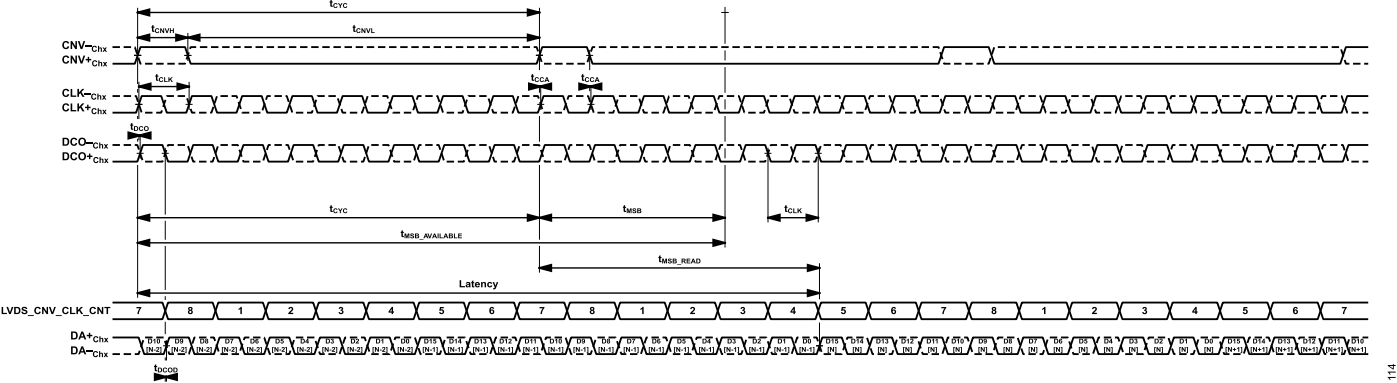
Figure 115. Single Lane LVDS, Echo Clock Mode, LVDS_CNV_CLK_CNT Position Example
