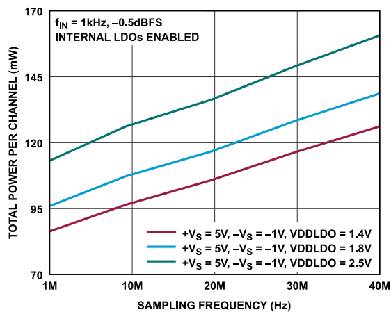
Figure 43. Total Power per Channel vs. Sampling Frequency, LDOs Enabled
