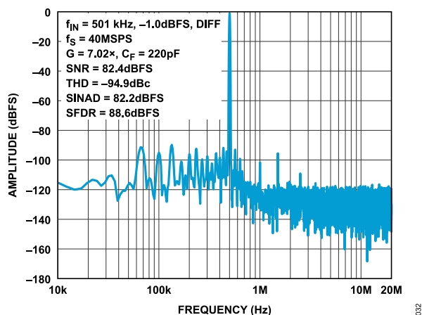
Figure 32. FFT 40MSPS, f_{IN} = 501\text{kHz} , Differential, -1\text{dBFS} , G = 7.02
