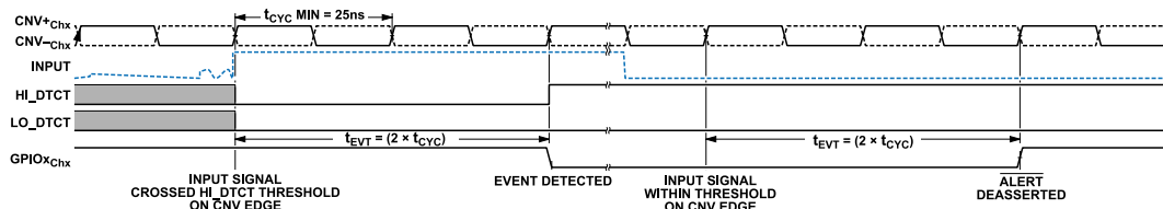
Figure 119. Event Detection Timing
