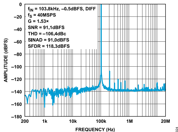
Figure 24. FFT 40MSPS, f_{IN} = 103.8\text{kHz} , Differential, -0.5\text{dBFS} , G = 1.53
