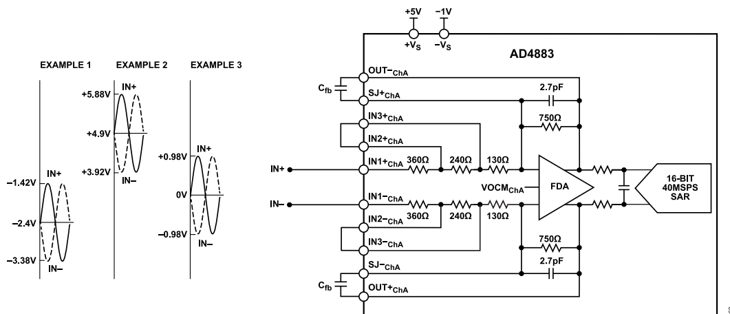
Figure 63. AD4883 Differential Input Configuration with Gain = 1.53, \pm 1.96\text{V} Input Range
