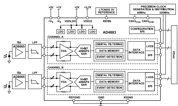
Figure 1. AD4883 Typical Application Diagram
