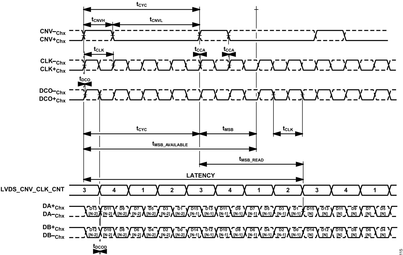
Figure 116. Dual Lane LVDS, Echo Clock Mode, LVDS_CNV_CLK_CNT Position Example
