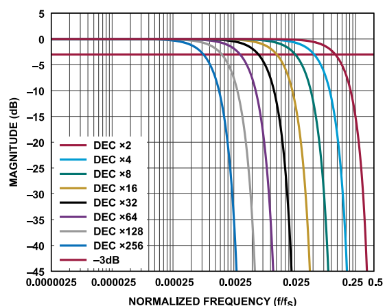
Figure 140. Sinc5 Filter Response, All Decimation Rates
