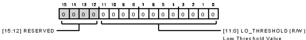
Figure 173. Event Detection Low Threshold Configuration Register
