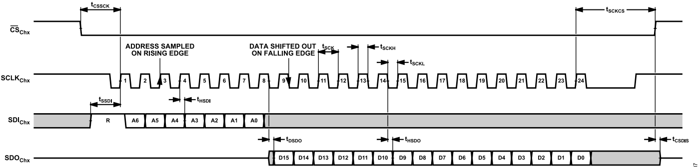
Figure 108. Configuration SPI Timing, Data Read Frame, 8-Bit Instruction Mode, Streaming Mode, Multibyte Register
