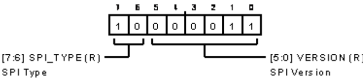
Figure 154. SPI Revision Register
