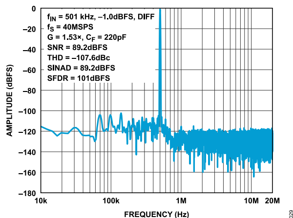
Figure 29. FFT 40MSPS, f_{IN} = 501\text{kHz} , Differential, -1\text{dBFS} , G = 1.53
