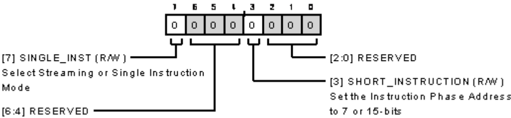
Figure 147. Additional Interface Configuration B Settings
