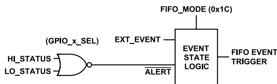
Figure 121. FIFO Event Detection Logic
