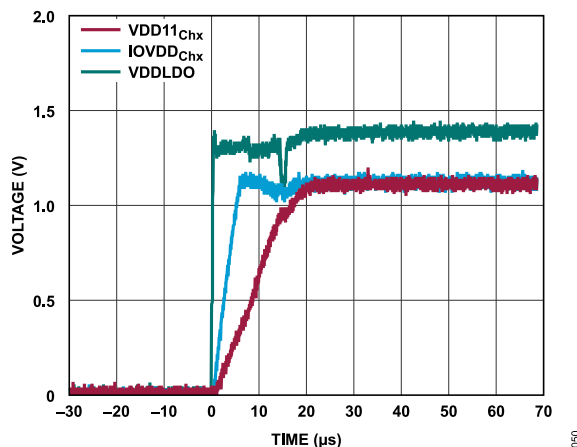
Figure 51. Typical Regulator Start-Up Transient, Converter Idle
