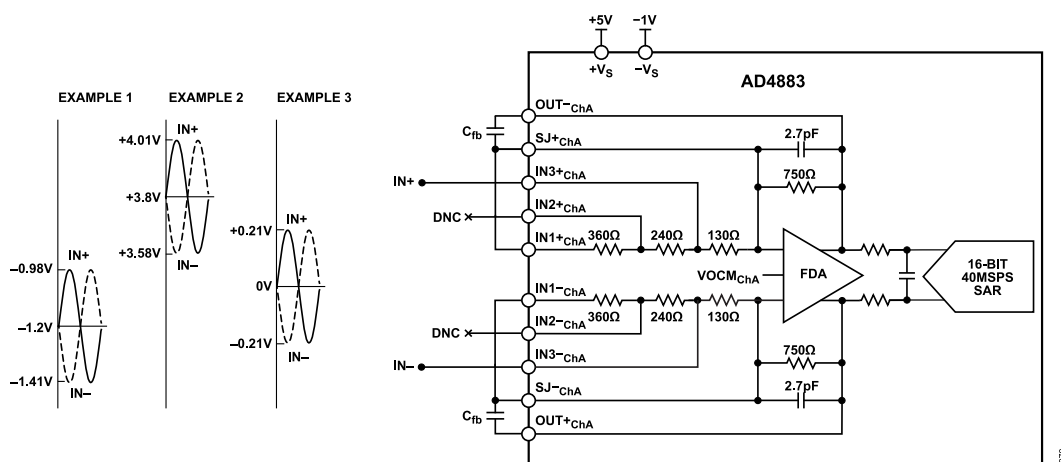
Figure 71. AD4883 Differential Input Configuration with Gain = 7.02, \pm 0.43\text{V} Input Range
