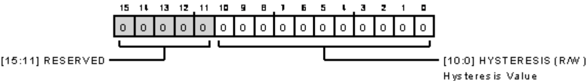
Figure 171. Event Detection Hysteresis Configuration Register
