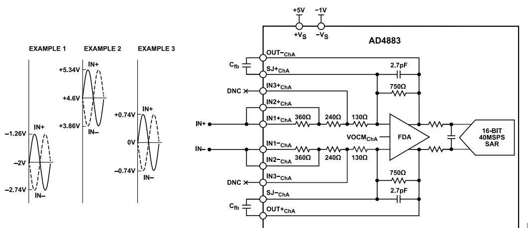
Figure 64. AD4883 Differential Input Configuration with Gain = 2.03, \pm 1.48\text{V} Input Range
