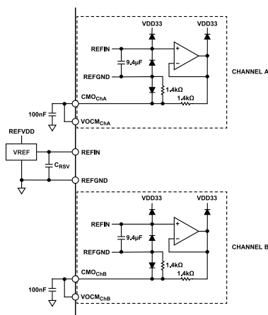
Figure 50. REFIN and CMO Internal Equivalent Circuit and Typical Application
