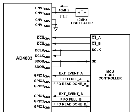
Figure 86. SPI Data Interface Clocking Example, Shared SPI Bus
