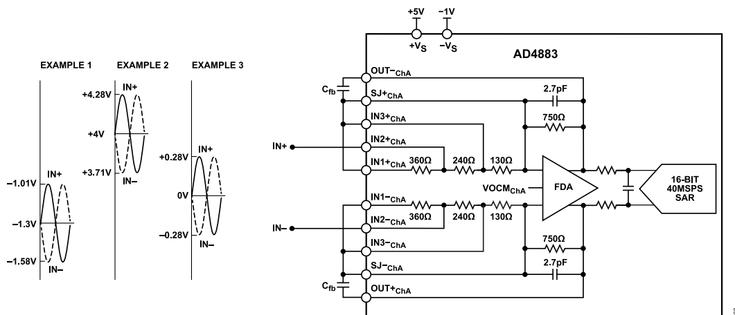
Figure 69. AD4883 Differential Input Configuration with Gain = 5.21, \pm 0.58\text{V} Input Range
