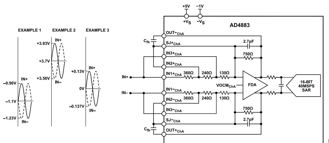
Figure 74. AD4883 Differential Input Configuration with Gain = 10.98, \pm 0.27\text{V} Input Range
