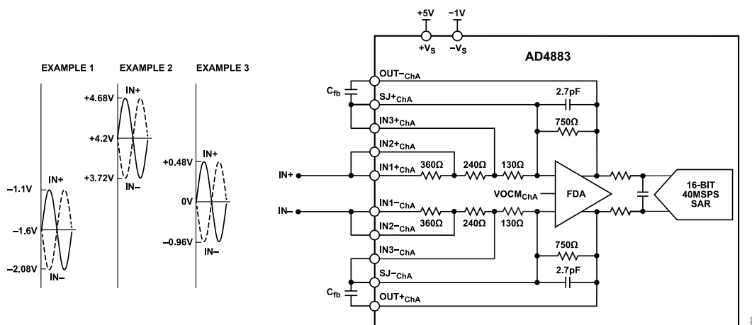
Figure 67. AD4883 Differential Input Configuration with Gain = 3.13, \pm 0.96\text{V} Input Range
