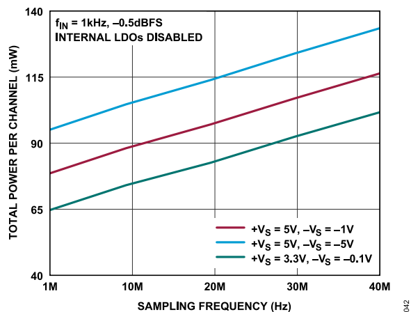
Figure 42. Total Power per Channel vs. Sampling Frequency, LDOs Disabled
