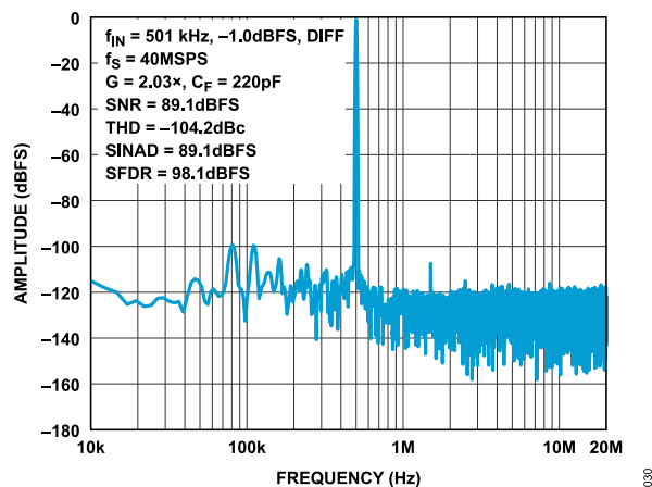
Figure 30. FFT 40MSPS, f_{IN} = 501\text{kHz} , Differential, -1\text{dBFS} , G = 2.03
