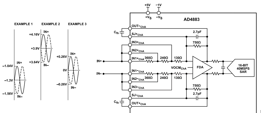
Figure 70. AD4883 Differential Input Configuration with Gain = 5.77, \pm 0.52\text{V} Input Range
