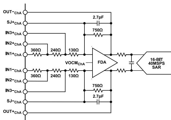
Figure 58. AD4883 Input (Shown for Channel A)
