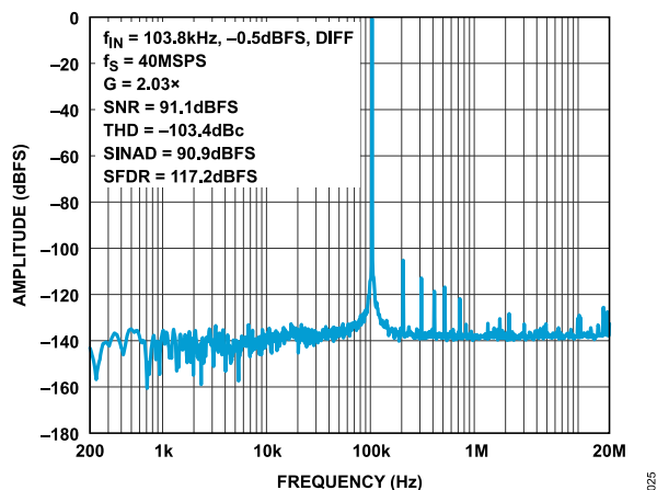
Figure 25. FFT 40MSPS, f_{IN} = 103.8\text{kHz} , Differential, -0.5\text{dBFS} , G = 2.03
