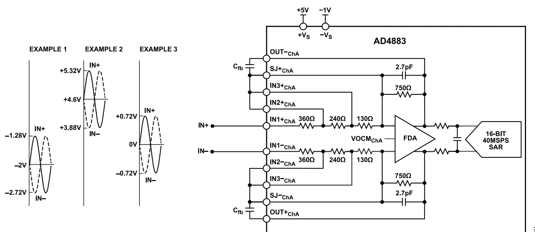
Figure 65. AD4883 Differential Input Configuration with Gain = 2.08, \pm 1.44\text{V} Input Range
