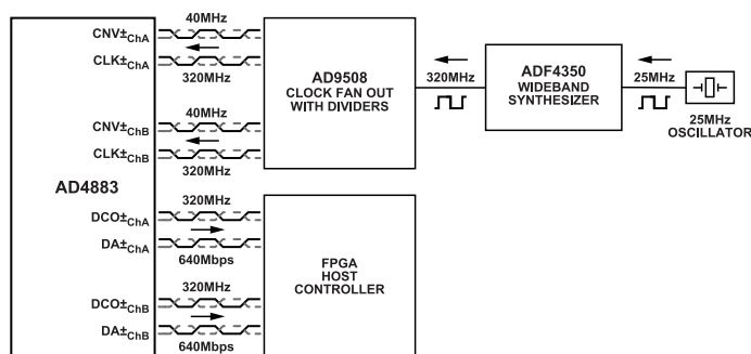
Figure 83. Single Lane, LVDS Data Interface Clocking Example
