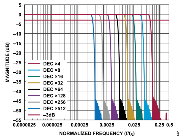
Figure 143. Sinc5 + Compensation Filter Response
