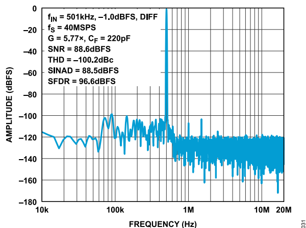
Figure 31. FFT 40MSPS, f_{IN} = 501\text{kHz} , Differential, -1\text{dBFS} , G = 5.77
