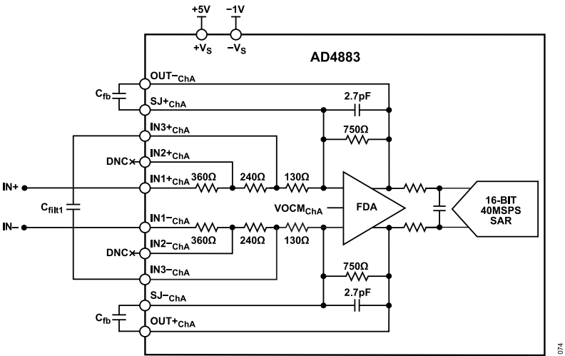
Figure 75. AD4883 FDA Stage, G = 1.03 , One Additional Capacitor for 2nd Order Response, Option 1
