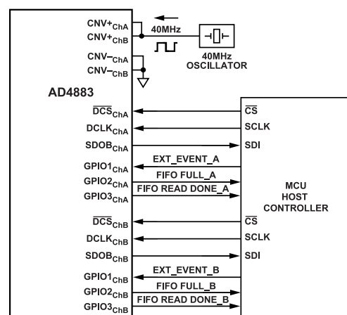
Figure 85. SPI Data Interface Clocking Example, x2 SPI Ports
