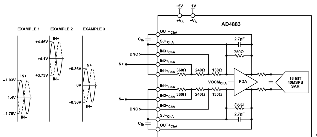
Figure 68. AD4883 Differential Input Configuration with Gain = 4.11, \pm 0.73\text{V} Input Range
