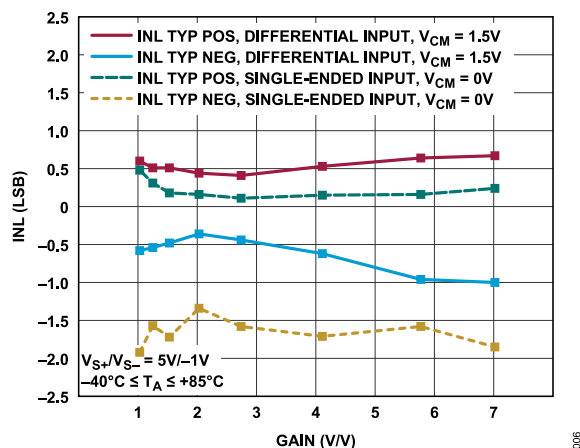
Figure 6. INL vs. Gain
