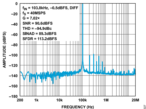
Figure 27. FFT 40MSPS, f_{IN} = 103.8\text{kHz} , Differential, -0.5\text{dBFS} , G = 7.02
