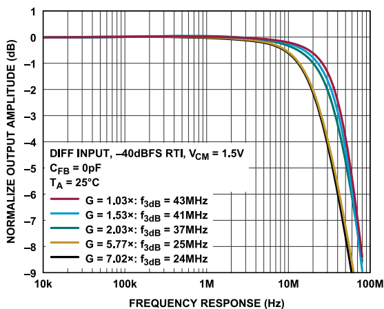
Figure 12. Small Signal Frequency Response, 40MSPS
