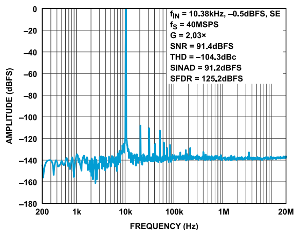
Figure 20. FFT 40MSPS, f_{IN} = 10.38\text{kHz} , Single-Ended, -0.5\text{dBFS} , G = 2.03
