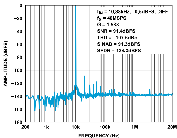
Figure 14. FFT 40MSPS, f_{IN} = 10.38\text{kHz} , Differential, -0.5\text{dBFS} , G = 1.53
