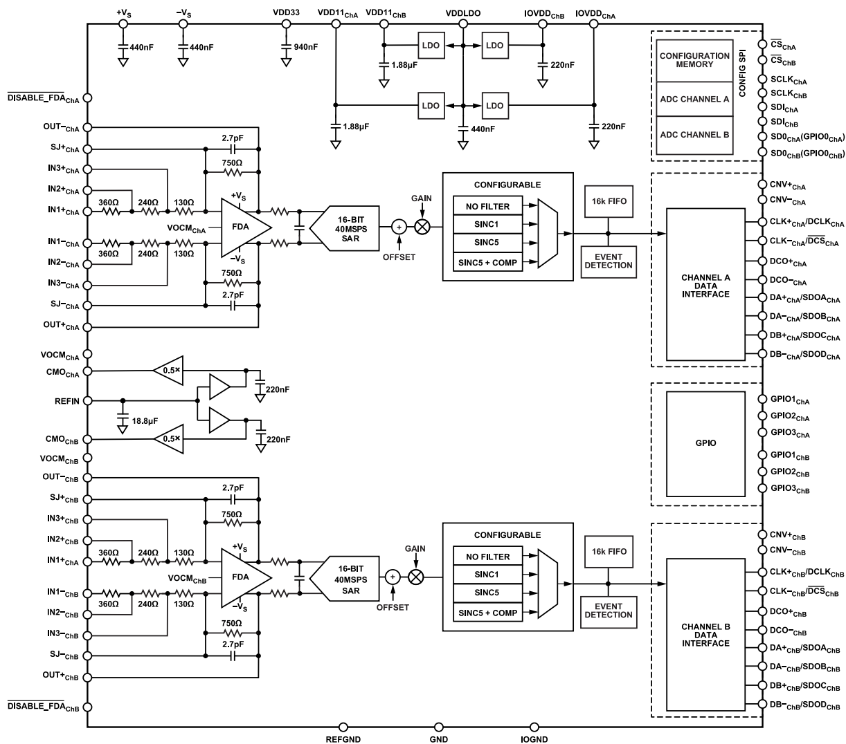
Figure 2. AD4883 Functional Block Diagram
