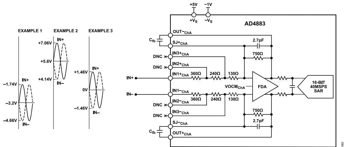
Figure 61. AD4883 Differential Input Configuration with Gain = 1.03, ±2.91V Input Range
