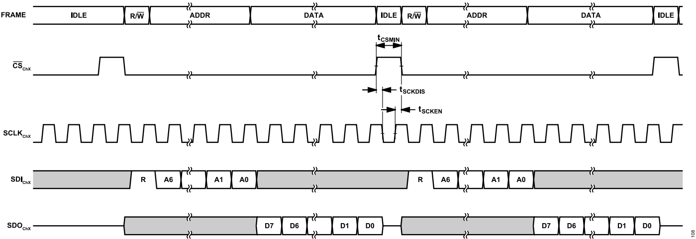
Figure 109. Configuration SPI Timing, Data Read Frame, Continuous SCLK ChX
