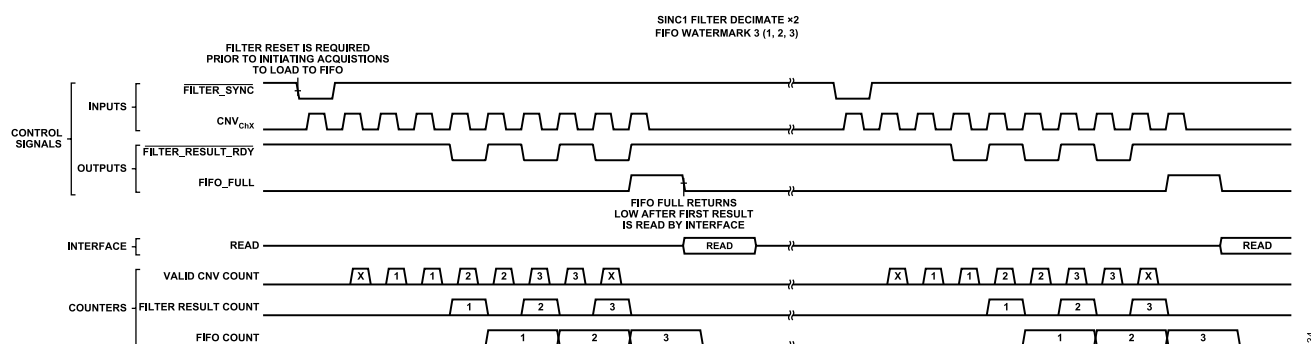
Figure 135. Description of Filter Timing with FIFO
