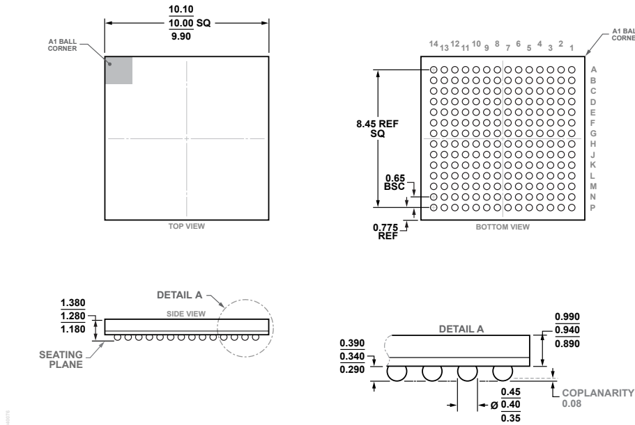
Figure 177. 196-Ball Chip-Scale Package Ball Grid Array [CSP_BGA] (BC-196-20) Dimensions shown in millimeters
