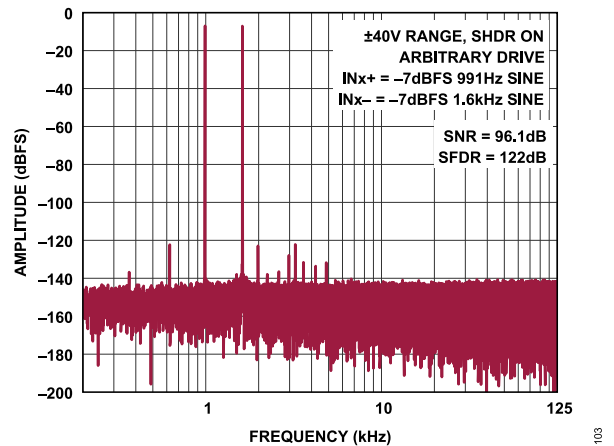
Figure 25. FFT, 250kSPS, f_{INx+} = 991\text{Hz} , f_{INx-} = 1.6\text{kHz} , \pm 40\text{V} Range
