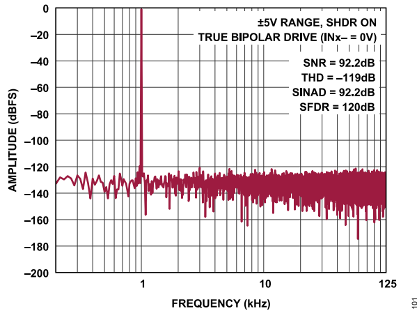
Figure 22. FFT, 250kSPS, f_{IN} = 1\text{kHz} , \pm 5\text{V} Range
