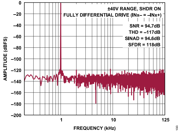
Figure 21. FFT, 250kSPS, f_{IN} = 1\text{kHz} , \pm 40\text{V} Range
