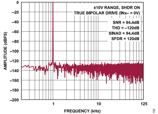
Figure 24. FFT, 250kSPS, f_{IN} = 1\text{kHz} , \pm 10\text{V} Range
