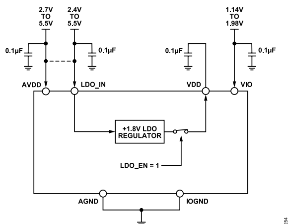
Figure 54. Powering VDD with the Internal LDO Regulator
