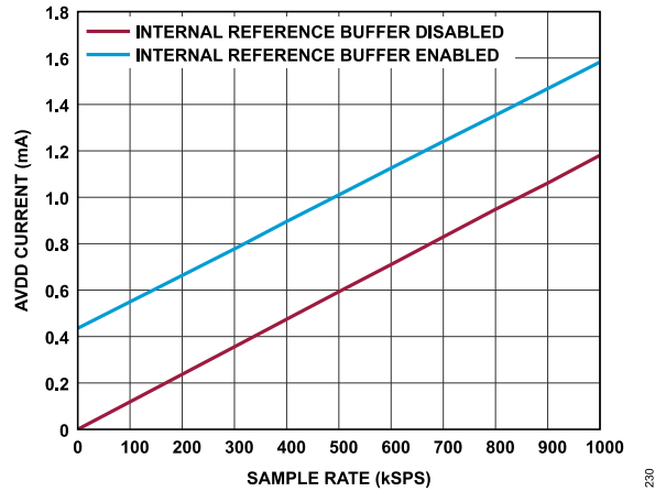
Figure 30. AVDD Current vs. Sample Rate
