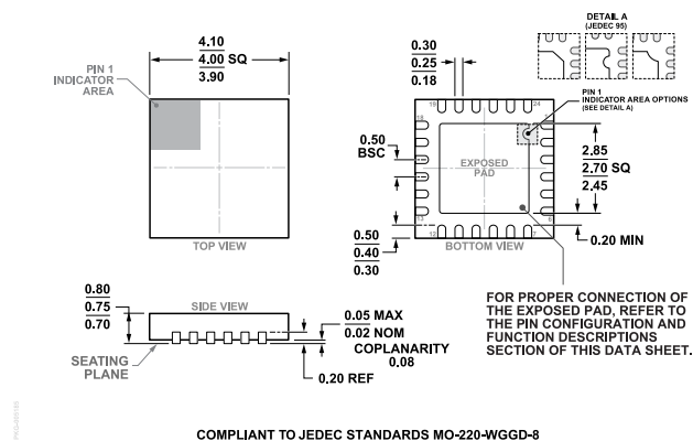
Figure 102. 24-Lead Lead Frame Chip Scale Package [LFCSP] 4mm × 4mm Body and 0.75mm Package Height (CP-24-8) Dimensions shown in millimeters
