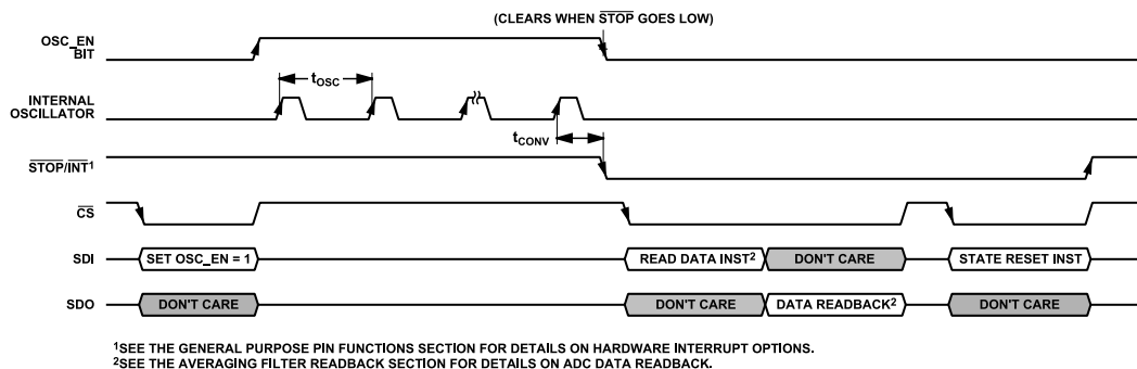
Figure 67. SPI Burst Mode Timing Diagram
