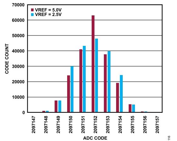
Figure 11. Histogram, Accumulator Depth = 64
