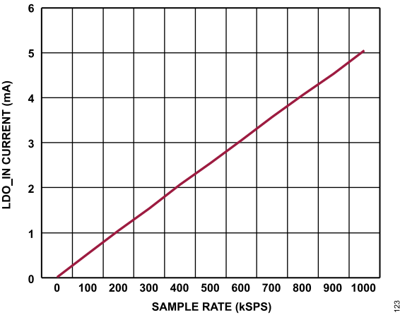
Figure 33. LDO_IN Current vs. Sample Rate
