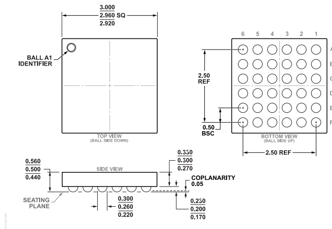
Figure 103. 36-Ball Wafer Level Chip Scale Package (WLCSP) (CB-36-5) Dimensions shown in millimeters
