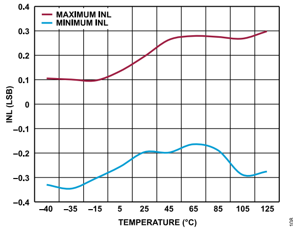
Figure 7. INL vs. Temperature
