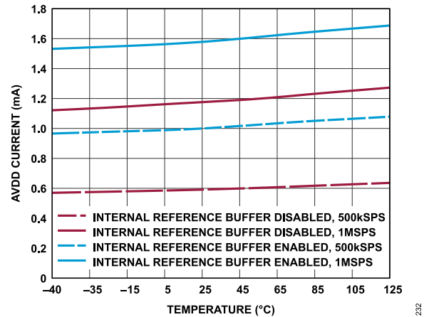
Figure 32. AVDD Current vs. Temperature
