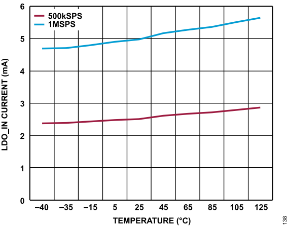
Figure 35. LDO_IN Current vs. Temperature
