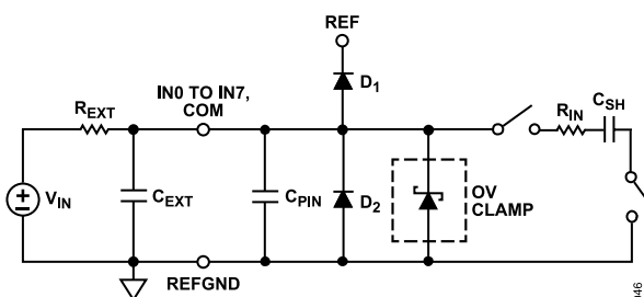
Figure 49. Equivalent Analog Input Circuit
