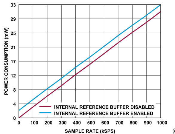
Figure 45. Power Consumption vs. Sample Rate (Internal LDO Enabled)
