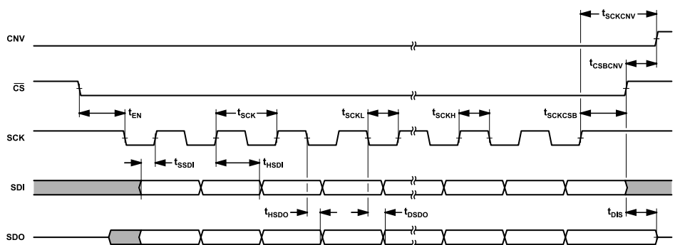
Figure 3. SPI Timing Specifications Definition Diagram
