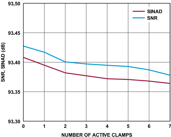
Figure 15. SNR and SINAD vs. Number of Active Clamps
