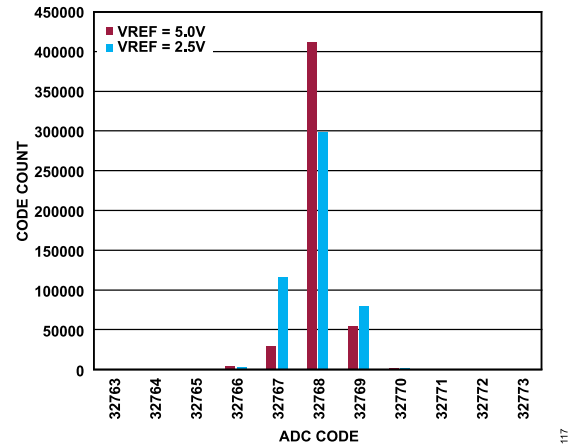
Figure 10. Histogram, Accumulator Depth = 1
