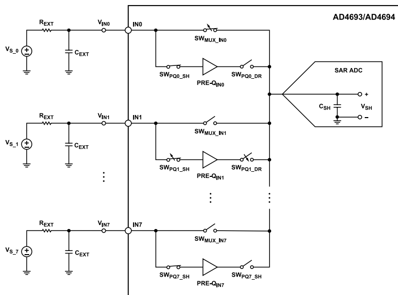
Figure 51. Precharge Buffer Simplified Circuit Diagram
