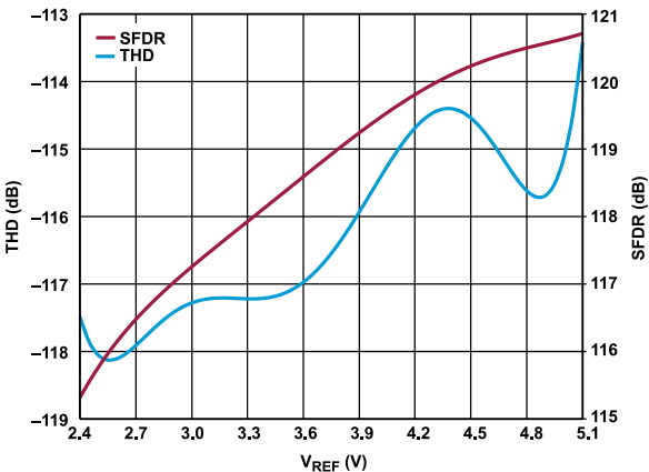
Figure 16. THD and SFDR vs. V_{REF}
