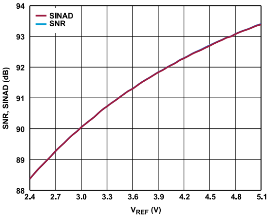
Figure 13. SNR and SINAD vs. V_{REF}
