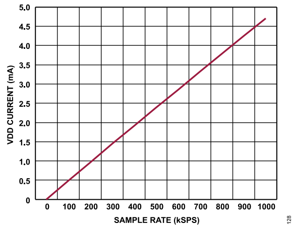
Figure 36. VDD Current vs. Sample Rate
