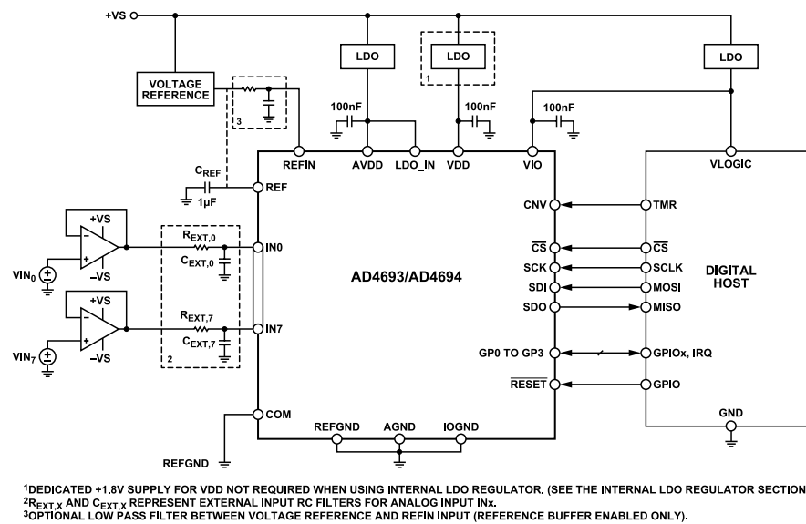
Figure 84. AD4693/AD4694 Typical Connection Diagram
