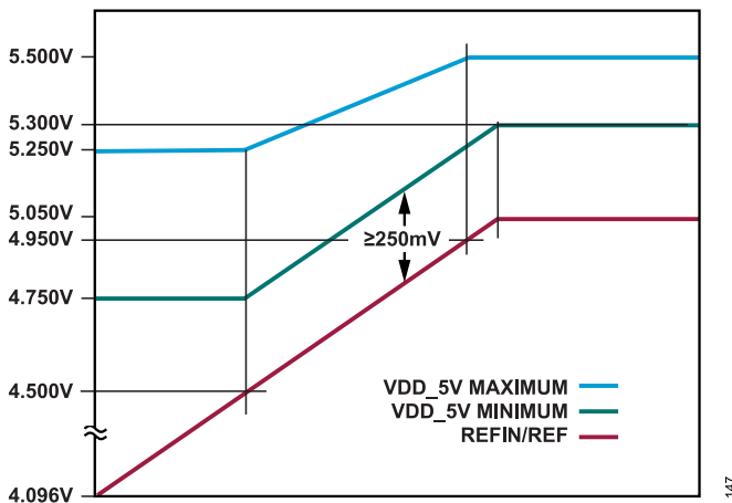
Figure 50. VDD_5V Minimum and Maximum Values for REFIN/REF
