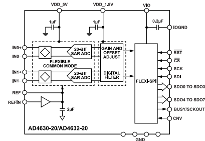
Figure 1. AD4630-20/AD4632-20 Functional Block Diagram
