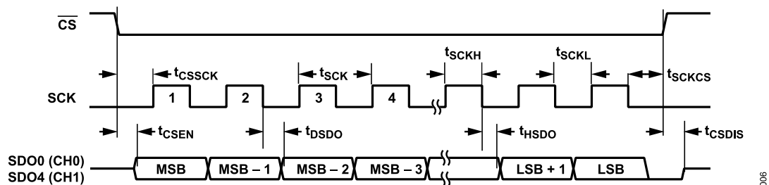
Figure 6. SPI Clcking Mode 1-Lane SDR Timing
