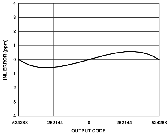
Figure 12. INL Error vs. Output Code, Differential Input
