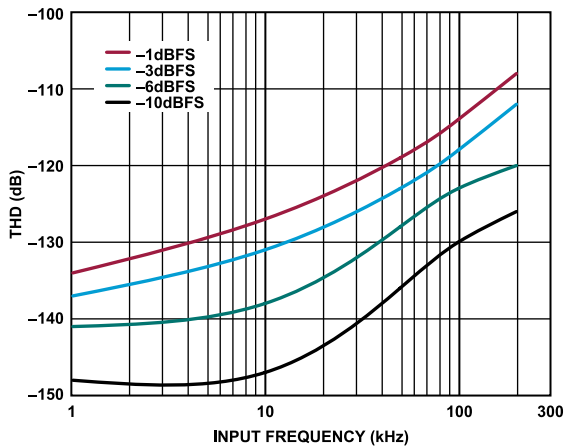
Figure 17. THD vs. Input Frequency and Amplitude
