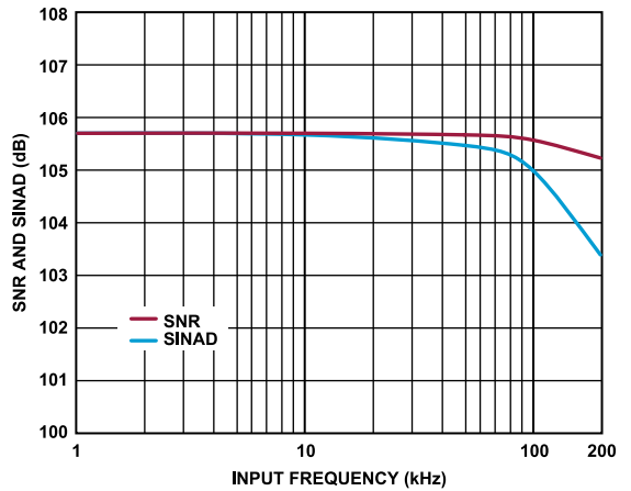
Figure 16. SNR and SINAD vs. Input Frequency
