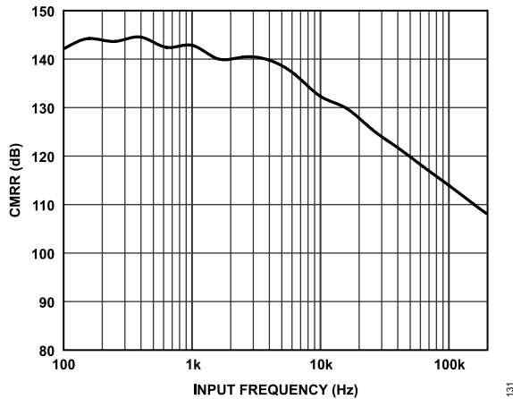
Figure 32. CMRR vs. Input Frequency
