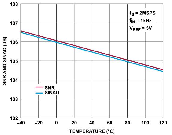
Figure 19. SNR and SINAD vs. Temperature, f_{IN} = 1\text{kHz}
