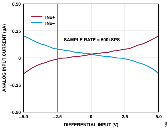
Figure 26. Analog Input Current vs. Differential Input, AD4632-20, 500kSPS
