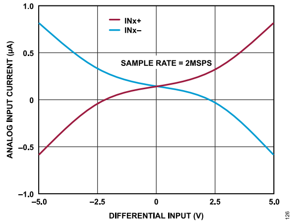
Figure 25. Analog Input Current vs. Differential Input, AD4630-20, 2MSPS
