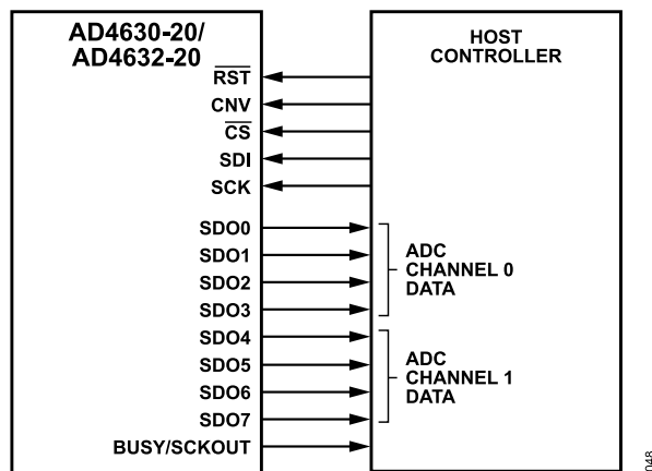
Figure 51. Multilane SPI
