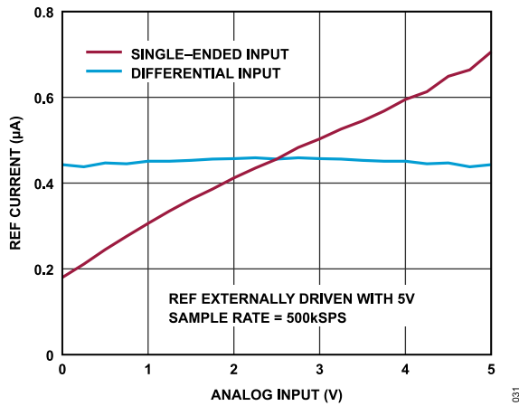
Figure 31. REF Current vs. Analog Input, AD4632-20, 500kSPS
