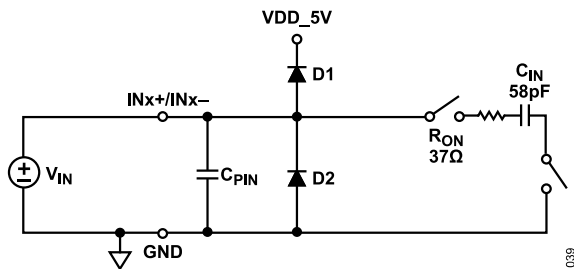
Figure 41. Equivalent Circuit for the AD4630-20/AD4632-20 Differential Analog Input
