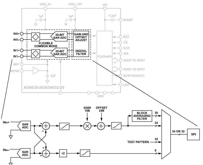
Figure 39. Functional Block Diagram and Channel Architecture
