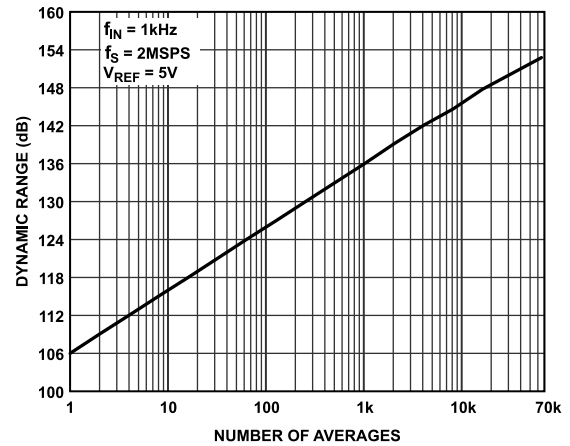
Figure 23. Dynamic Range vs. Number of Averages
