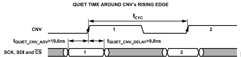
Figure 57. Quiet Zones
