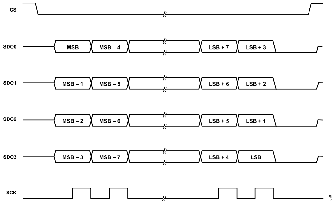
Figure 67. 4-Lane, SDR Timing Diagram
