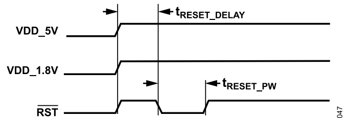
Figure 49. Power-On Reset (POR) Timing
