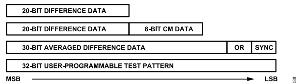
Figure 43. Summary of Selectable Output Sample Formats
