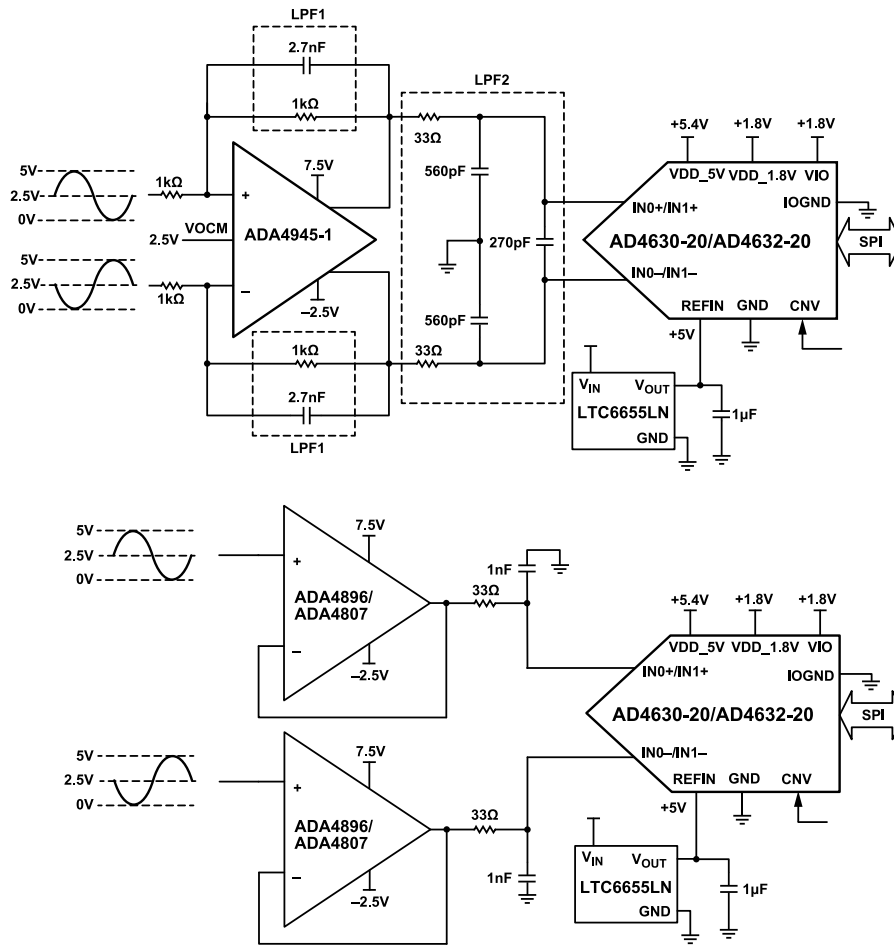
Figure 44. Typical Application Circuit Diagrams
