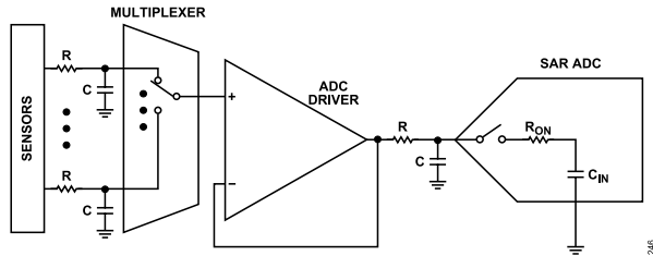
Figure 46. Multiplexed Data Acquisition Signal Using the AD4630-20/AD4632-20
