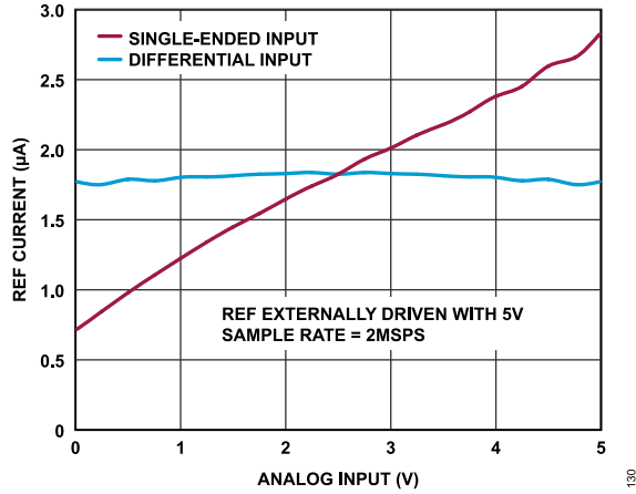
Figure 30. REF Current vs. Analog Input, AD4630-20, 2MSPS
