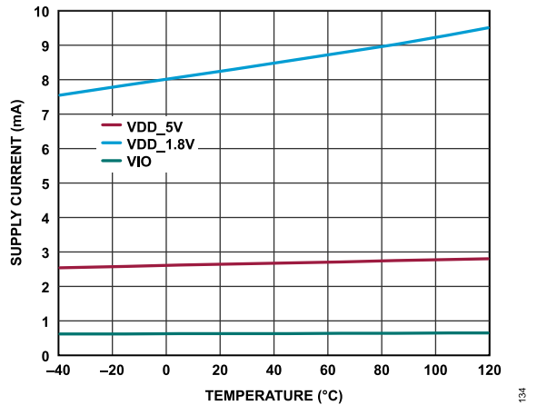
Figure 35. Supply Current vs. Temperature, AD4630-20, 2MSPS
