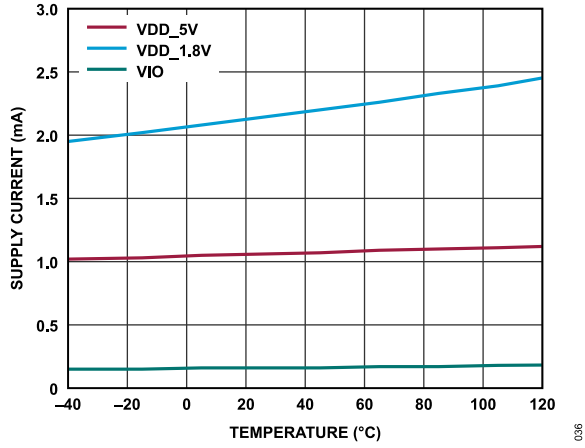
Figure 36. Supply Current vs. Temperature, AD4632-20, 500kSPS
