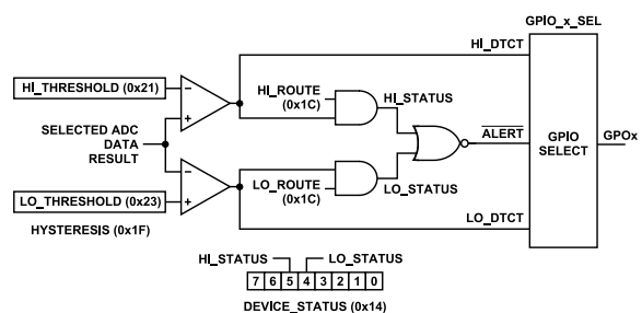
Figure 81. Internally Generated Event Detection Signal Path
