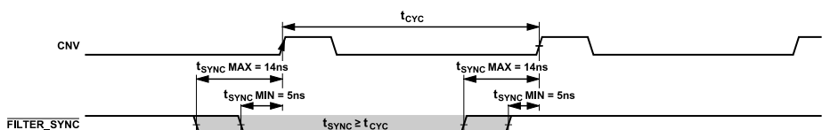
Figure 97. Filter Reset Timing
