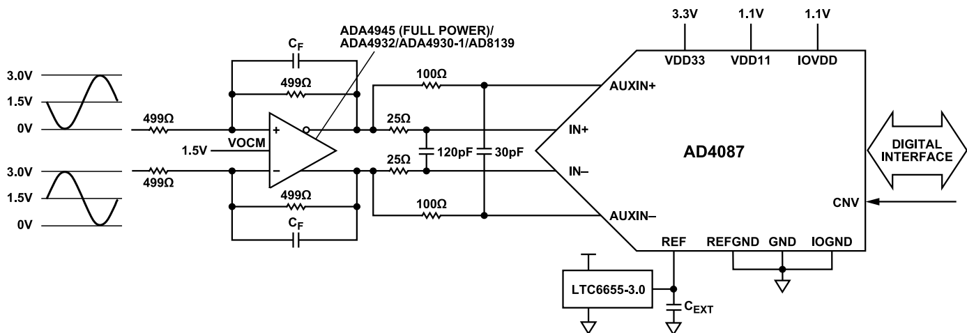
Figure 44. AD4087 Typical Applications Diagram, Fully Differential Amplifier
