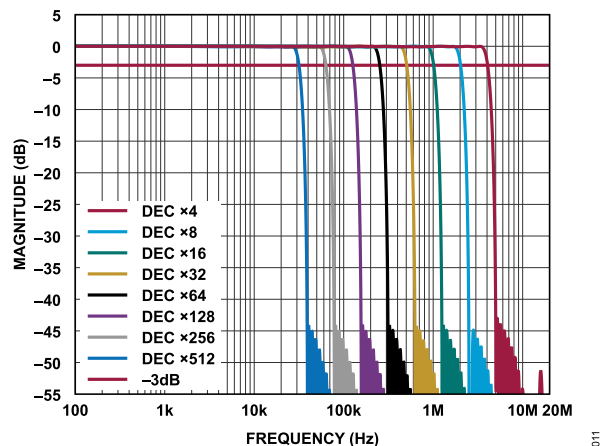
Figure 11. Sinc5 + Compensation Filter Response, f_s = 20\text{MHz}
