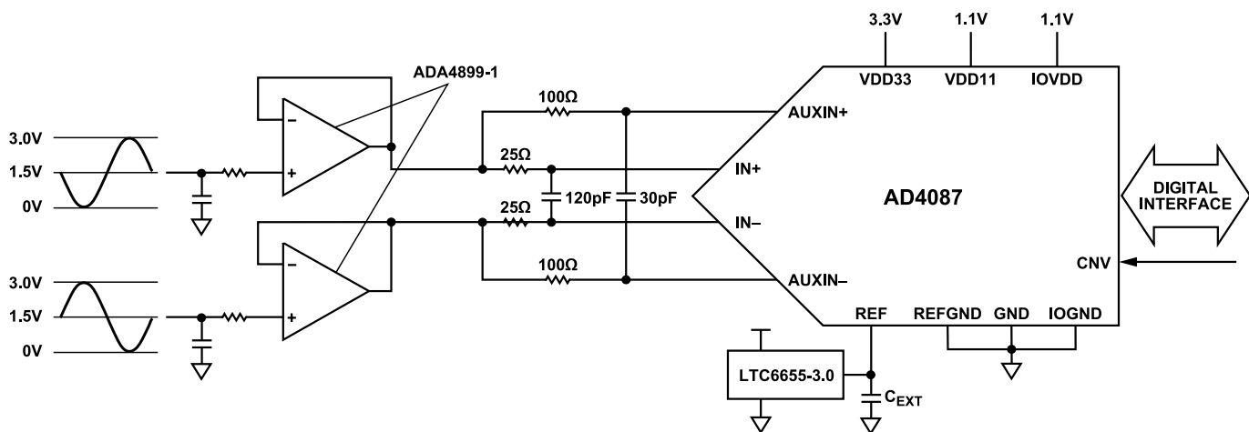
Figure 45. AD4087 Typical Applications Diagram, Single Op-Amp Drivers
