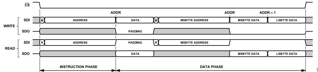
Figure 55. Interface Access Example, Single Instruction Mode (SINGLE_INST = 1), All Other Interface Options Default
