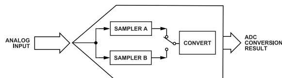
Figure 30. Simplified Representation of the AD4087 SAR ADC
