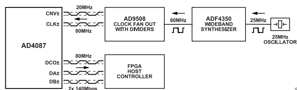
Figure 48. Dual Lane, LVDS Data Interface Clocking Example
