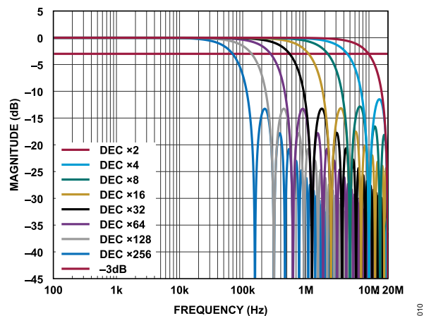
Figure 10. Sinc5 Filter Response, f_s = 20\text{MHz}
