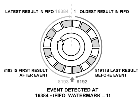
Figure 92. Event Capture Mode Read All FIFO Mode Example, FIFO Filling
