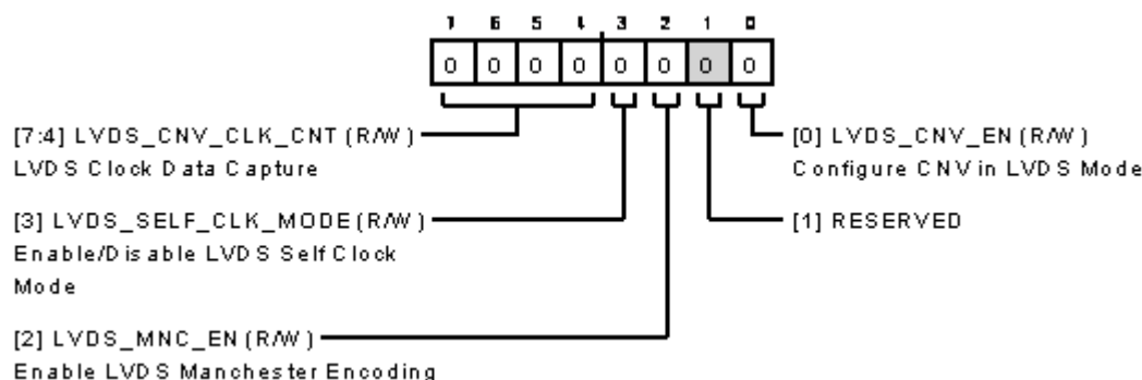
Figure 126. ADC Data Interface Configuration B Register
