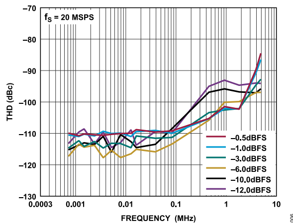
Figure 6. THD vs. Input Signal Frequency (Amplitude = -0.5\text{ dBFS} , -1\text{ dBFS} , -3\text{ dBFS} , -6\text{ dBFS} , -10\text{ dBFS} , and -12\text{ dBFS} )
