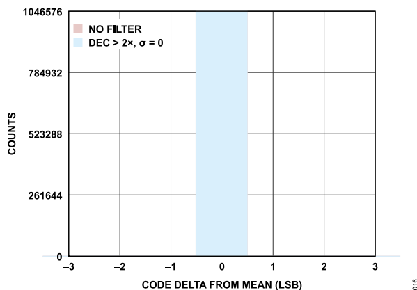
Figure 16. Histogram of Codes, Sinc1, No Filter, Decimate 2x, Decimate 4x ... Decimate 1024x
