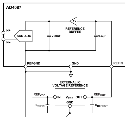
Figure 46. AD4087 General External Reference Design Functional Diagram
