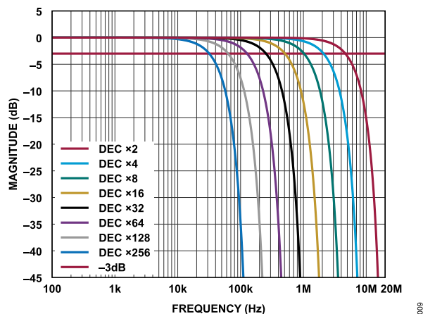
Figure 9. Sinc1 Filter Response, f_s = 20\text{MHz} (DEC \times Means Decimate By)
